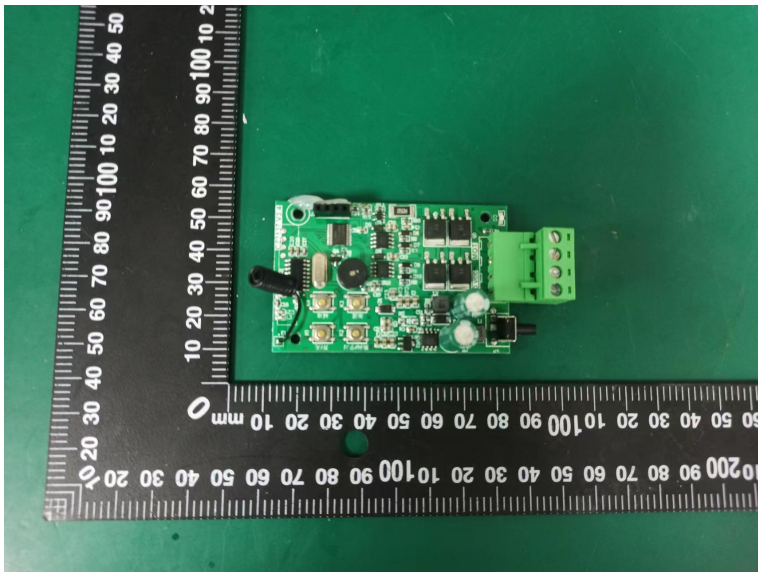
315 receiver Antenna
