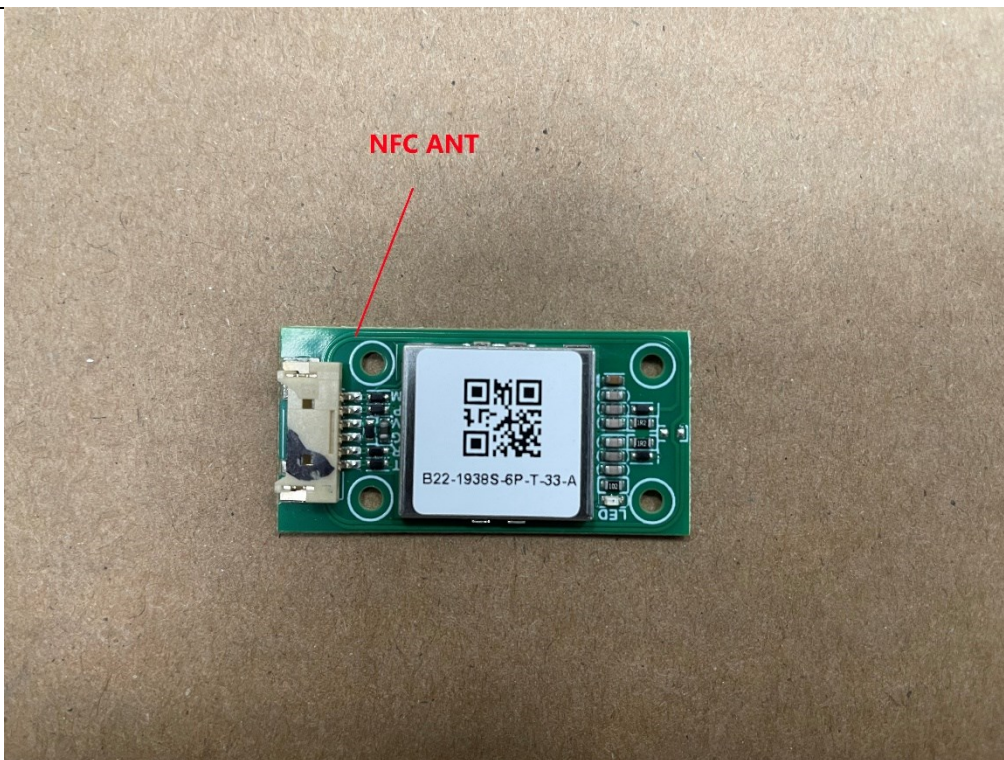
EUT Photo(2) - NFC Antenna
