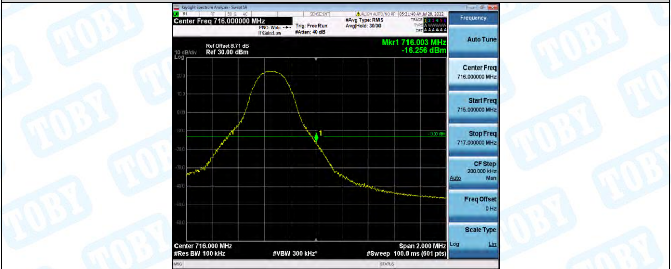
Band17-5MHz-QPSK-23825-25RB#0
