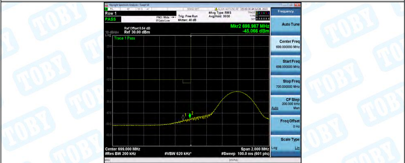
Band12-10MHz-16QAM-23060-50RB#0
