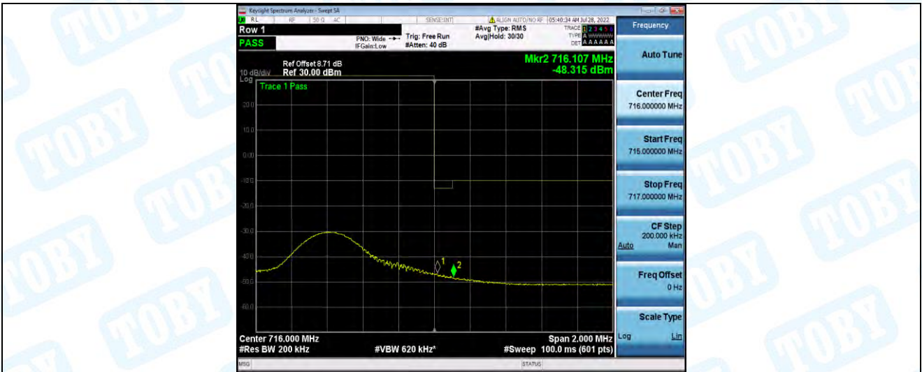
Band17-10MHz-QPSK-23800-1RB#49
