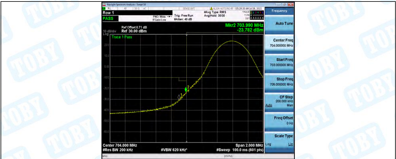
Band17-10MHz-16QAM-23780-1RB#49
