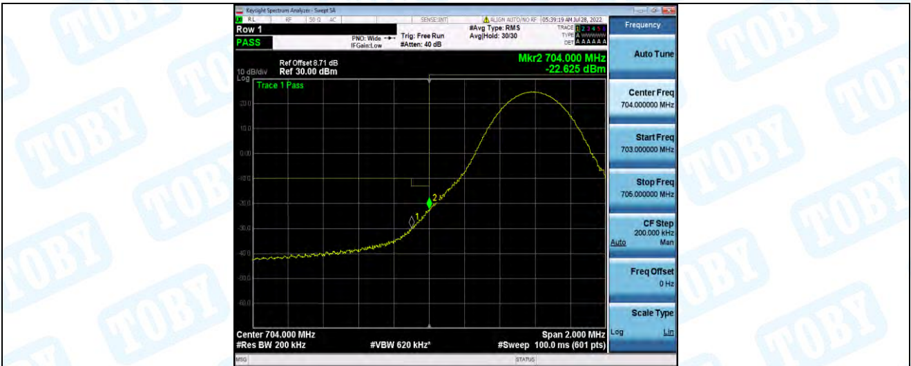
Band17-10MHz-QPSK-23780-1RB#49
