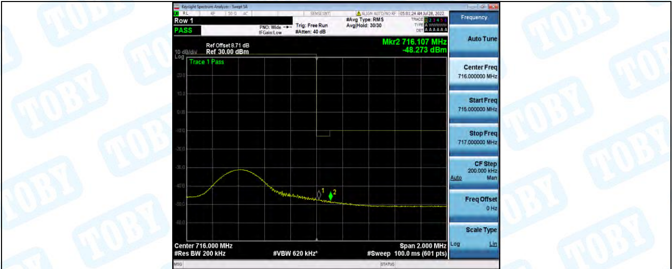
Band12-10MHz-16QAM-23130-1RB#49
