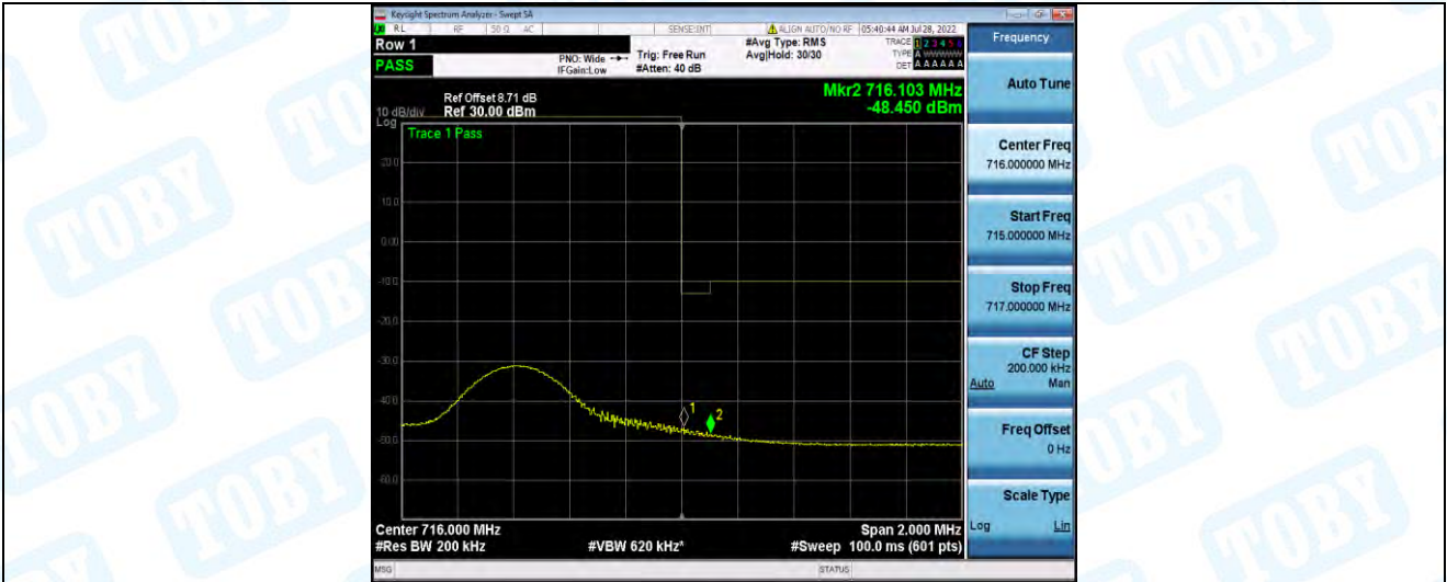
Band17-10MHz-16QAM-23800-1RB#49
