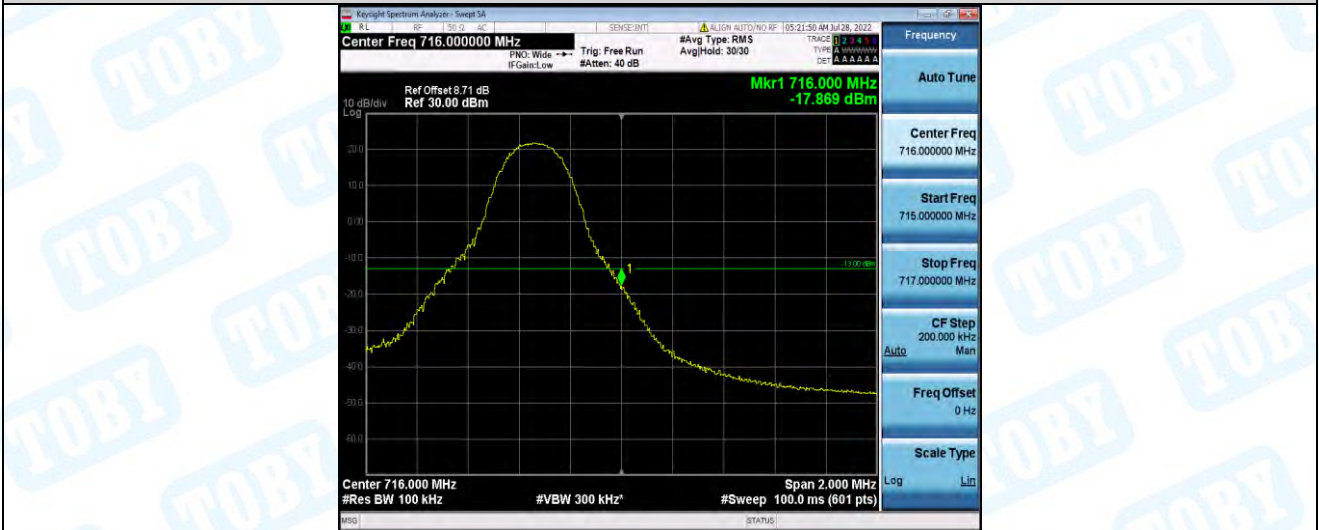
Band17-5MHz-16QAM-23825-25RB#0
