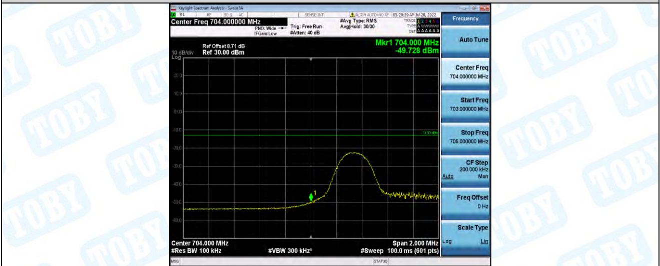
Band17-5MHz-16QAM-23755-25RB#0
