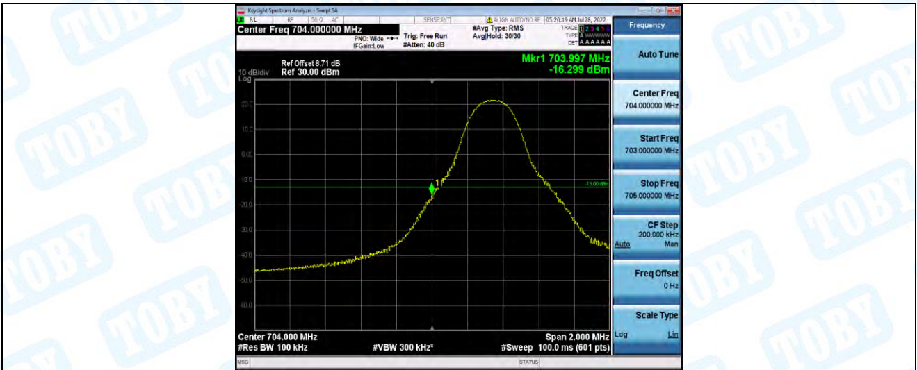
Band17-5MHz-16QAM-23755-1RB#24
