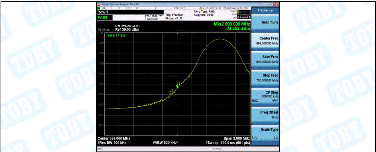
Band12-10MHz-16QAM-23060-1RB#49
