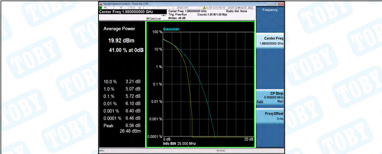
Band2-15MHz-16QAM-19125-1RB#0
