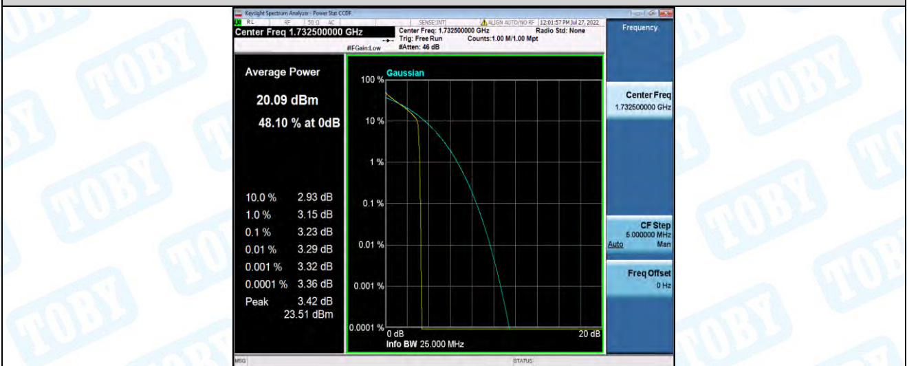
Band4-10MHz-QPSK-20175-50RB#0
