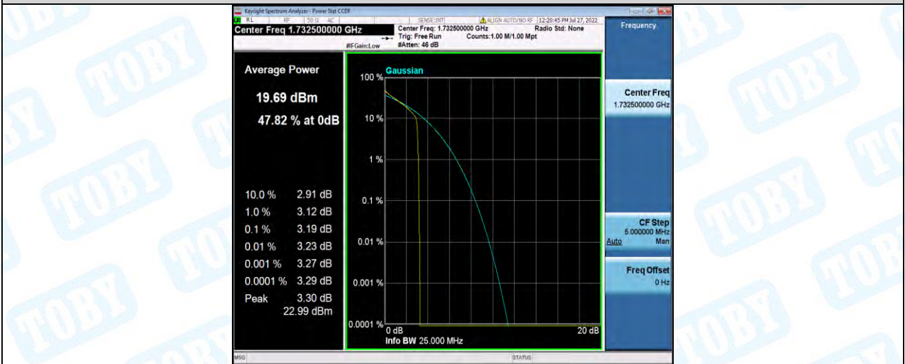
Band4-15MHz-QPSK-20175-75RB#0
