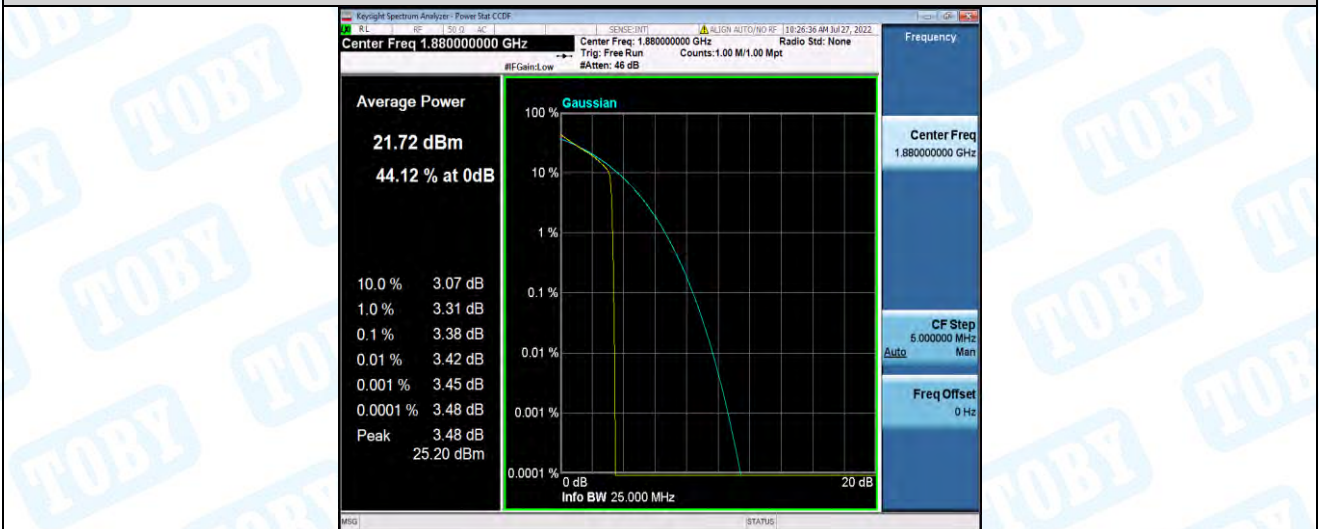
Band2-15MHz-QPSK-18900-75RB#0
