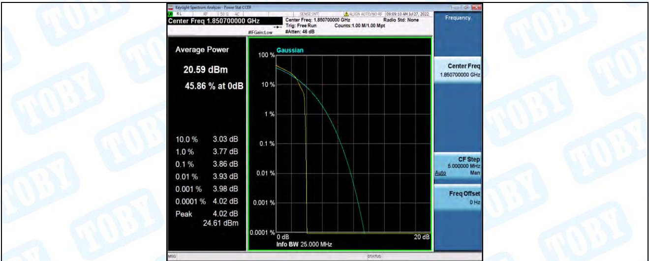
Band2-1.4MHz-16QAM-18607-6RB#0
