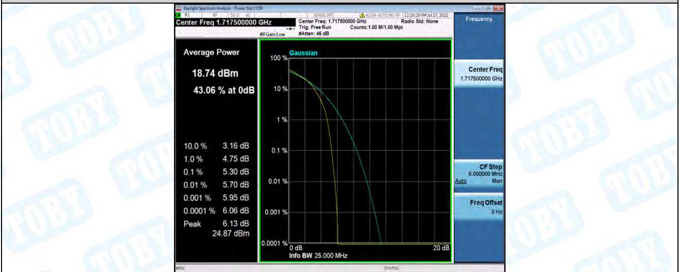
Band4-15MHz-16QAM-20175-1RB#0
