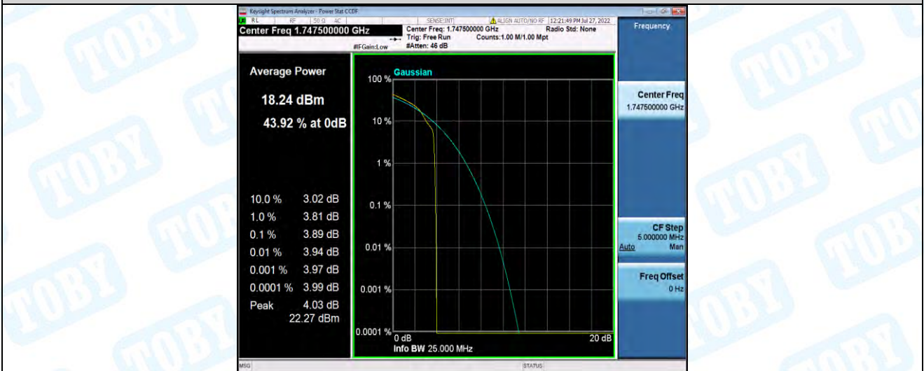
Band4-15MHz-16QAM-20325-75RB#0
