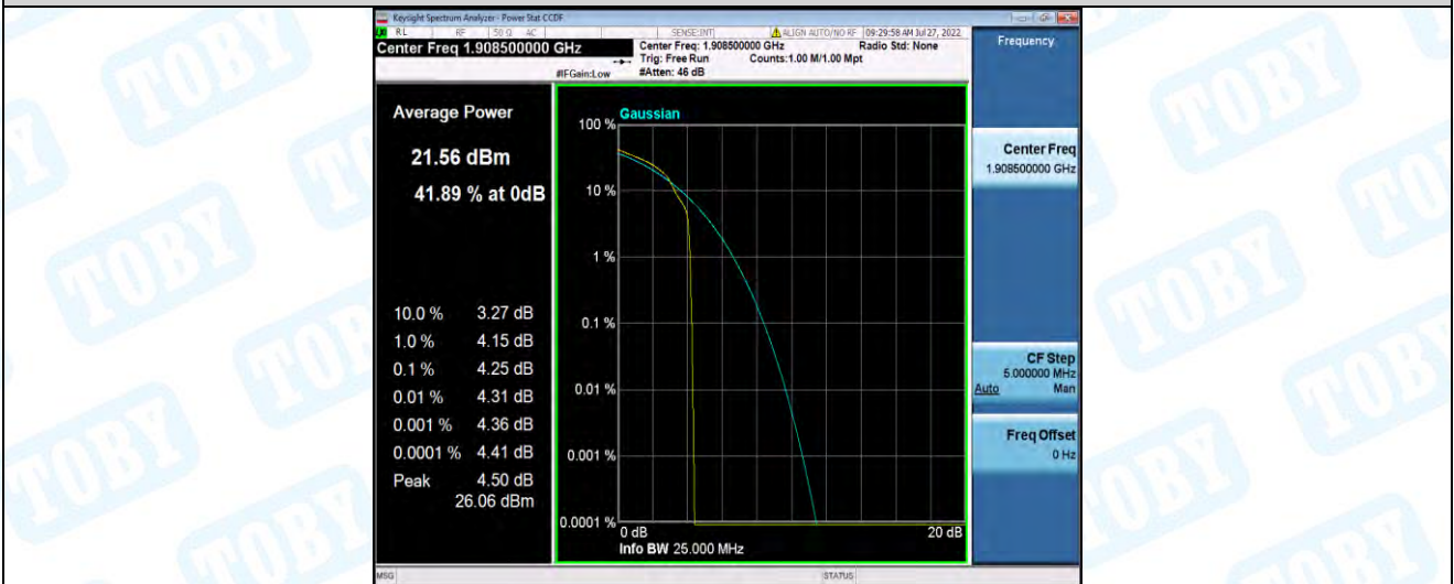
Band2-3MHz-16QAM-19185-15RB#0
