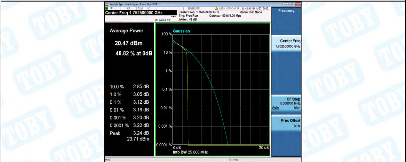
Band4-5MHz-QPSK-20375-25RB#0
