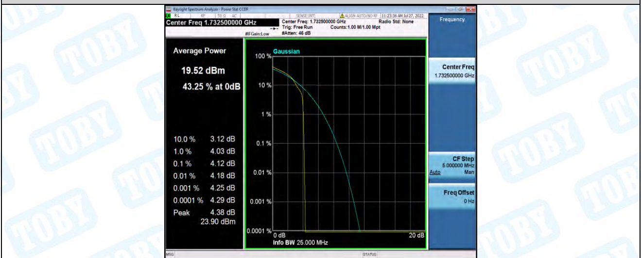
Band4-3MHz-16QAM-20175-15RB#0
