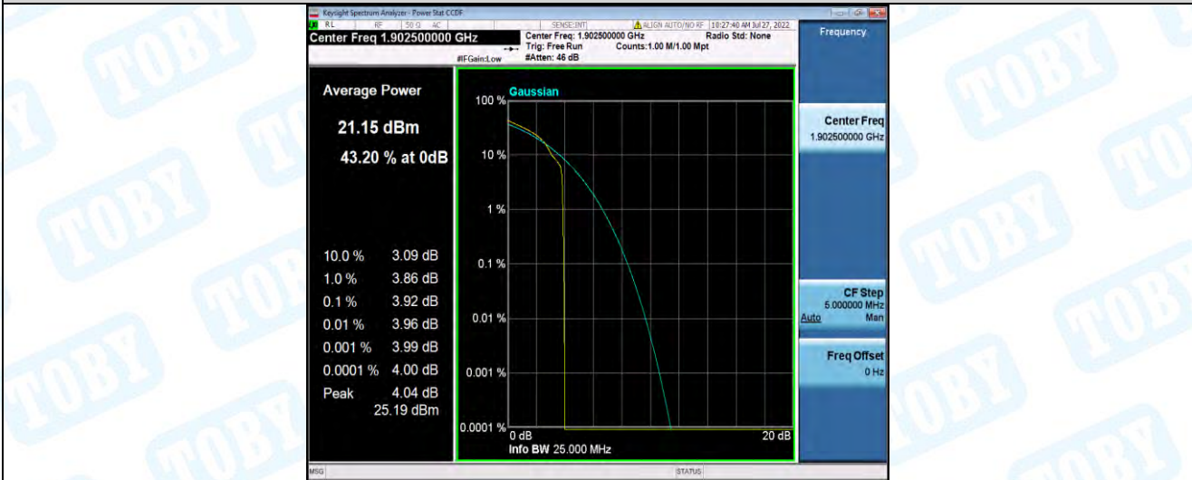
Band2-15MHz-16QAM-19125-75RB#0
