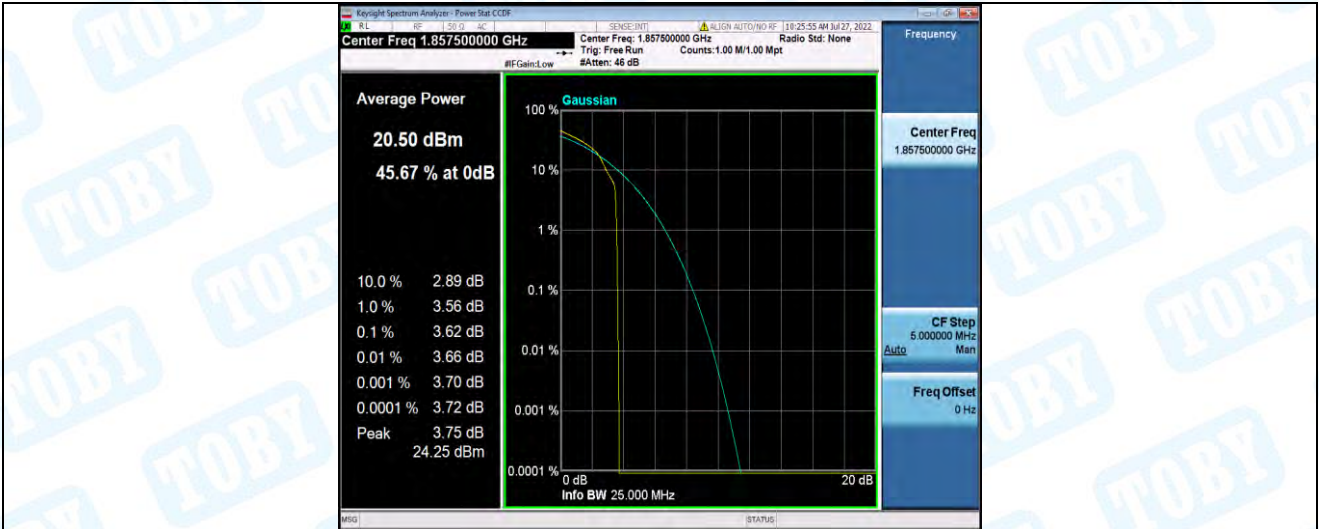
Band2-15MHz-16QAM-18675-75RB#0
