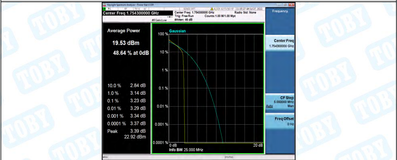
Band4-1.4MHz-QPSK-20393-6RB#0
