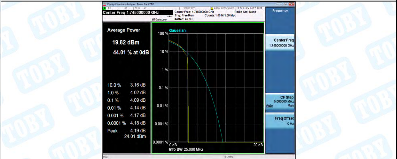
Band4-20MHz-16QAM-20300-100RB#0
