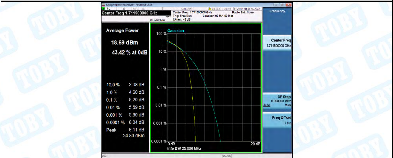
Band4-3MHz-16QAM-20175-1RB#0
