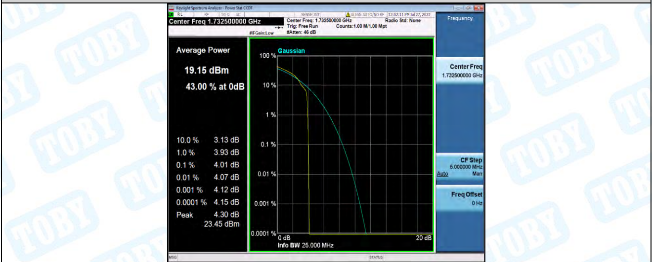
Band4-10MHz-16QAM-20175-50RB#0
