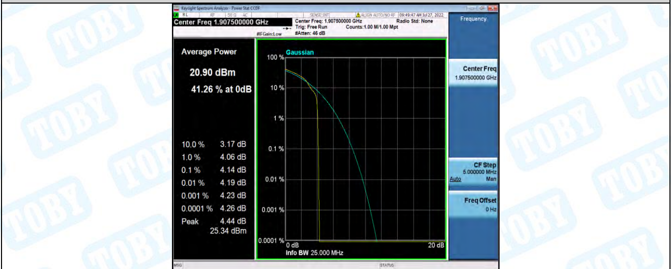
Band2-5MHz-16QAM-19175-25RB#0
