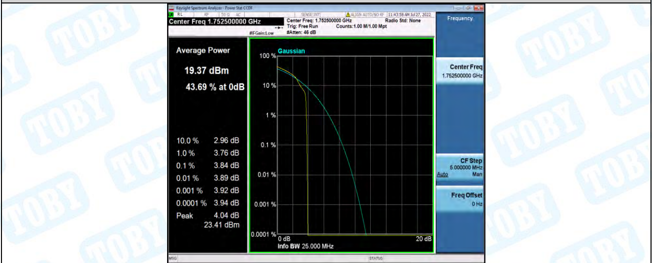
Band4-5MHz-16QAM-20375-25RB#0
