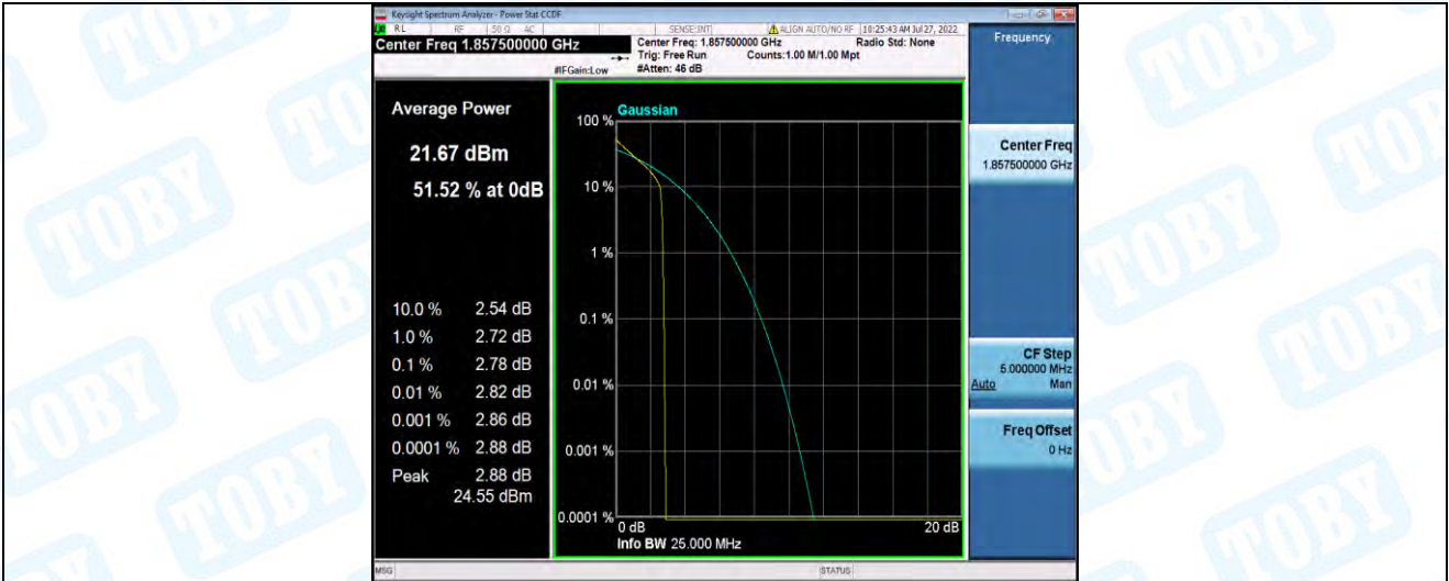
Band2-15MHz-QPSK-18675-75RB#0
