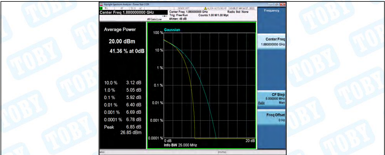
Band2-10MHz-16QAM-19150-1RB#0
