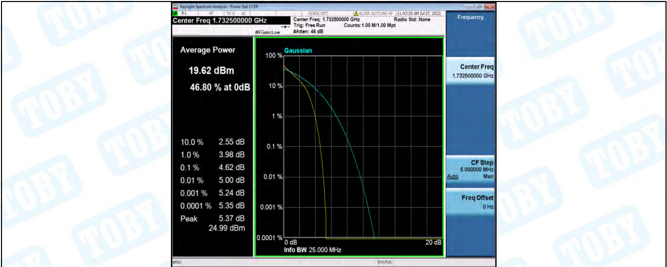
Band4-5MHz-QPSK-20375-1RB#0
