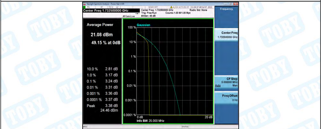
Band4-1.4MHz-QPSK-20175-6RB#0
