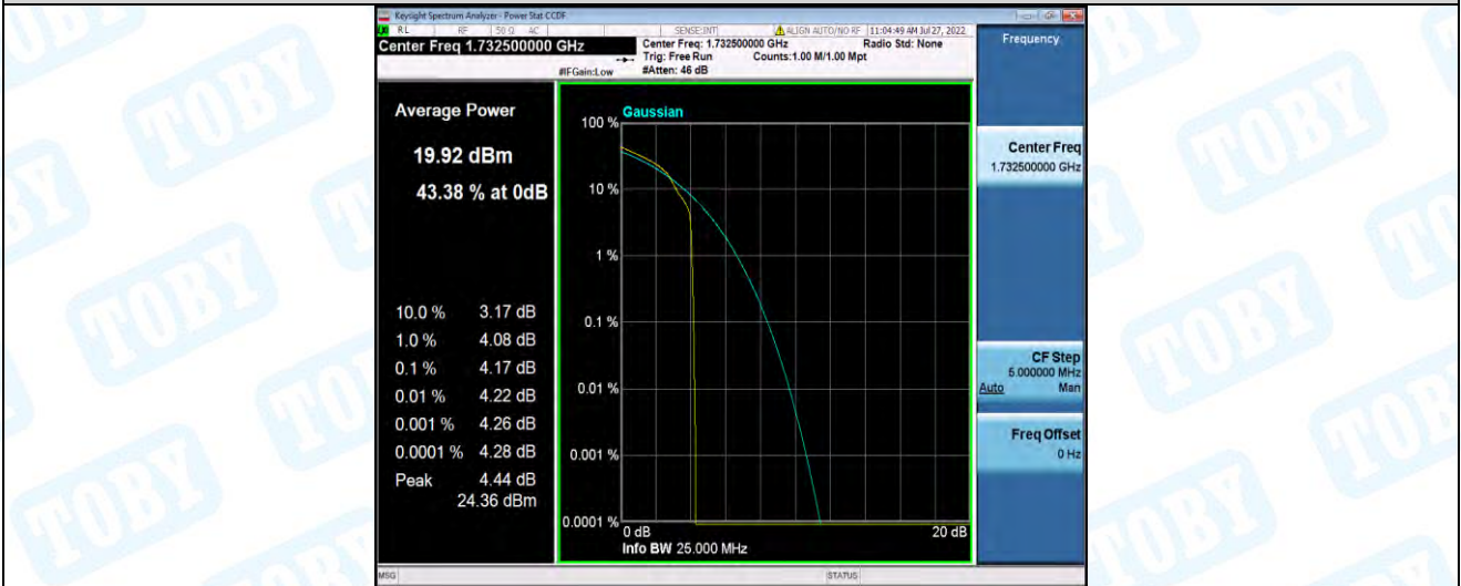
Band4-1.4MHz-16QAM-20175-6RB#0
