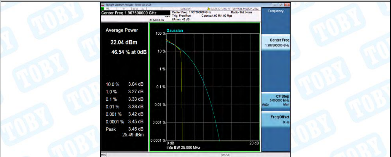
Band2-5MHz-QPSK-19175-25RB#0
