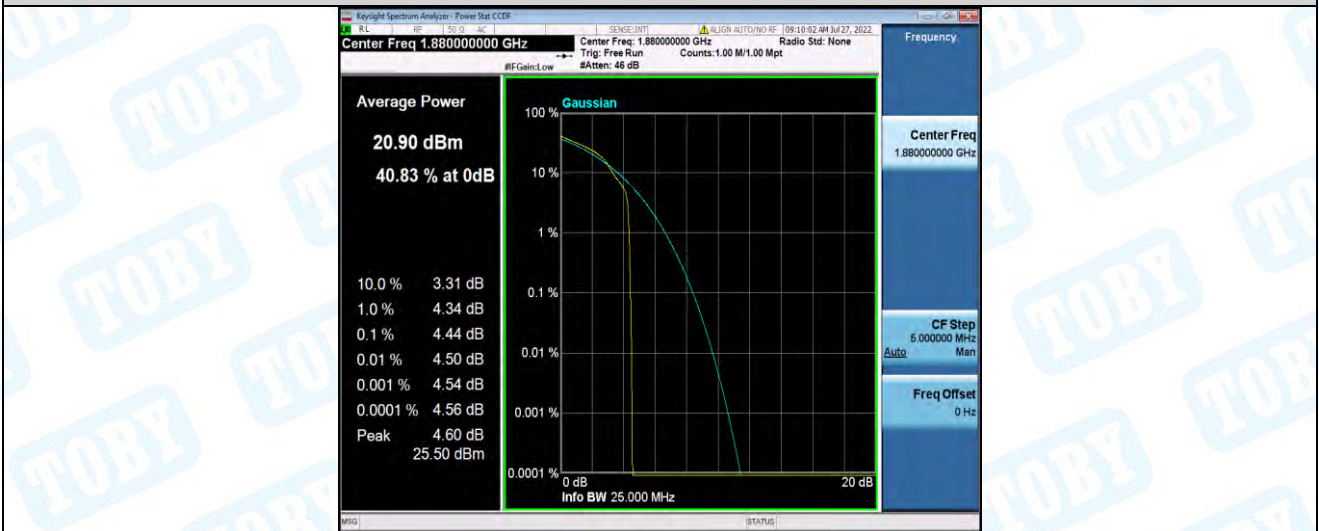
Band2-1.4MHz-16QAM-18900-6RB#0
