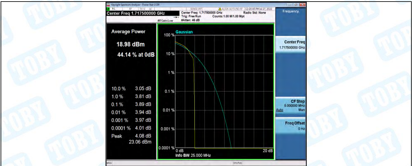
Band4-15MHz-16QAM-20025-75RB#0
