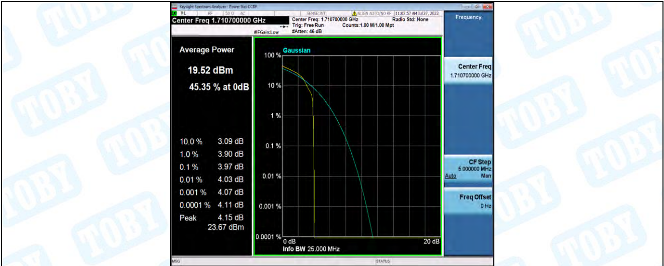
Band4-1.4MHz-16QAM-19957-6RB#0
