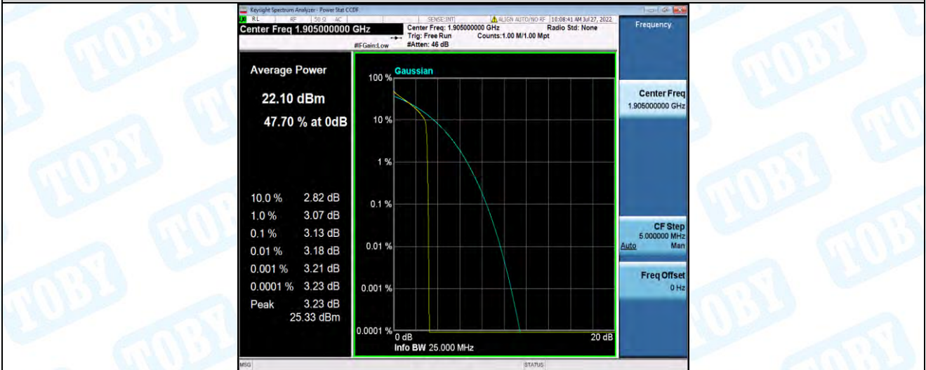
Band2-10MHz-QPSK-19150-50RB#0
