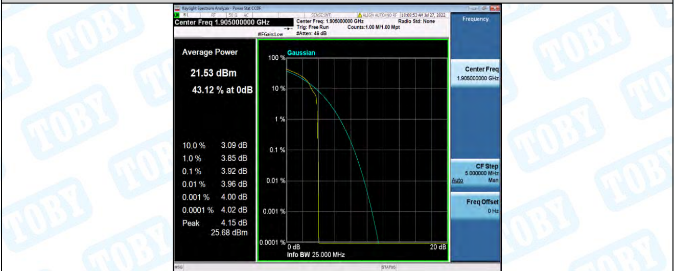
Band2-10MHz-16QAM-19150-50RB#0
