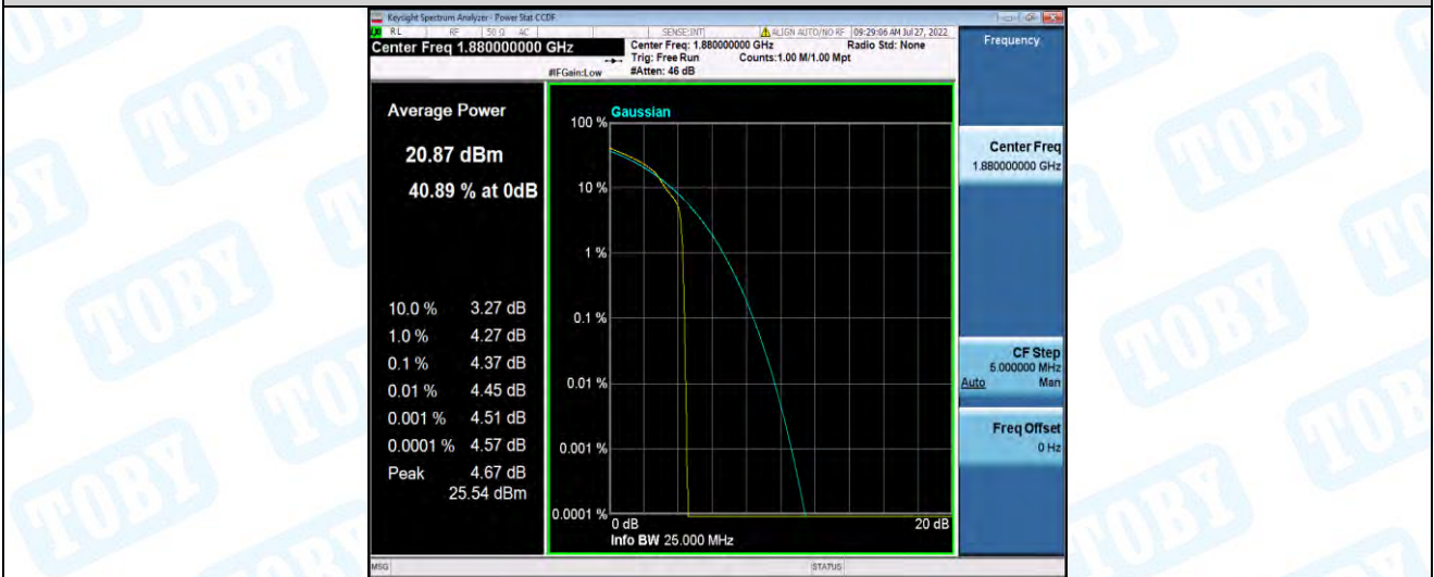
Band2-3MHz-16QAM-18900-15RB#0
