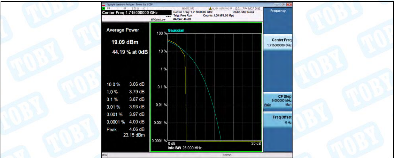
Band4-10MHz-16QAM-20000-50RB#0
