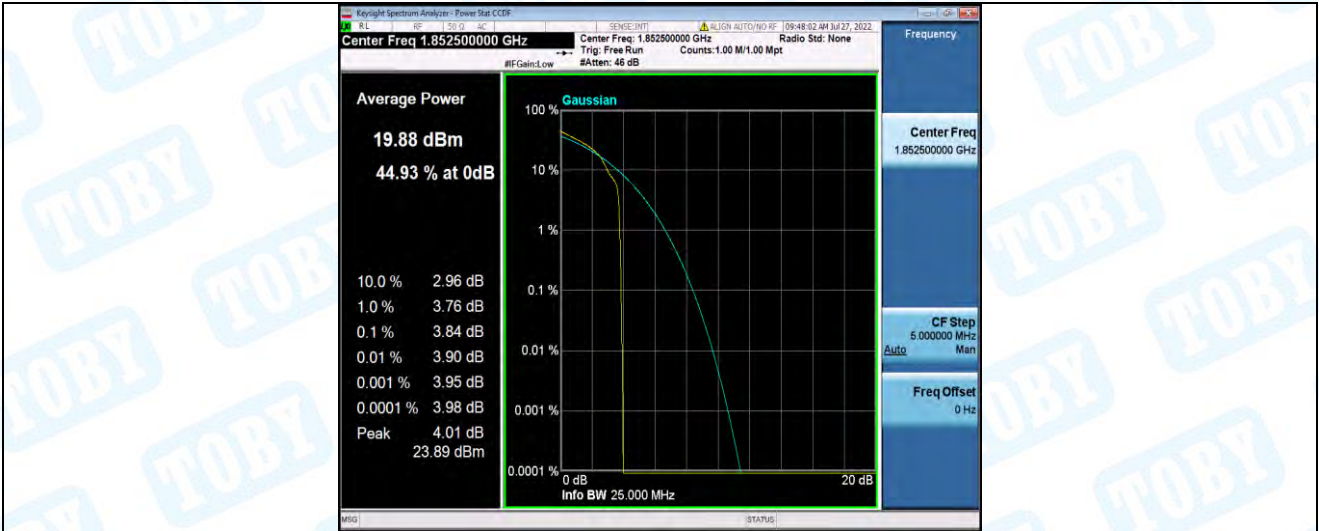
Band2-5MHz-16QAM-18625-25RB#0
