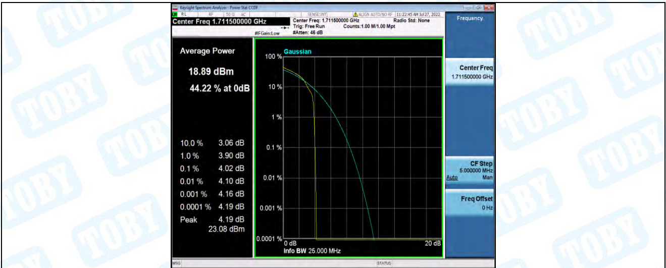
Band4-3MHz-16QAM-19965-15RB#0
