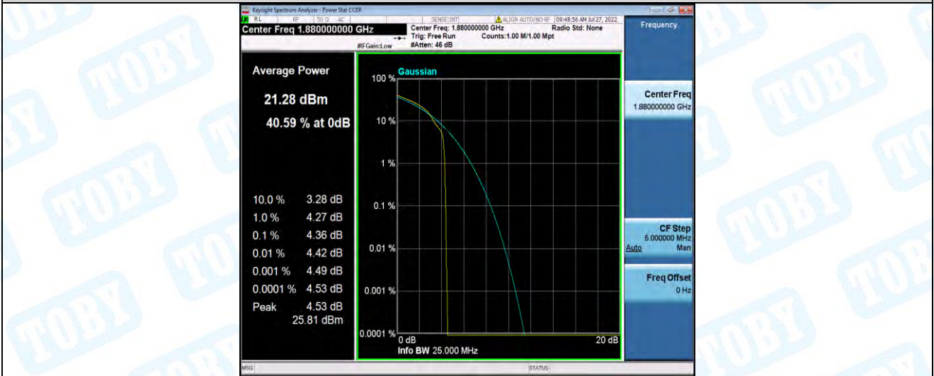
Band2-5MHz-16QAM-18900-25RB#0
