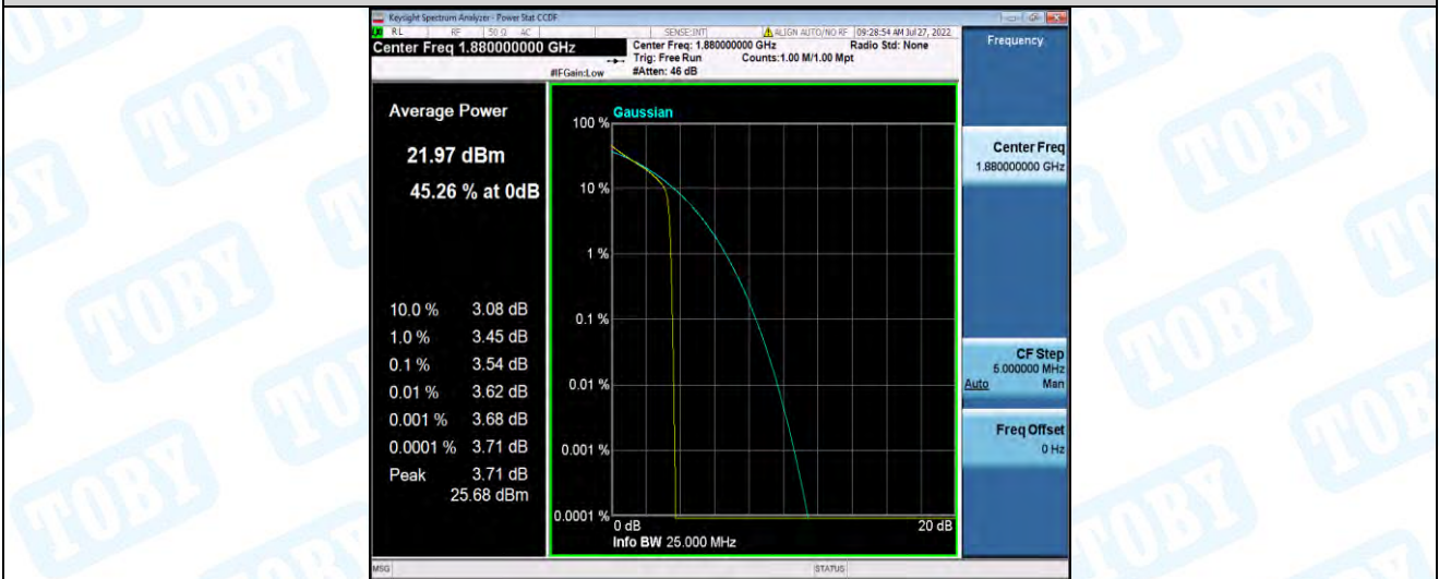
Band2-3MHz-QPSK-18900-15RB#0
