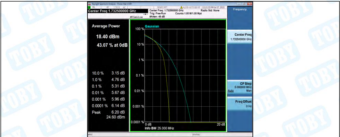
Band4-15MHz-16QAM-20325-1RB#0
