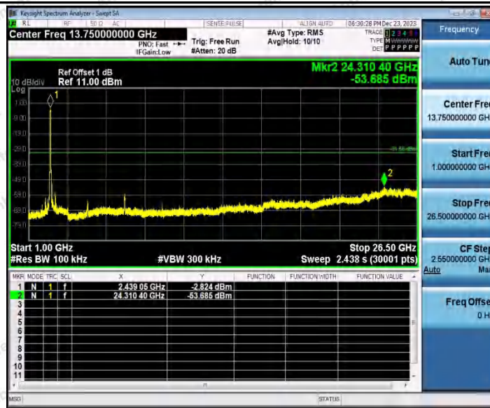
11N40SISO_Ant1_2452_0~Reference
