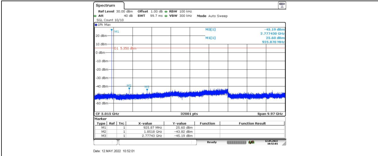
2GFSK-25 kbps_Ant1_HCH_Spurious
