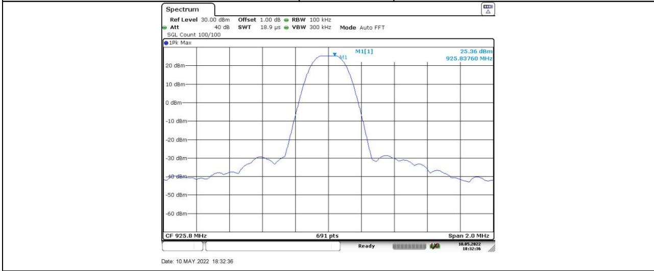
2GFSK-75 kbps_Ant1_HCH_Reference
