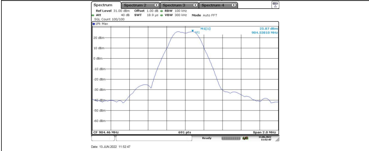
2GFSK-150 kbps_Ant1_LCH_Reference
