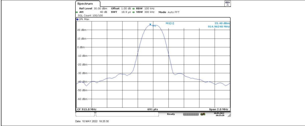
2GFSK-75 kbps_Ant1_MCH_Reference
