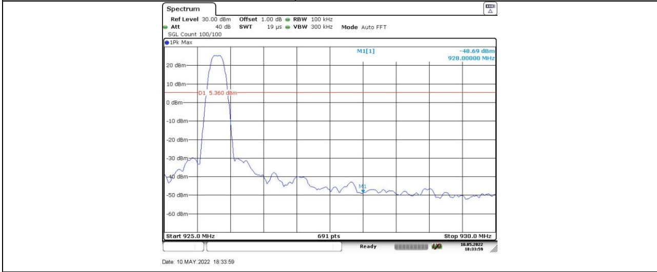
2GFSK-75 kbps_Ant1_HCH_Bandedge
