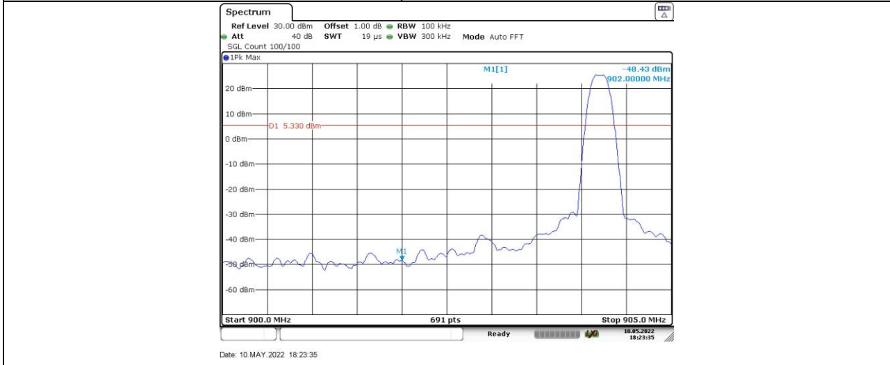
2GFSK-75 kbps_Ant1_LCH_Bandedge
