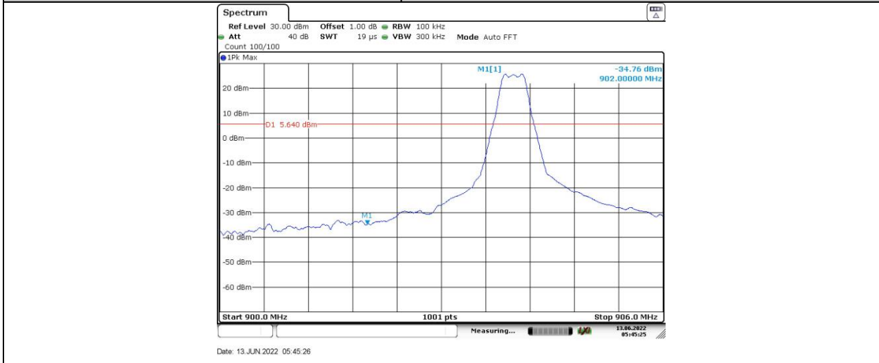
2GFSK-250 kbps_Ant1_LCH_Bandedge
