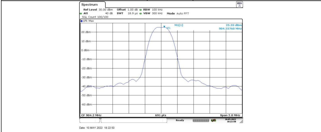
2GFSK-75 kbps_Ant1_LCH_Reference
