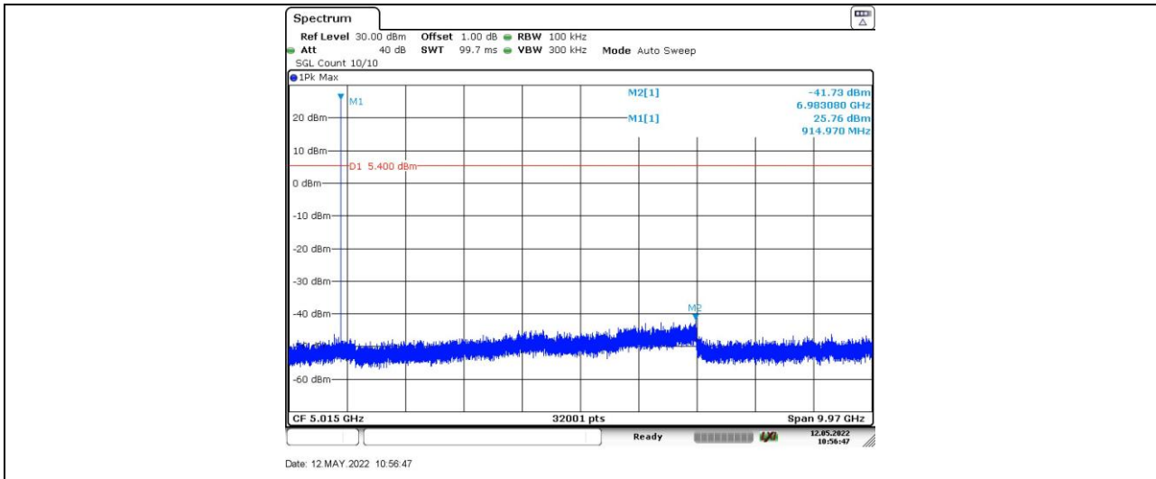
2GFSK-75 kbps_Ant1_MCH_Spurious
