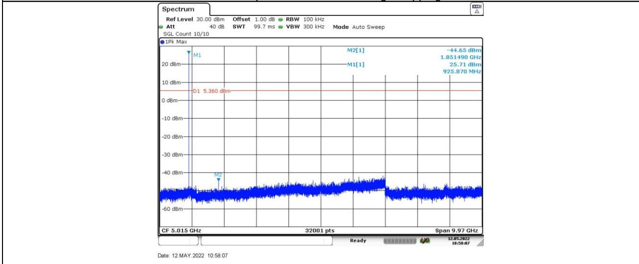
2GFSK-75 kbps_Ant1_HCH_Spurious
