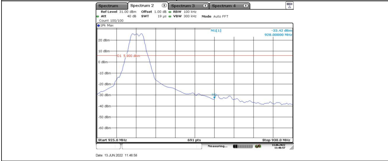
2GFSK-250 kbps_Ant1_HCH_Bandedge
