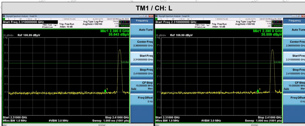
Peak Value(Vertical)
