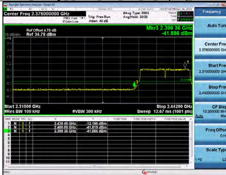
2_Bandedge 2_4GWiFi_NVNT_ANT1_802_11n(HT40)_2422
