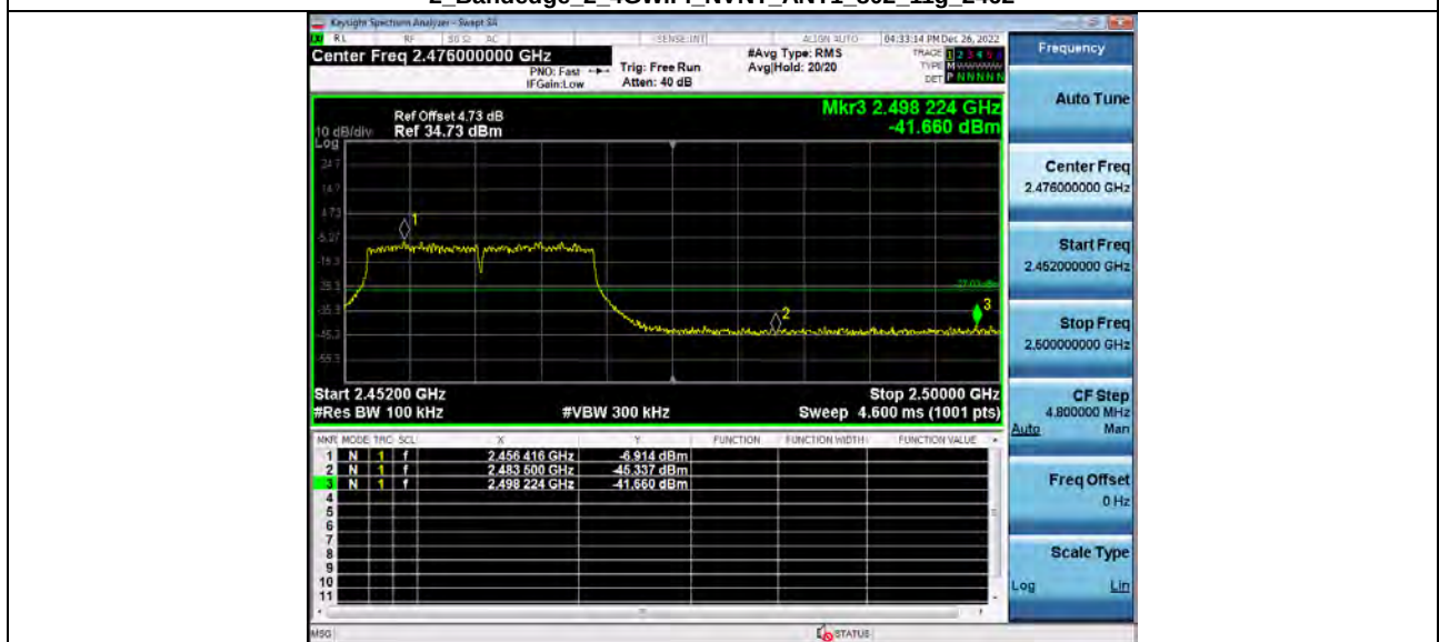
2 Bandedge 2 4GWiFi NVNT ANT1 802_11g 2462
