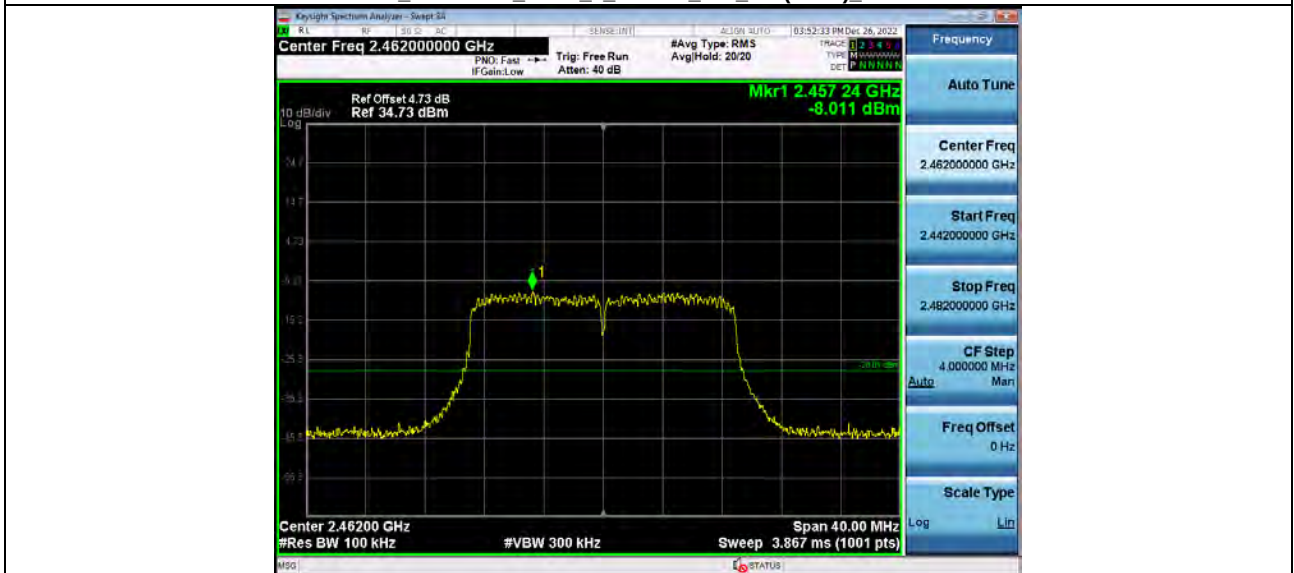
2 Bandedge 2 4GWiFi NVNT ANT1 802_11n(HT20) 2462
