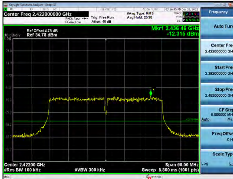
2_Bandedge 2_4GWiFi_NVNT_ANT1_802_11n(HT40)_2422
