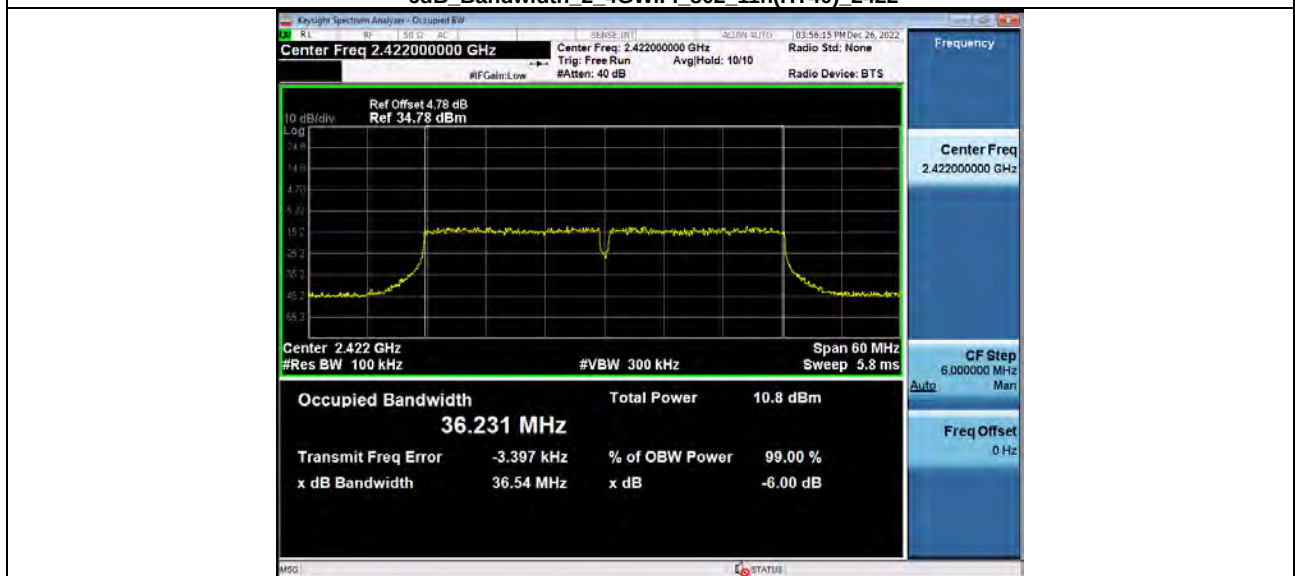
-6dB_Bandwidth 2_4GWiFi 802_11n(HT40) 2422
