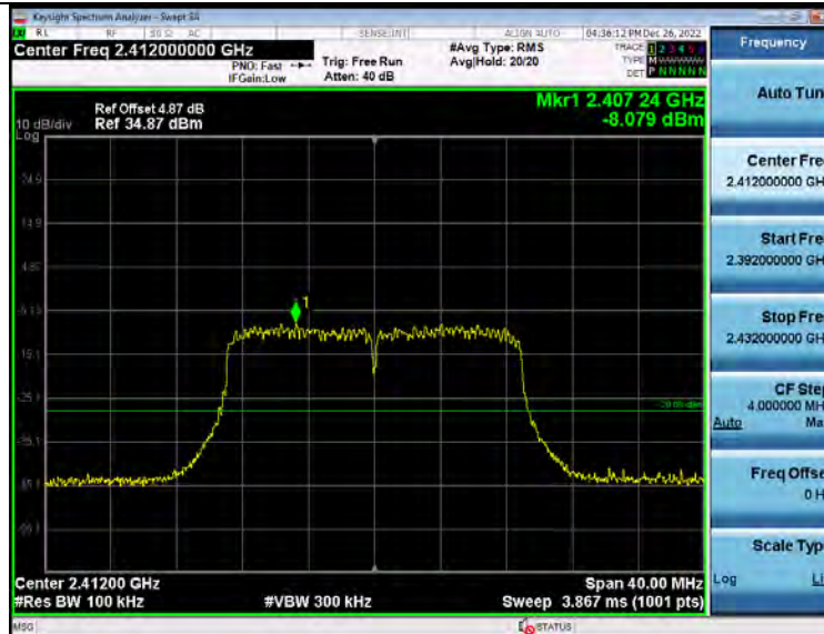
2_Bandedge 2_4GWiFi_NVNT_ANT1_802_11n(HT20)_2412
