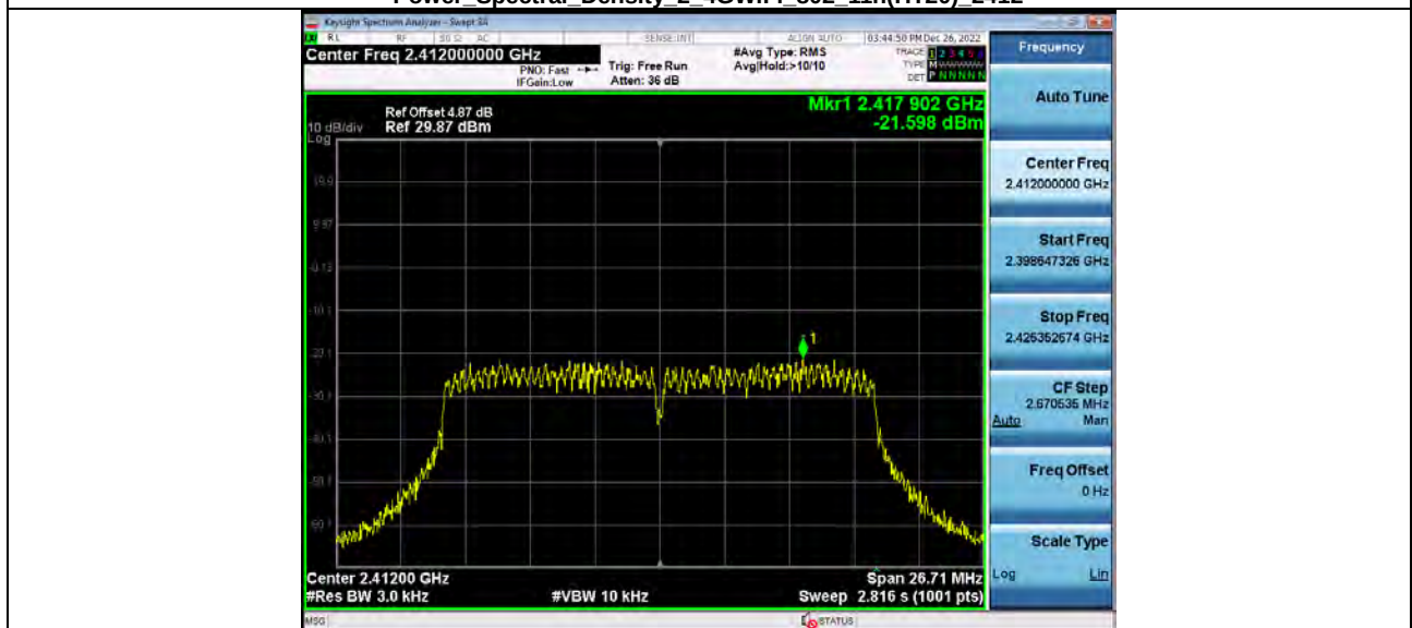
Power_Spectral_Density_2_4GWiFi_802_11n(HT20)_2412
