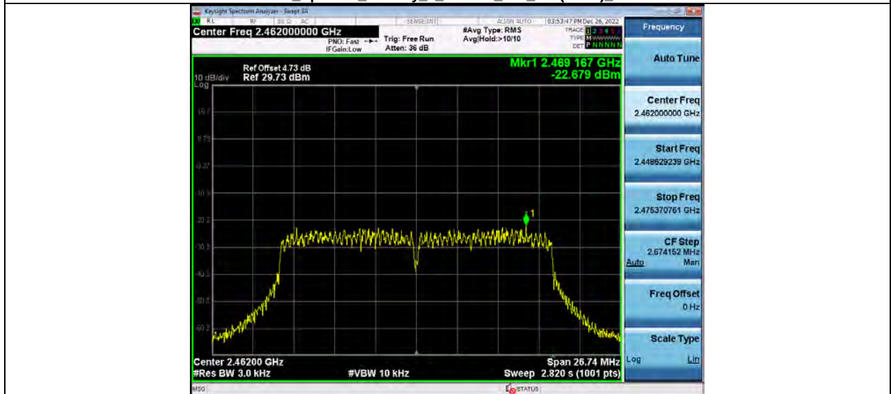
Power Spectral Density 2_4GWiFi_802_11n(HT20)_2462
