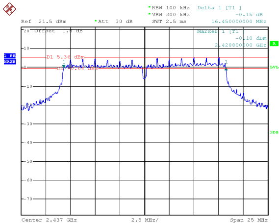
TX 11g channel 6
