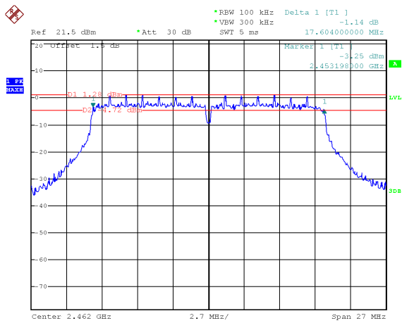
TX 11n HT20 channel 11
