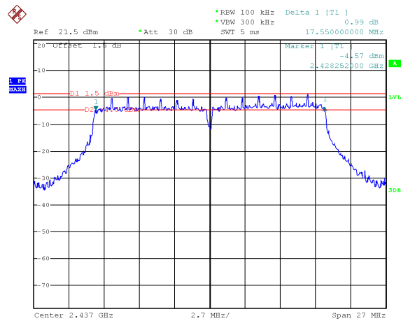
TX 11n HT20 channel 6
