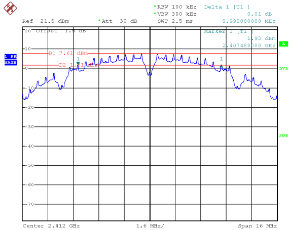
TX 11b channel 1
