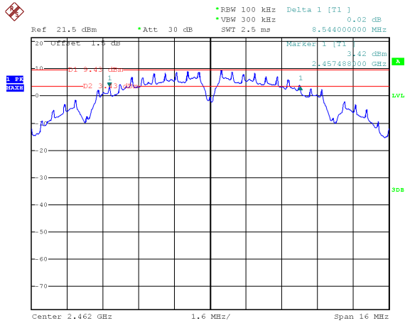
TX 11b channel 11
