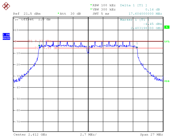
TX 11n HT20 channel 1
