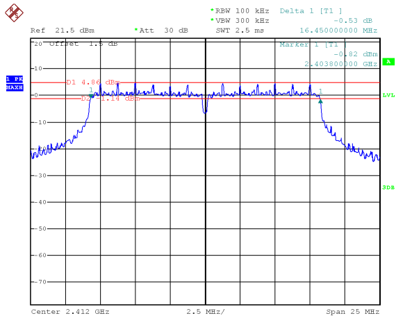
TX 11g channel 1
