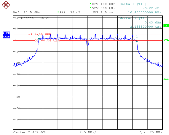
TX 11g channel 11
