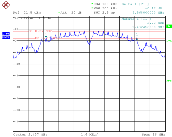
TX 11b channel 6
