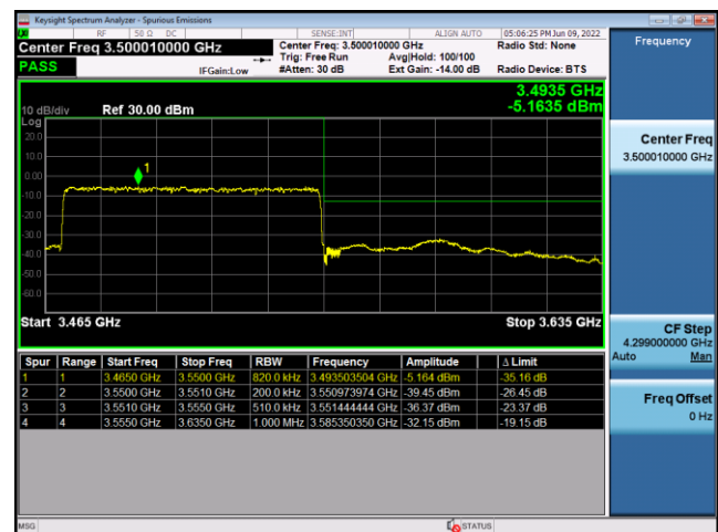
N78(80M)_CP-OFDM_QPSK_Edge_ Outer_Full_High_CH
