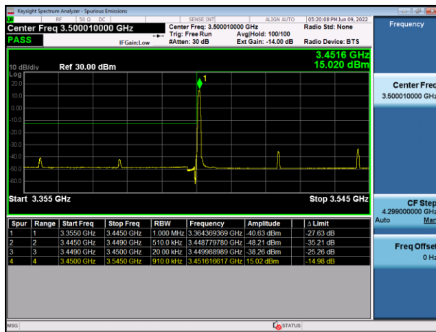
N78(90M)_CP-OFDM_QPSK_Edge_ 1RB_Left_Low_CH
