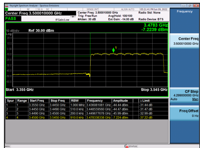
N78(90M)_DFT-s-OFDM_PI/2-BPSK_Edge_ Outer_Full_High_CH
