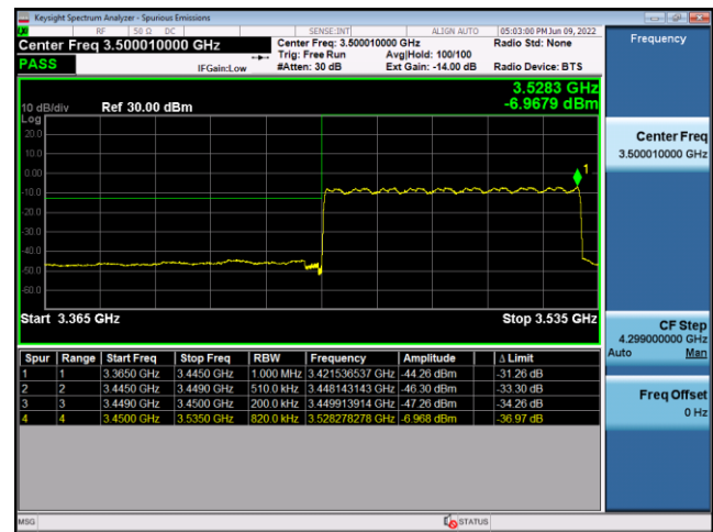
N78(80M)_DFT-s-OFDM_PI/2-BPSK_Edge_ Outer_Full_High_CH
