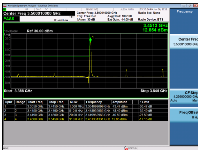
N78(90M)_DFT-s-OFDM_PI/2-BPSK_Edge_ 1RB_Right_High_CH
