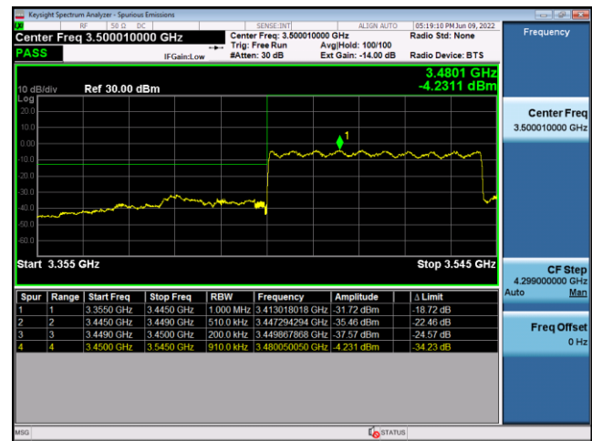
N78(90M)_CP-OFDM_QPSK_Edge_ Outer_Full_Low_CH
