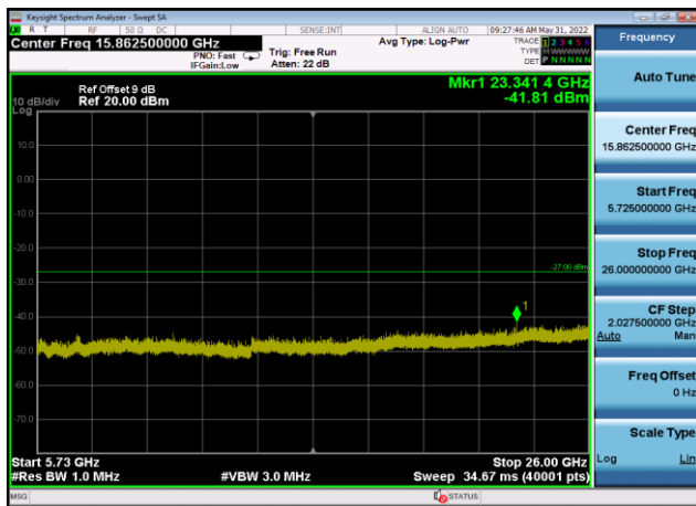
U-NII-2c ,Plot 3,5725MHz~26000MHz-802 .11a(20MHz),5500MHz,Ant9
