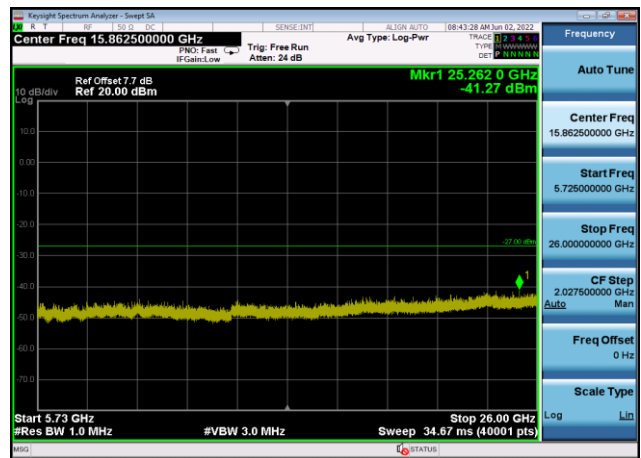
U-NII-2c ,Plot 3,5725MHz~26000MHz-802 .11a(20MHz),5500MHz,Ant8
