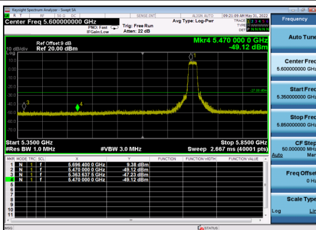
U-NII-2c ,Plot 1,Band Edge-802.11a(20 MHz),5700MHz,Ant9
