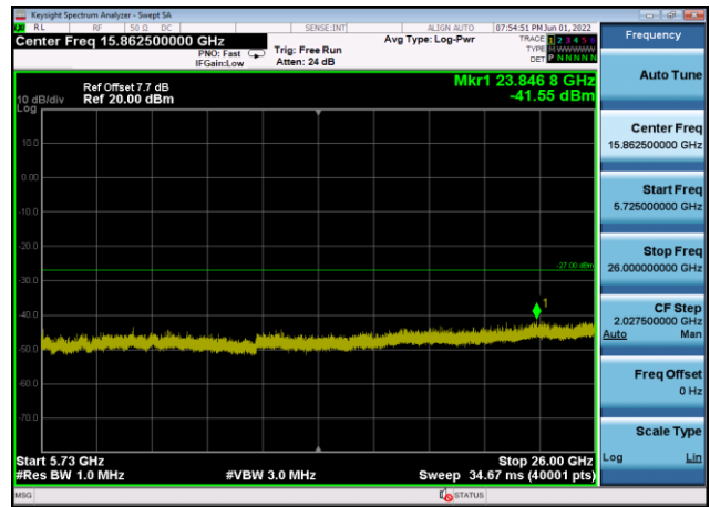
U-NII-2c ,Plot 3,5725MHz~26000MHz-802 .11n(40MHz),5590MHz,Ant8
