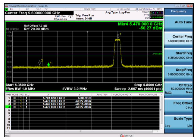
U-NII-2c ,Plot 1,Band Edge-802.11n(20 MHz),5700MHz,Ant8
