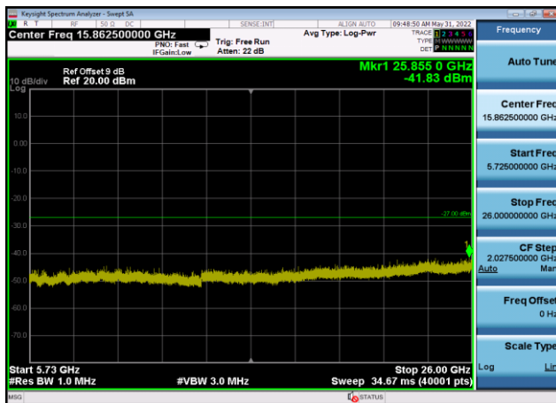
U-NII-2c ,Plot 3,5725MHz~26000MHz-802 .11n(20MHz),5600MHz,Ant9
