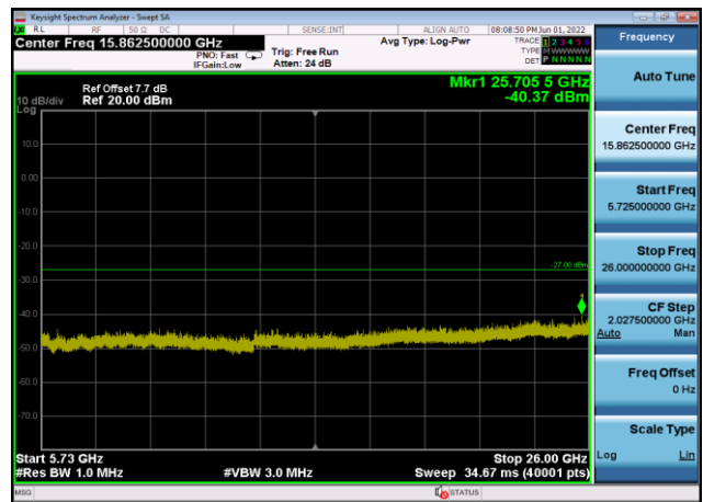
U-NII-2c ,Plot 3,5725MHz~26000MHz-802 .11n(40MHz),5670MHz,Ant8
