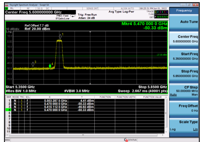
U-NII-2c ,Plot 1,Band Edge-802.11n(20 MHz),5600MHz,Ant8
