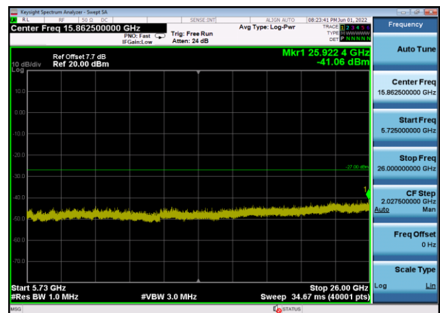
U-NII-2c ,Plot 3,5725MHz~26000MHz-802 .11n(20MHz),5700MHz,Ant8
