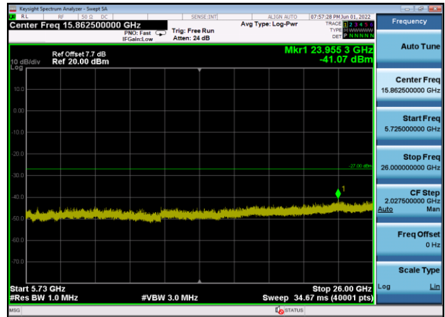
U-NII-2c ,Plot 3,5725MHz~26000MHz-802 .11n(40MHz),5670MHz,Ant8
