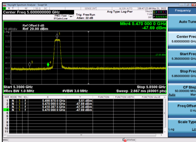
U-NII-2c ,Plot 1,Band Edge-802.11n(20 MHz),5600MHz,Ant9
