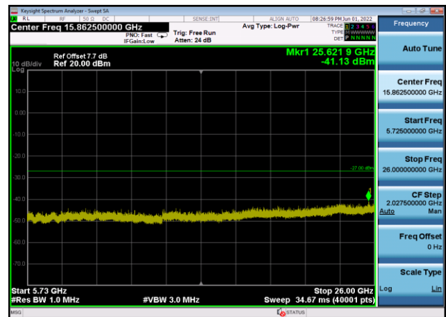
U-NII-2c ,Plot 3,5725MHz~26000MHz-802 .11n(20MHz),5600MHz,Ant8
