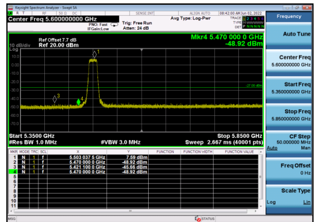
U-NII-2c ,Plot 1,Band Edge-802.11a(20 MHz),5600MHz,Ant8
