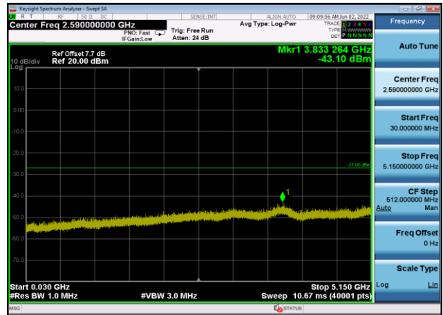
U-NII-1 ,Plot 2,30MHz~5150MHz-802.11n (20MHz),5240MHz,Ant8
