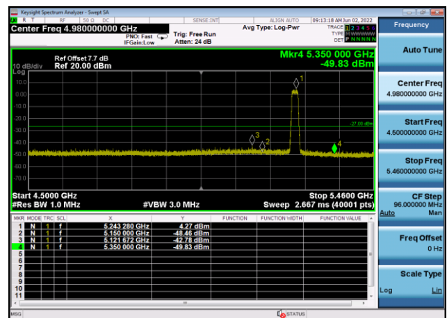
U-NII-1 ,Plot 1,Band Edge-802.11n(20M Hz),5240MHz,Ant8
