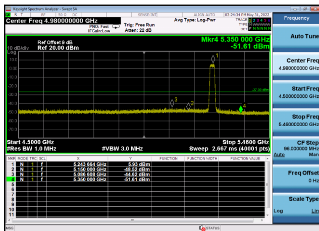
U-NII-1 ,Plot 1,Band Edge-802.11n(20M Hz),5240MHz,Ant9
