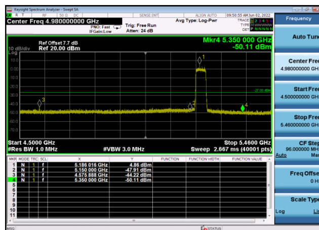
U-NII-1 ,Plot 1,Band Edge-802.11ax(40 MHz),5230MHz,Ant8
