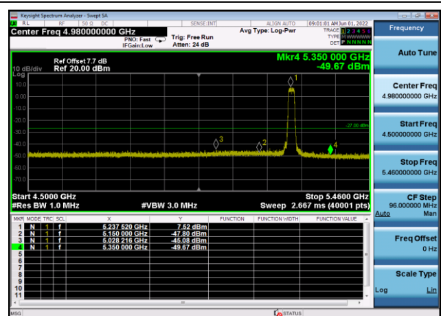
U-NII-1 ,Plot 1,Band Edge-802.11a(20M Hz),5240MHz,Ant8
