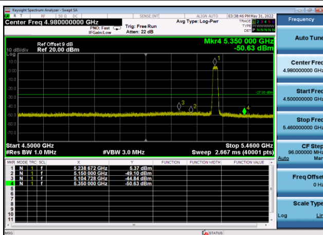
U-NII-1 ,Plot 1,Band Edge-802.11ac(20 MHz),5240MHz,Ant9
