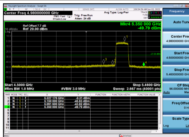
U-NII-1 ,Plot 1,Band Edge-802.11ax(80 MHz),5210MHz,Ant8
