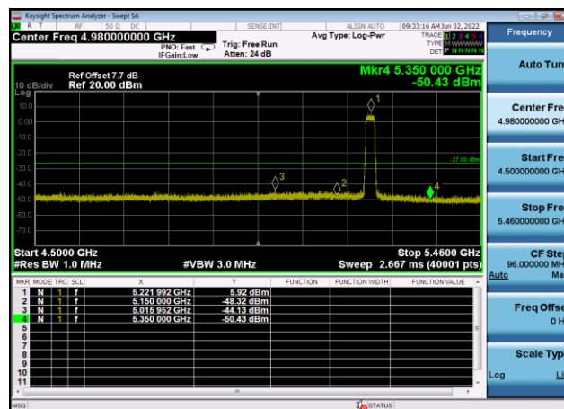
U-NII-1 ,Plot 1,Band Edge-802.11ax(20 MHz),5240MHz,Ant8
