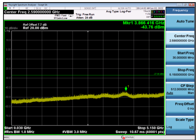
U-NII-1 ,Plot 2,30MHz~5150MHz-802.11n (20MHz),5240MHz,Ant8
