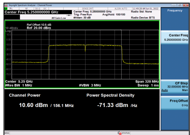
U-NII-2a Output Power-802.11ax(160MHz) ,5250MHz,Ant8
