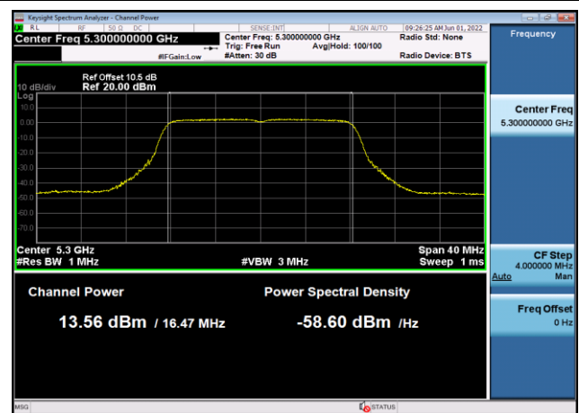
U-NII-2a Output Power-802.11a(20MHz) ,5300MHz,Ant8
