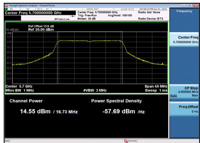
U-NII-2c Output Power-802.11a(20MHz) ,5700MHz,Ant8
