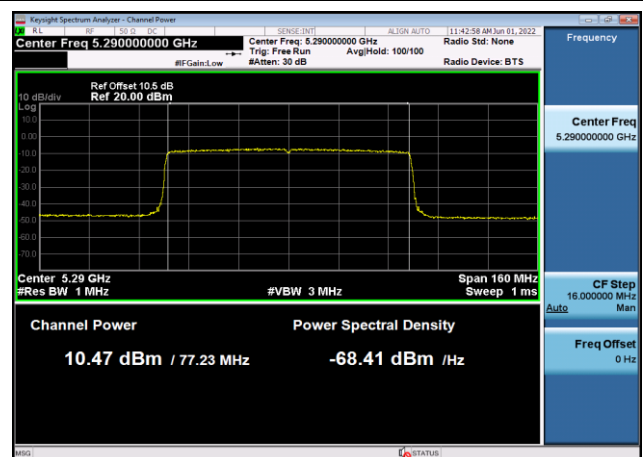
U-NII-2a Output Power-802.11ax(80MHz) ,5290MHz,Ant8
