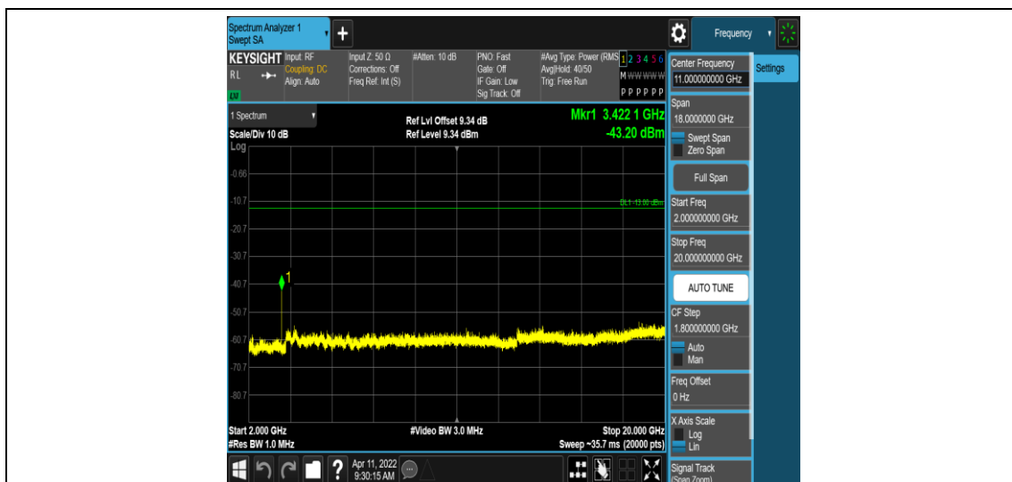
Band4-20MHz-16QAM-20050-1RB#0-Range5:2000~20000MHz
