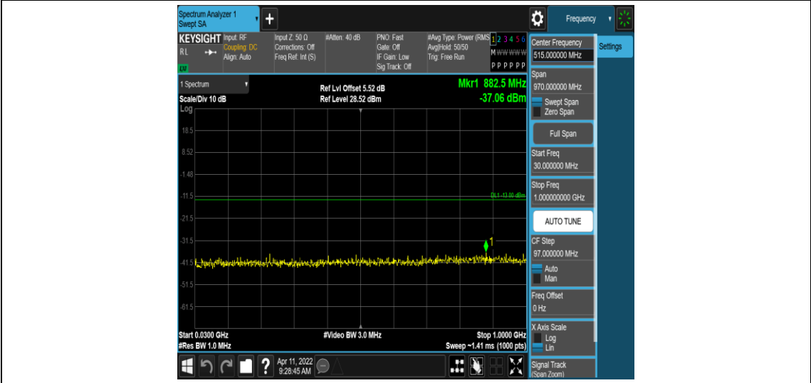
Band4-20MHz-QPSK-20050-1RB#0-Range3:30~1000MHz
