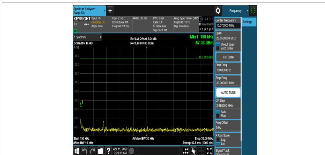
Band4-20MHz-16QAM-20050-1RB#0-Range2:0.15~30MHz
