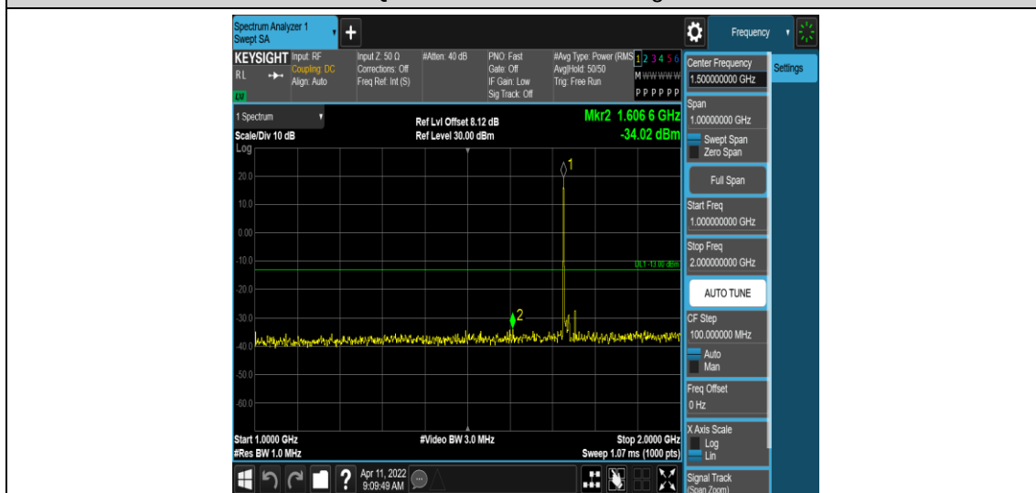
Band4-15MHz-QPSK-20175-1RB#0-Range4:1000~2000MHz
