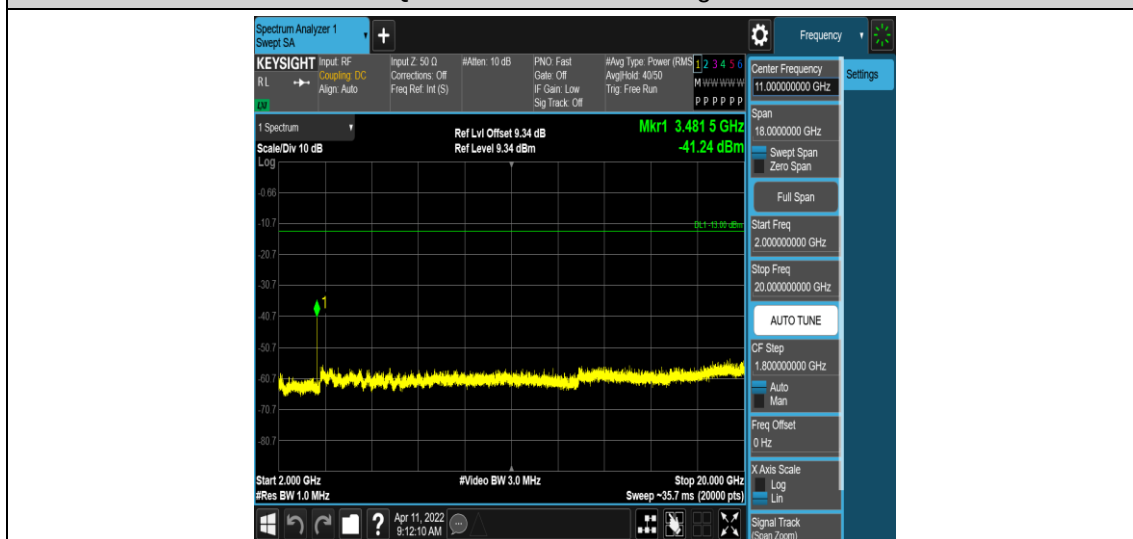
Band4-15MHz-QPSK-20325-1RB#0-Range5:2000~20000MHz
