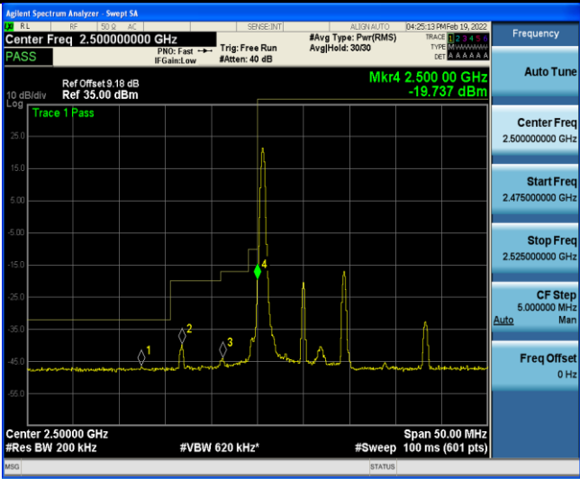
Band7-10MHz-16QAM-20800-1RB#49
