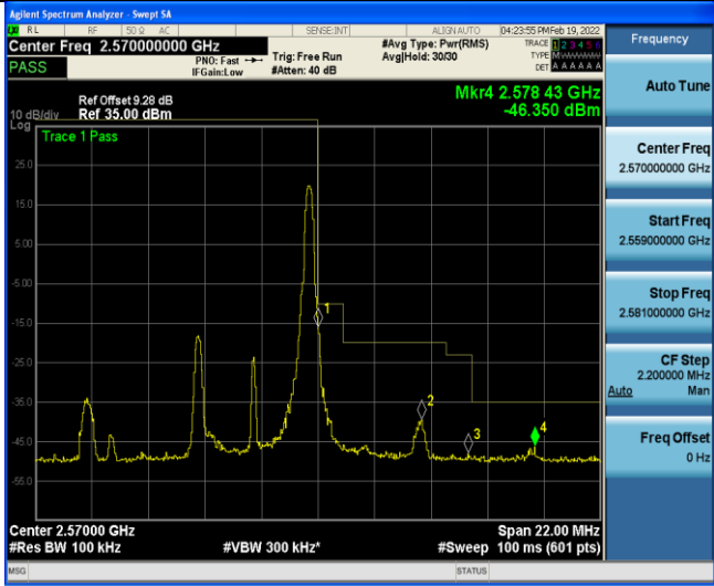
Band7-5MHz-16QAM-21425-25RB#0
