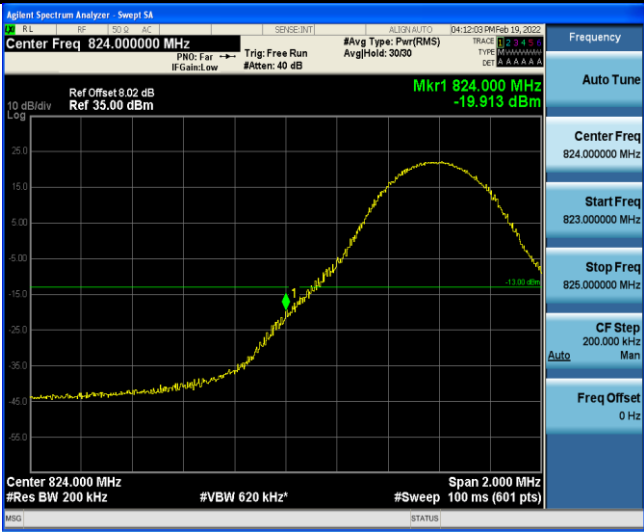
Band5-10MHz-16QAM-20450-1RB#49
