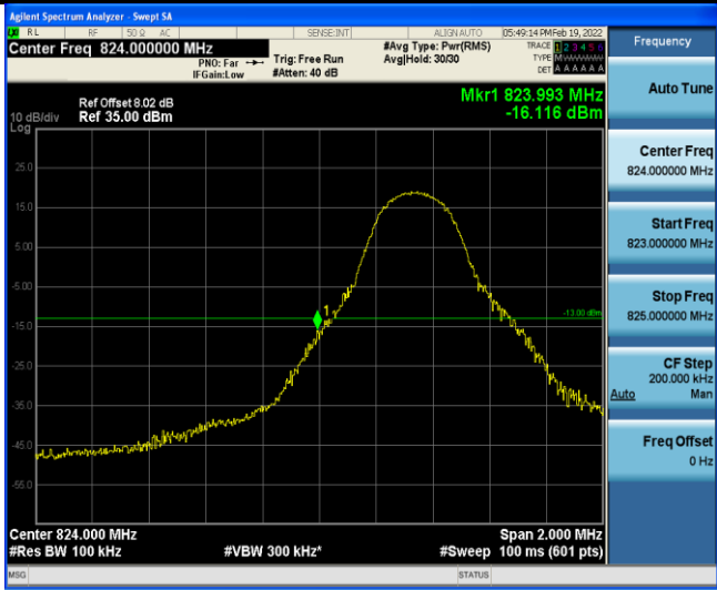
Band5-5MHz-QPSK-20425-1RB#24
