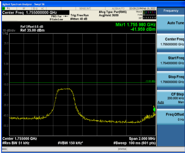
Band4-3MHz-16QAM-20385-1RB#14
