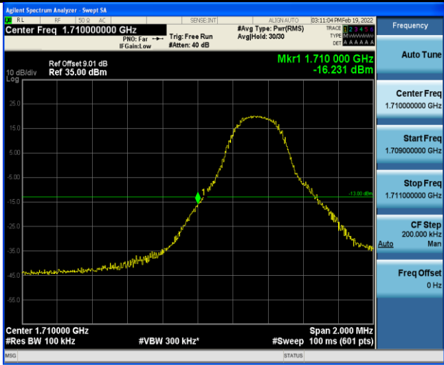
Band4-5MHz-16QAM-19975-1RB#24
