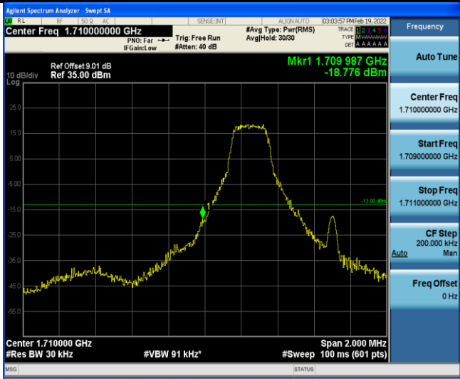
Band4-1.4MHz-QPSK-19957-1RB#5
