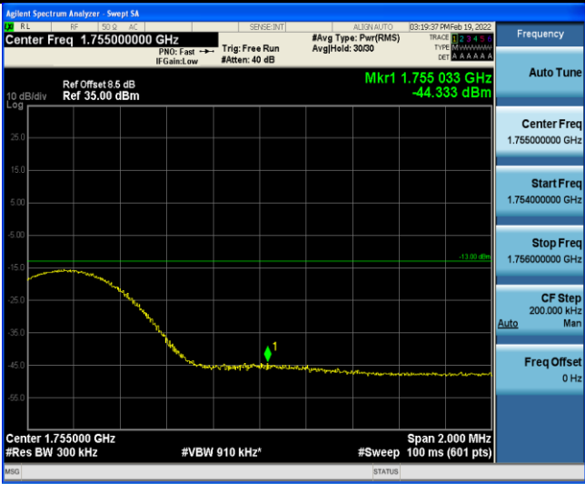
Band4-15MHz-16QAM-20325-1RB#74
