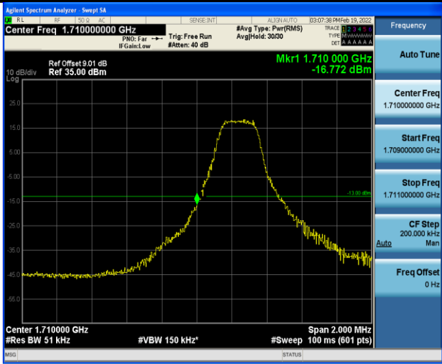
Band4-3MHz-16QAM-19965-1RB#14
