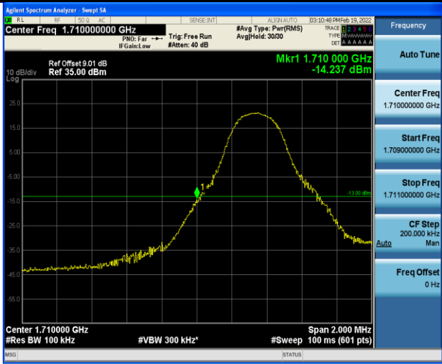
Band4-5MHz-QPSK-19975-1RB#24
