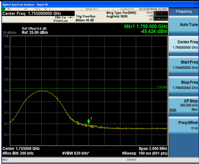
Band4-10MHz-QPSK-20350-1RB#49
