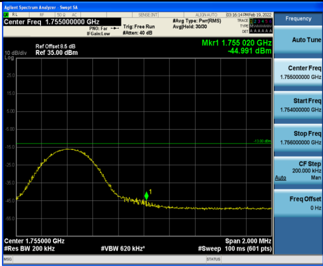
Band4-10MHz-16QAM-20350-1RB#49
