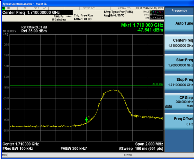
Band4-5MHz-16QAM-19975-25RB#0
