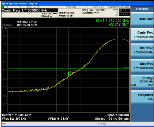
Band4-15MHz-16QAM-20025-1RB#74
