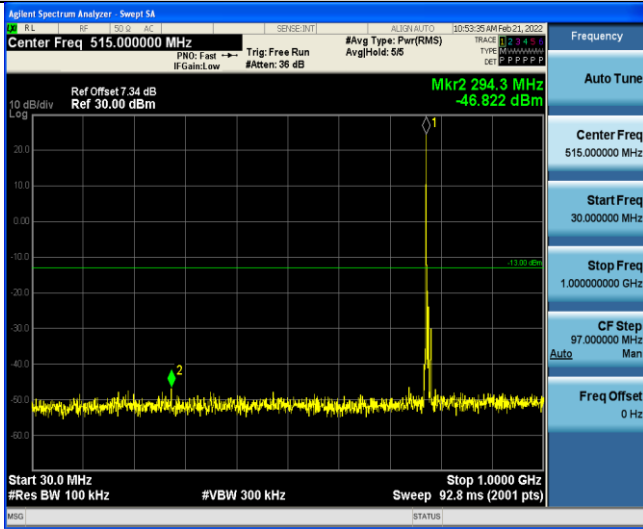
Band13-5MHz-QPSK-23205-1RB#0-Range1:30~1000MHz
