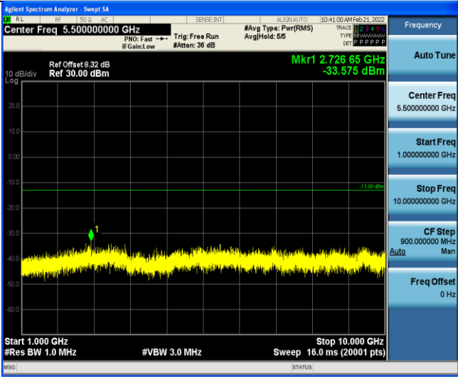
Band12-5MHz-16QAM-23155-1RB#0-Range2:1000~10000MHz
