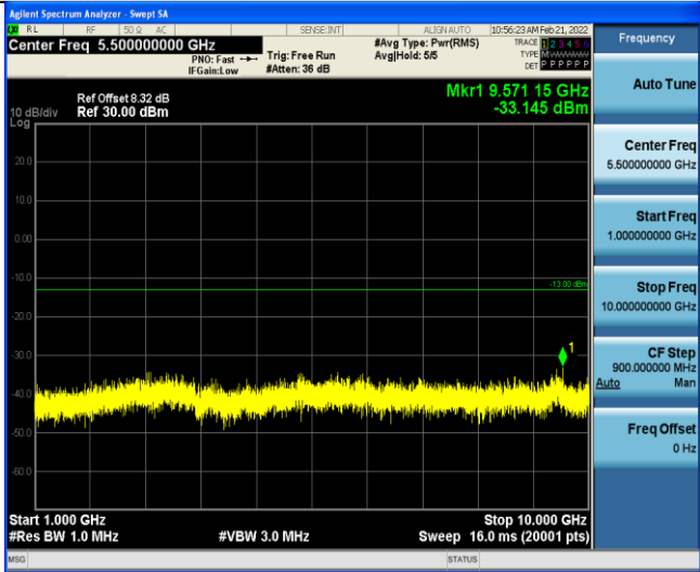
Band13-5MHz-16QAM-23230-1RB#0-Range2:1000~10000MHz
