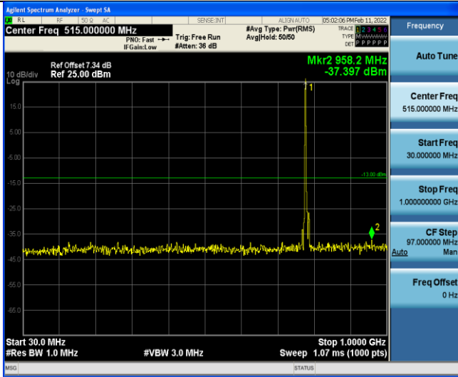
Band13-5MHz-QPSK-23255-1RB#0-Range3:30~1000MHz
