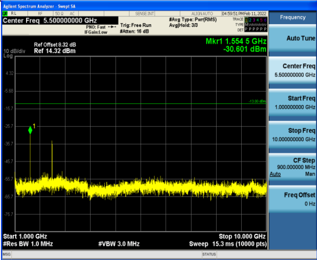
Band13-5MHz-QPSK-23205-1RB#0-Range4:1000~10000MHz
