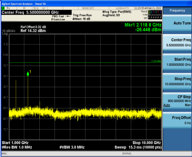
Band12-3MHz-QPSK-23095-1RB#0-Range4:1000~10000MHz
