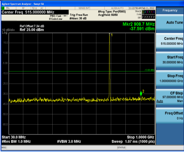
Band12-3MHz-16QAM-23025-1RB#0-Range3:30~1000MHz
