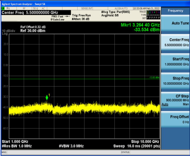
Band12-3MHz-QPSK-23165-1RB#0-Range1:0.009~0.15MHz
