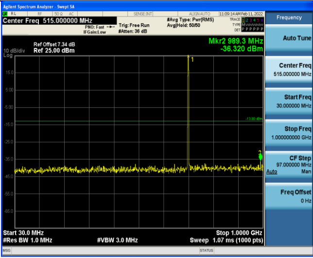
Band12-1.4MHz-16QAM-23095-1RB#0-Range3:30~1000MHz
