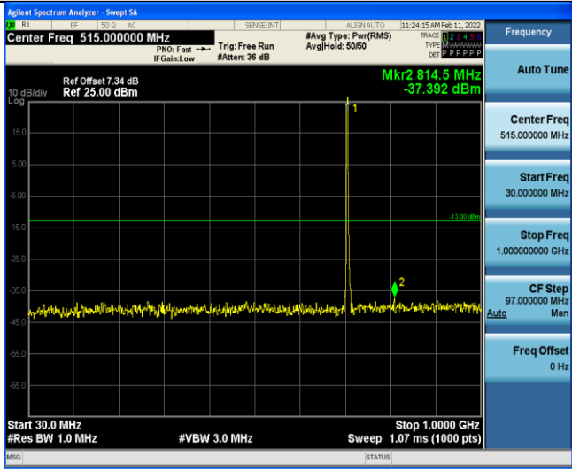
Band12-3MHz-QPSK-23165-1RB#0-Range3:30~1000MHz
