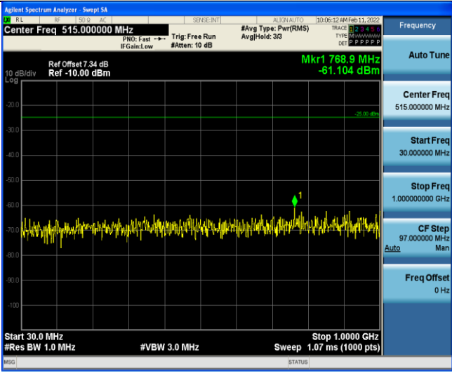
Band7-20MHz-16QAM-20850-1RB#0-Range3:30~1000MHz
