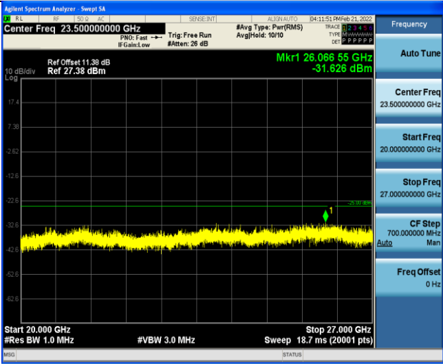
Band7-20MHz-16QAM-21350-1RB#0-Range3:20000~27000MHz
