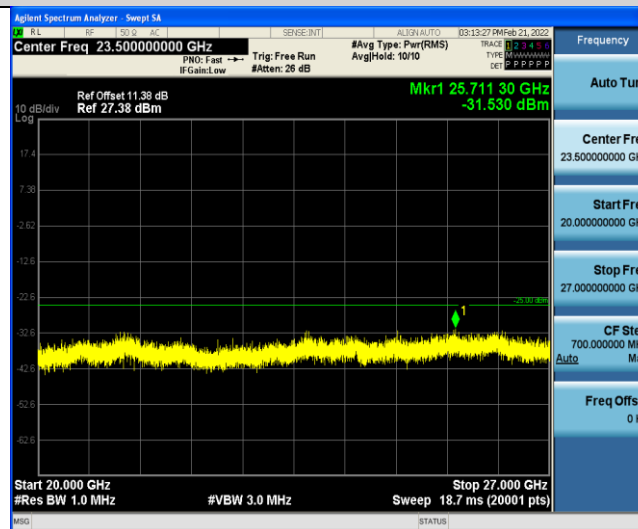
Band7-15MHz-16QAM-21375-1RB#0-Range5:20000~27000MHz
