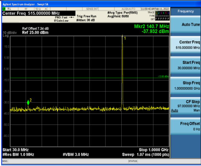
Band12-1.4MHz-QPSK-23173-1RB#0-Range3:30~1000MHz
