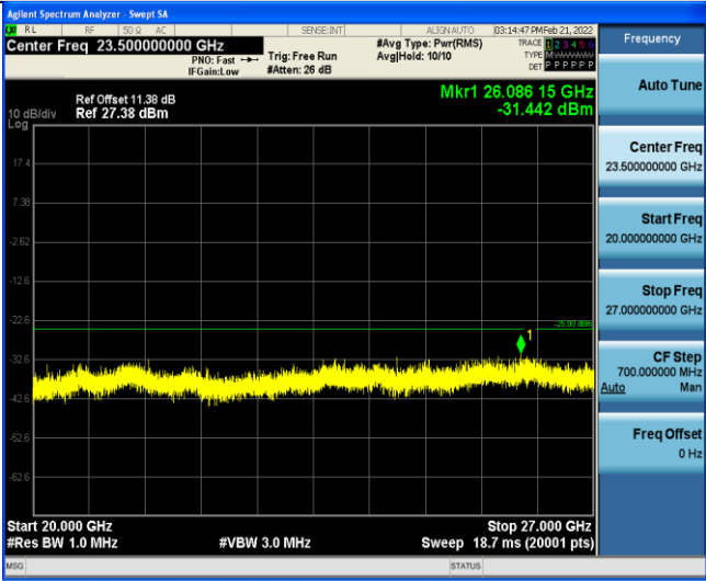
Band7-20MHz-16QAM-20850-1RB#0-Range5:20000~27000MHz
