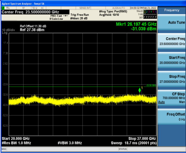
Band7-20MHz-16QAM-21100-1RB#0-Range3:20000~27000MHz
