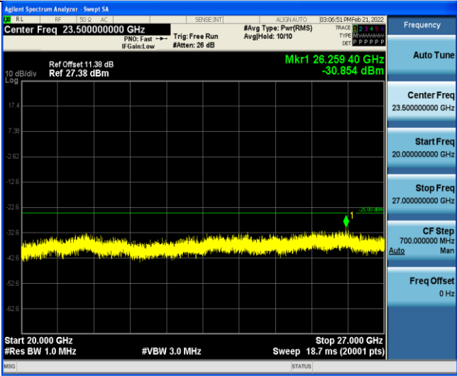
Band7-10MHz-16QAM-20800-1RB#0-Range5:20000~27000MHz
