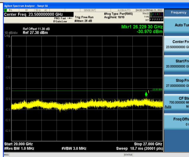
Band7-15MHz-16QAM-20825-1RB#0-Range3:20000~27000MHz
