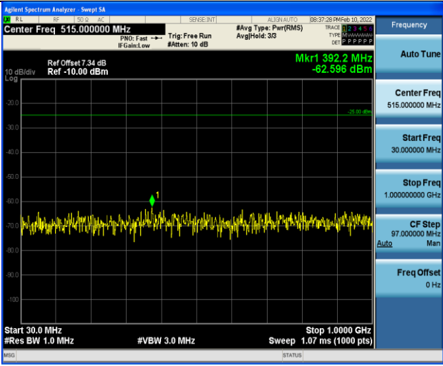
Band7-10MHz-16QAM-21100-1RB#0-Range3:30~1000MHz
