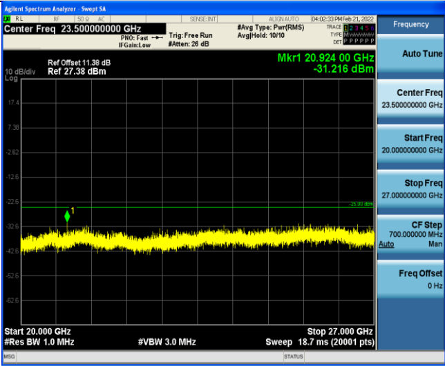
Band7-15MHz-16QAM-21100-1RB#0-Range3:20000~27000MHz
