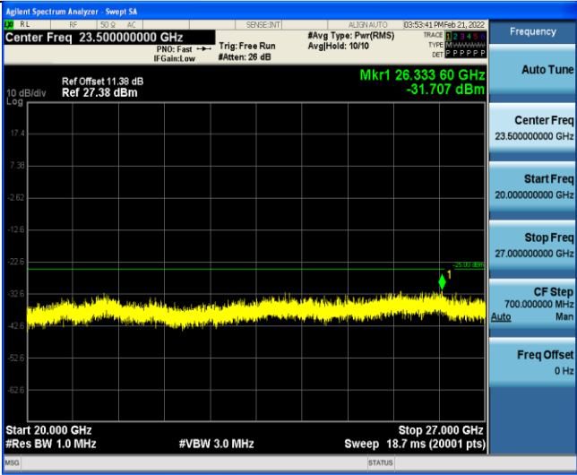
Band7-10MHz-16QAM-21400-1RB#0-Range3:20000~27000MHz
