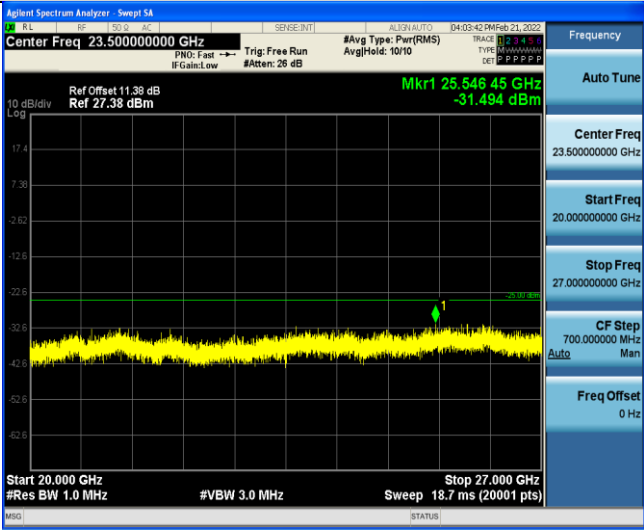
Band7-15MHz-QPSK-21375-1RB#0-Range3:20000~27000MHz
