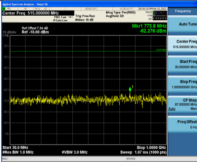
Band7-10MHz-16QAM-20800-1RB#0-Range3:30~1000MHz
