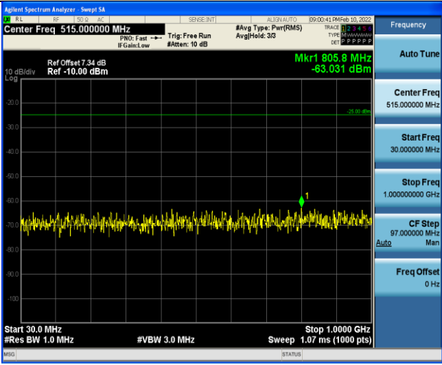
Band7-15MHz-16QAM-20825-1RB#0-Range3:30~1000MHz
