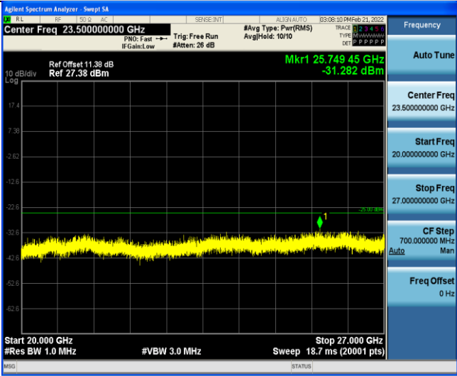
Band7-10MHz-16QAM-21100-1RB#0-Range5:20000~27000MHz
