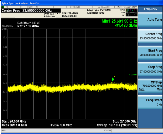
Band7-15MHz-QPSK-21100-1RB#0-Range3:20000~27000MHz
