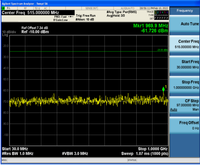
Band7-15MHz-16QAM-21375-1RB#0-Range3:30~1000MHz
