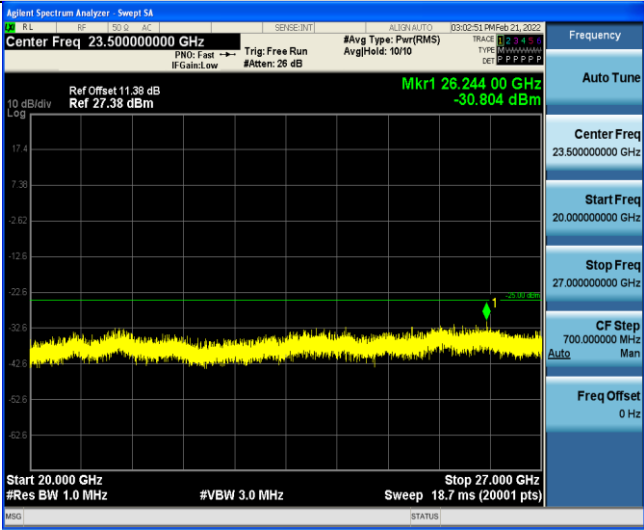
Band7-5MHz-16QAM-20775-1RB#0-Range5:20000~27000MHz
