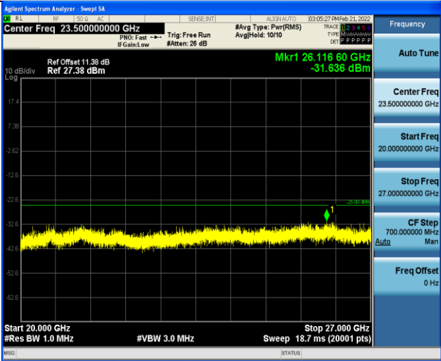
Band7-5MHz-16QAM-21425-1RB#0-Range5:20000~27000MHz
