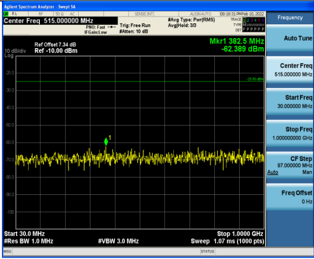
Band7-5MHz-16QAM-21425-1RB#0-Range3:30~1000MHz
