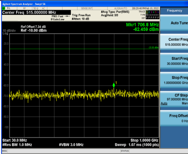
Band7-5MHz-16QAM-20775-1RB#0-Range3:30~1000MHz
