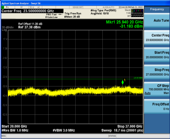
Band7-5MHz-16QAM-21100-1RB#0-Range3:20000~27000MHz
