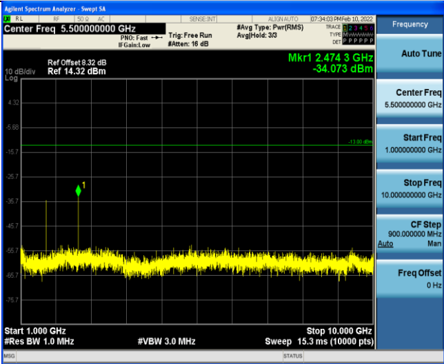
Band5-10MHz-16QAM-20450-1RB#0-Range4:1000~10000MHz
