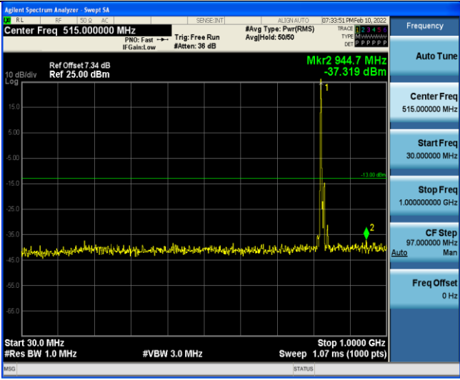
Band5-10MHz-16QAM-20450-1RB#0-Range3:30~1000MHz
