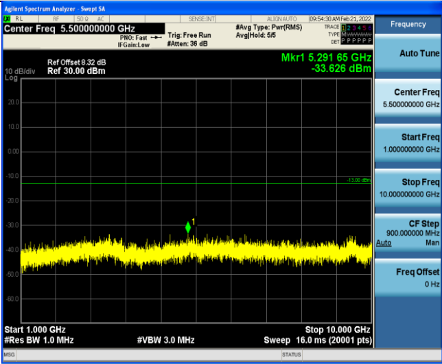
Band5-5MHz-16QAM-20525-1RB#0-Range2:1000~10000MHz
