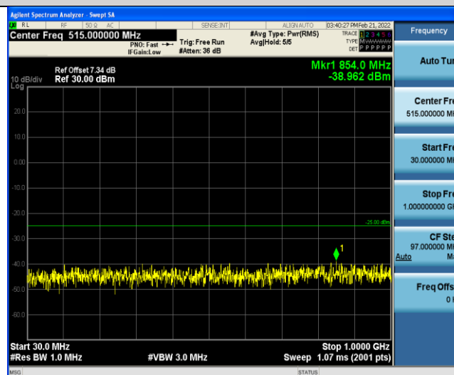
Band7-5MHz-QPSK-20775-1RB#0-Range1:30~1000MHz
