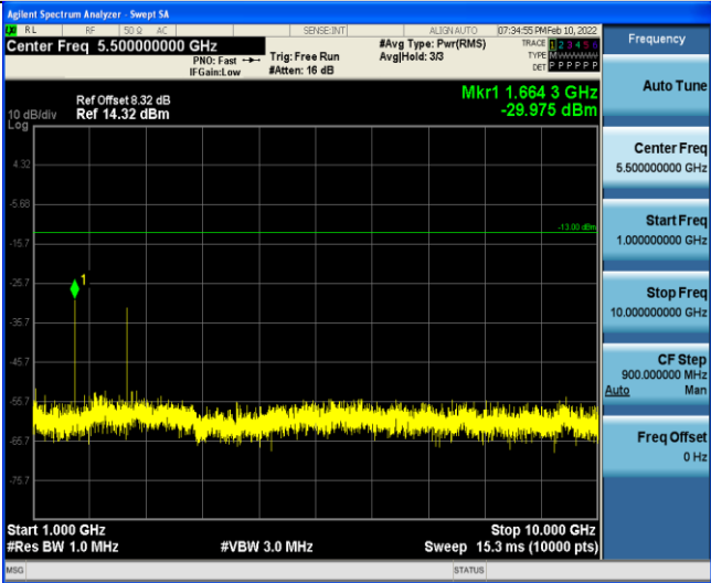
Band5-10MHz-16QAM-20525-1RB#0-Range4:1000~10000MHz
