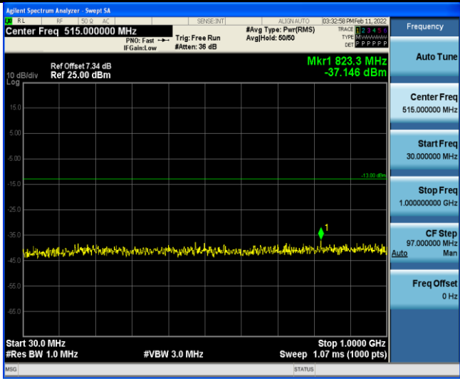
Band4-5MHz-QPSK-20175-1RB#0-Range3:30~1000MHz
