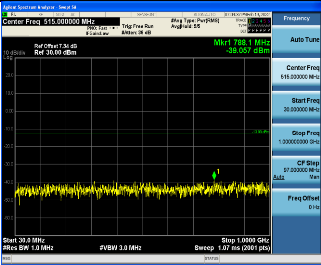
Band4-5MHz-16QAM-20175-1RB#0-Range1:30~1000MHz
