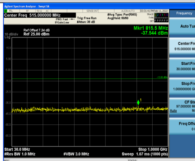
Band4-5MHz-QPSK-19975-1RB#0-Range3:30~1000MHz
