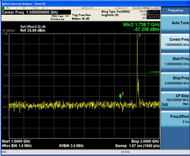
Band2-10MHz-16QAM-18650-1RB#0-Range4:1000~20000MHz
