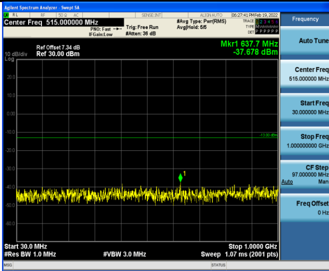
Band2-5MHz-QPSK-18900-1RB#0-Range1:30~1000MHz
