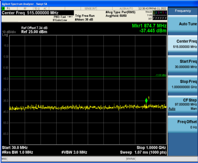
Band2-1.4MHz-16QAM-19193-1RB#0-Range3:30~1000MHz
