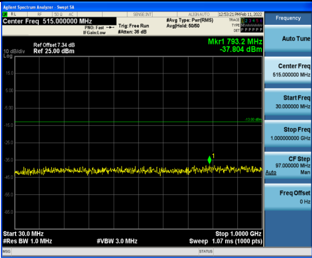
Band2-3MHz-16QAM-18900-1RB#0-Range3:30~1000MHz
