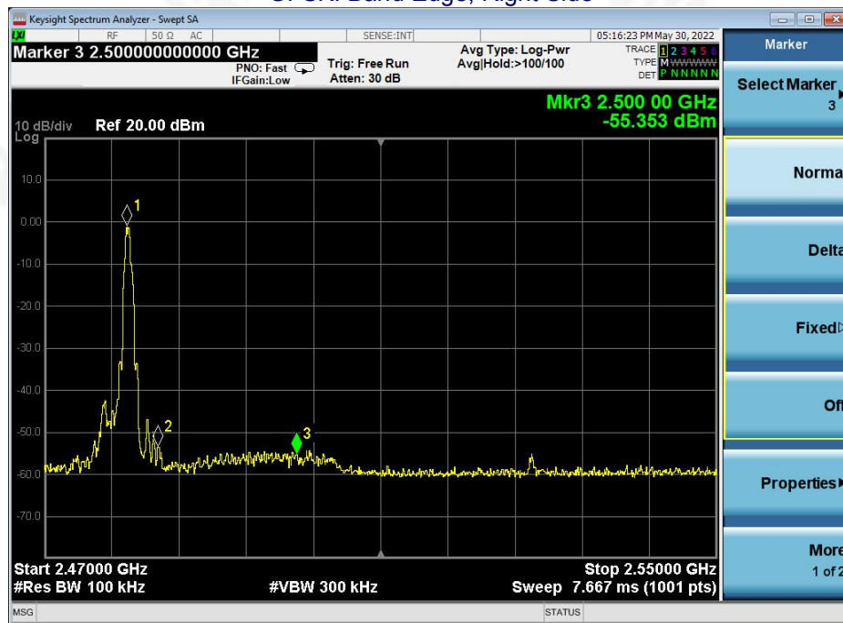
GFSK: Band Edge, Right Side
