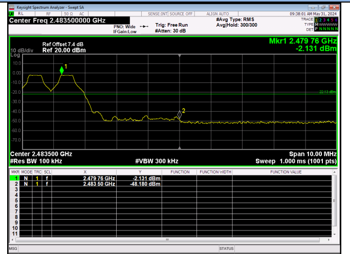
GFSK / Hopping
