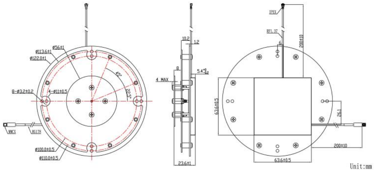
Figure 2. AH323-A7 Dimension View / AH323-A7 三视图
