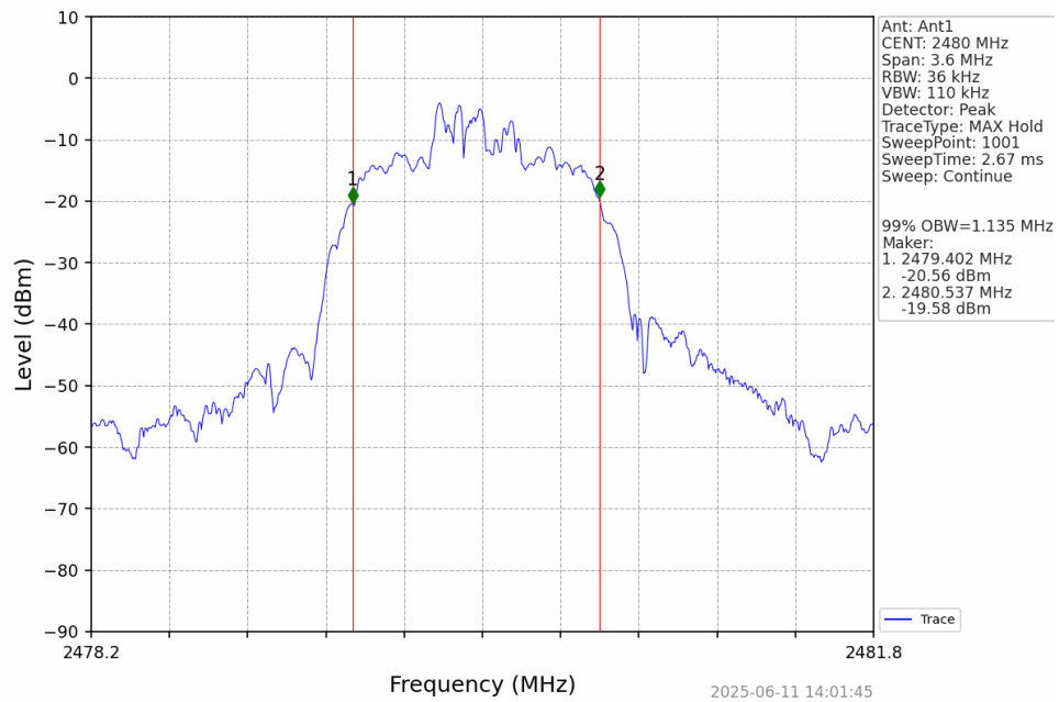
Pi/4DQPSK_2DH5_HCH_2480MHz_Ant1_NTNV
