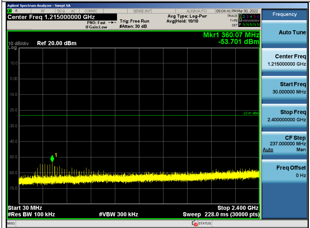
Test_Graph_GFSK_ANT1_2470_1Mbps_Lower Band Emissions
