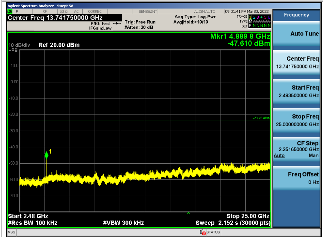
Test_Graph_GFSK_ANT1_2445_1Mbps_Higher Band Emissions
