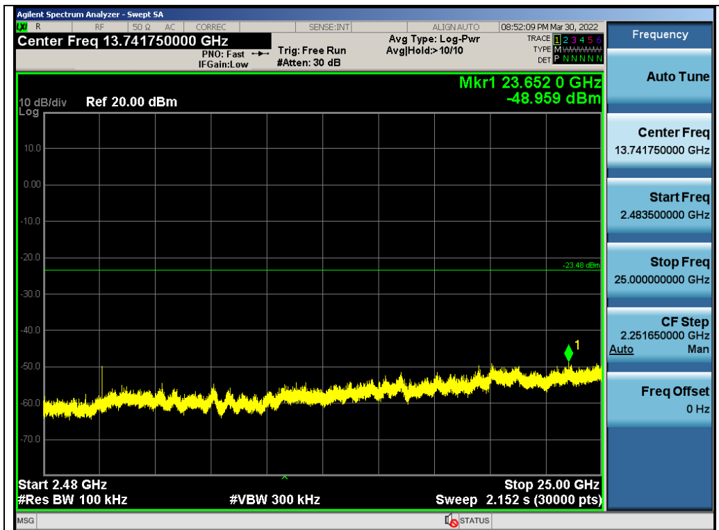
Test_Graph_GFSK_ANT1_2417_1Mbps_Higher Band Emissions
