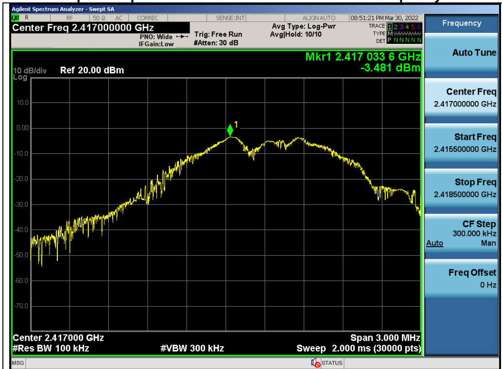
Test_Graph_GFSK_ANT1_2417_1Mbps_Reference Level
