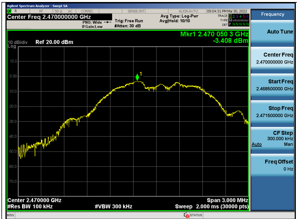
Test_Graph_GFSK_ANT1_2470_1Mbps_Reference Level
