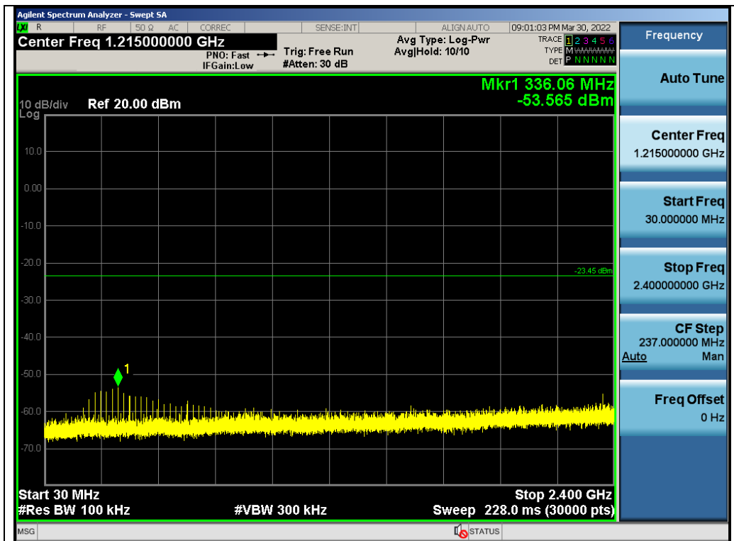
Test_Graph_GFSK_ANT1_2445_1Mbps_Lower Band Emissions
