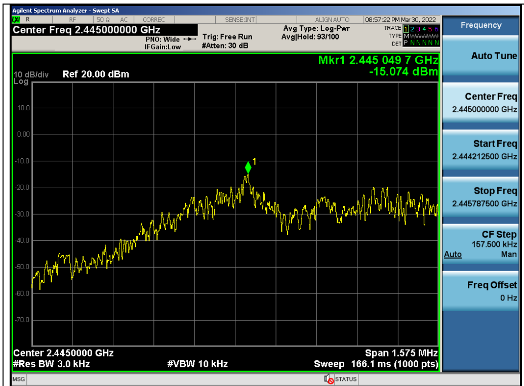
Test_Graph_GFSK_ANT1_2445_1Mbps_PSD
