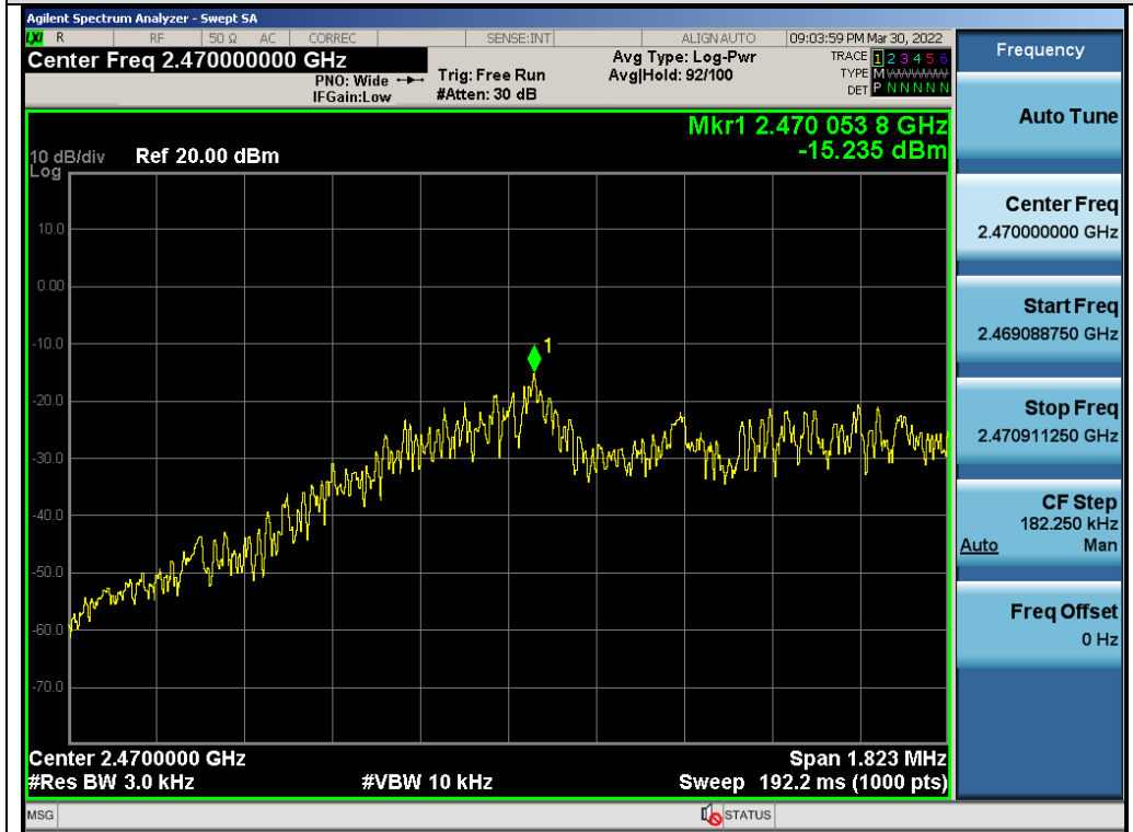
Test_Graph_GFSK_ANT1_2470_1Mbps_PSD
