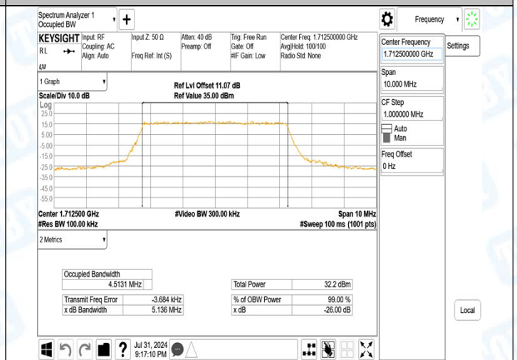
Band4-5MHz-16QAM-20375-25RB#0-PASS
