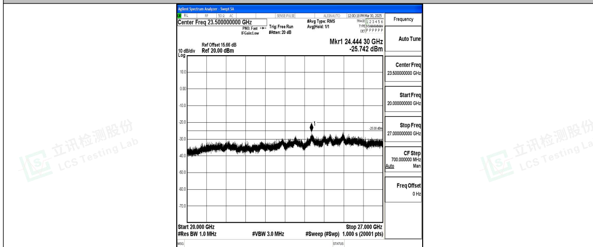
Band7_15MHz_QPSK_21100_1RB#0_20000~27000_20000~27000
