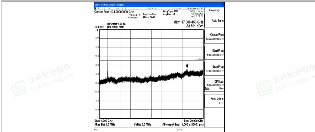
Band7_15MHz_16QAM_20825_1RB#0_1000~20000_1000~20000
