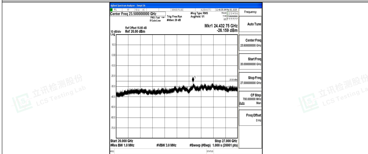
Band7_10MHz_16QAM_21400_1RB#0_20000~27000_20000~27000
