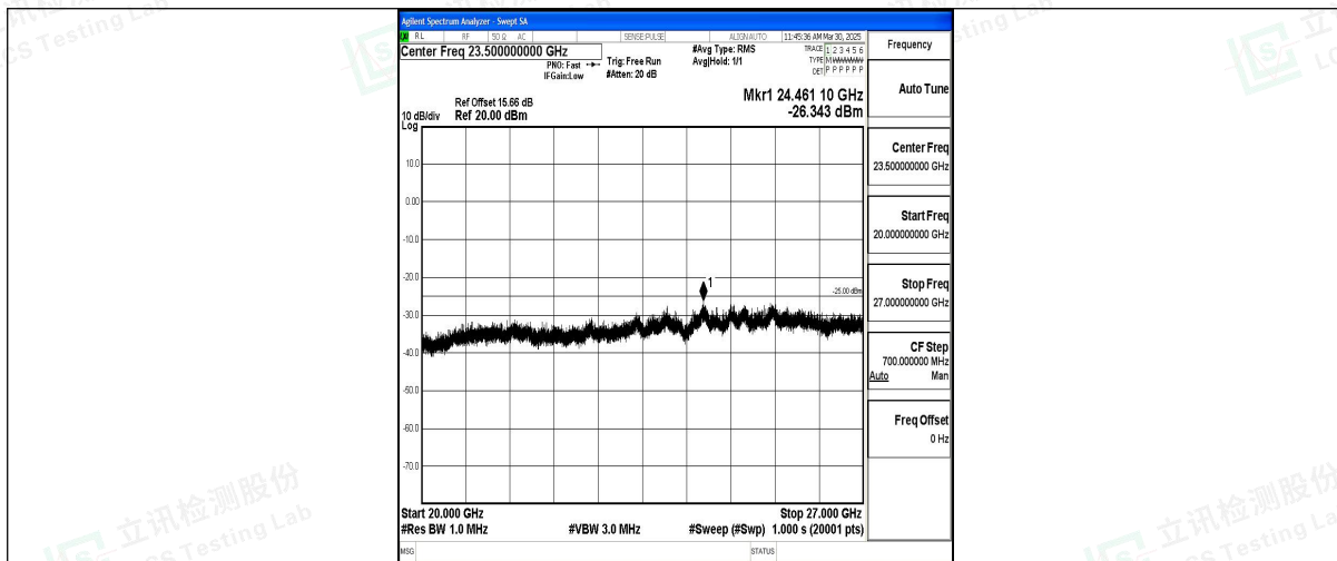
Band7_10MHz_QPSK_21400_1RB#0_20000~27000_20000~27000
