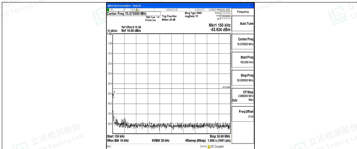
Band7_15MHz_16QAM_20825_1RB#0_0.15~30_0.15~30
