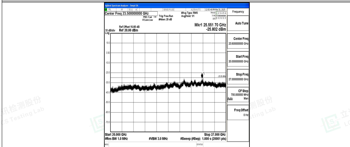
Band7_15MHz_16QAM_21100_1RB#0_20000~27000_20000~27000
