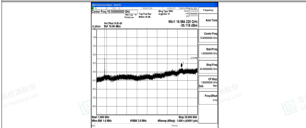
Band7_15MHz_QPSK_21100_1RB#0_1000~20000_1000~20000
