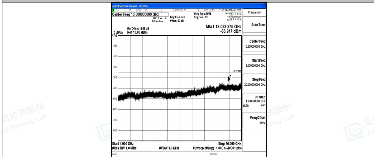
Band7_10MHz_16QAM_21400_1RB#0_1000~20000_1000~20000
