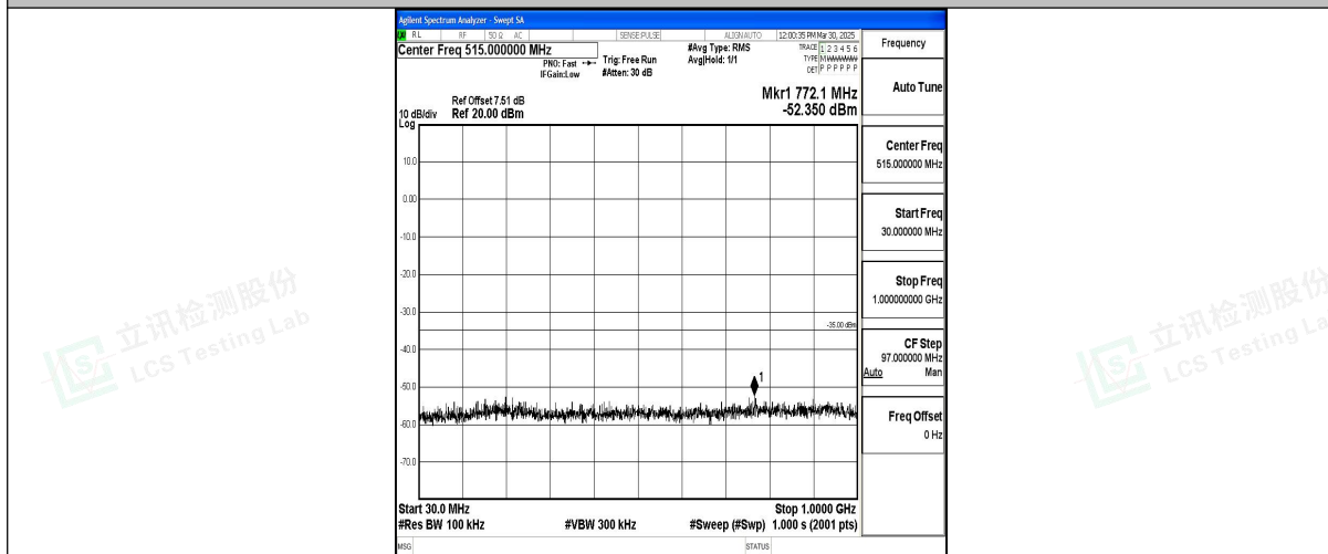
Band7_15MHz_16QAM_21100_1RB#0_30~1000_30~1000
