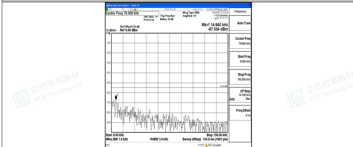
Band7_15MHz_16QAM_20825_1RB#0_0.009~0.15_0.009~0.15
