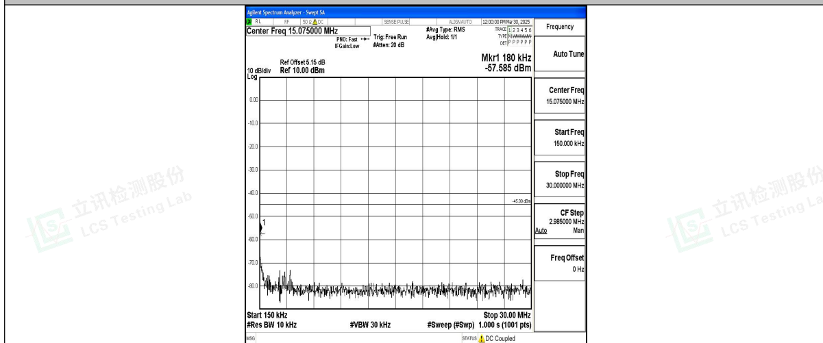
Band7_15MHz_QPSK_21100_1RB#0_0.15~30_0.15~30
