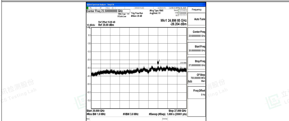
Band7_15MHz_QPSK_20825_1RB#0_20000~27000_20000~27000
