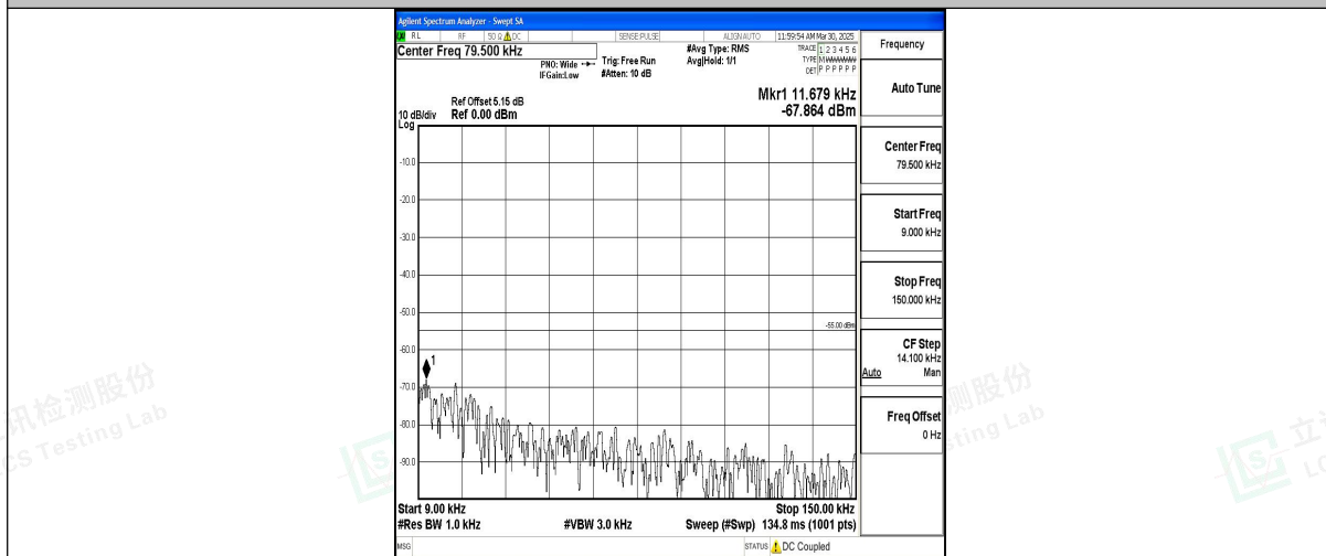
Band7_15MHz_QPSK_21100_1RB#0_0.009~0.15_0.009~0.15
