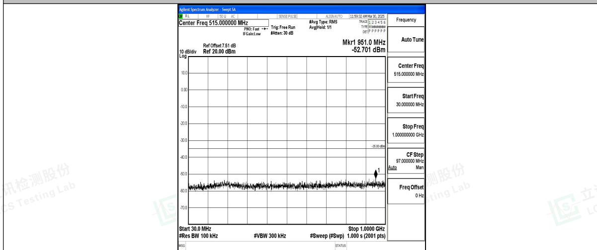
Band7_15MHz_16QAM_20825_1RB#0_30~1000_30~1000
