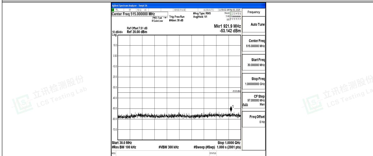
Band7_15MHz_QPSK_20825_1RB#0_30~1000_30~1000
