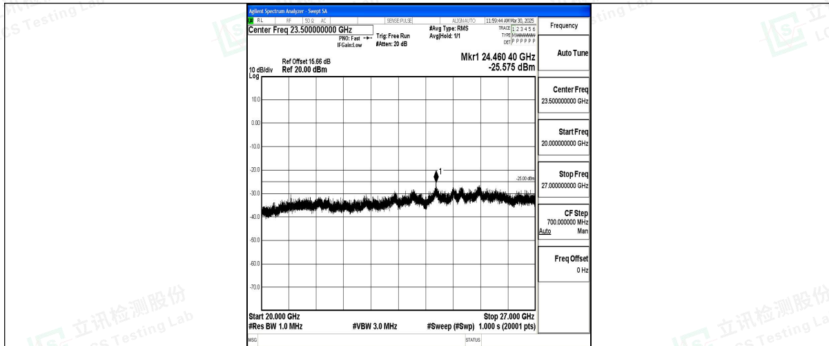
Band7_15MHz_16QAM_20825_1RB#0_20000~27000_20000~27000
