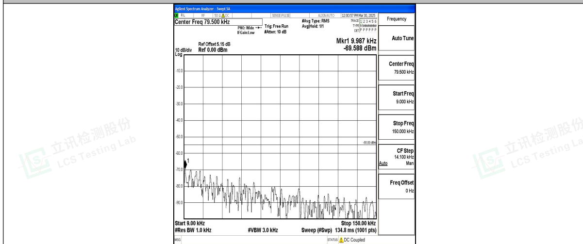
Band7_15MHz_QPSK_21375_1RB#0_0.009~0.15_0.009~0.15
