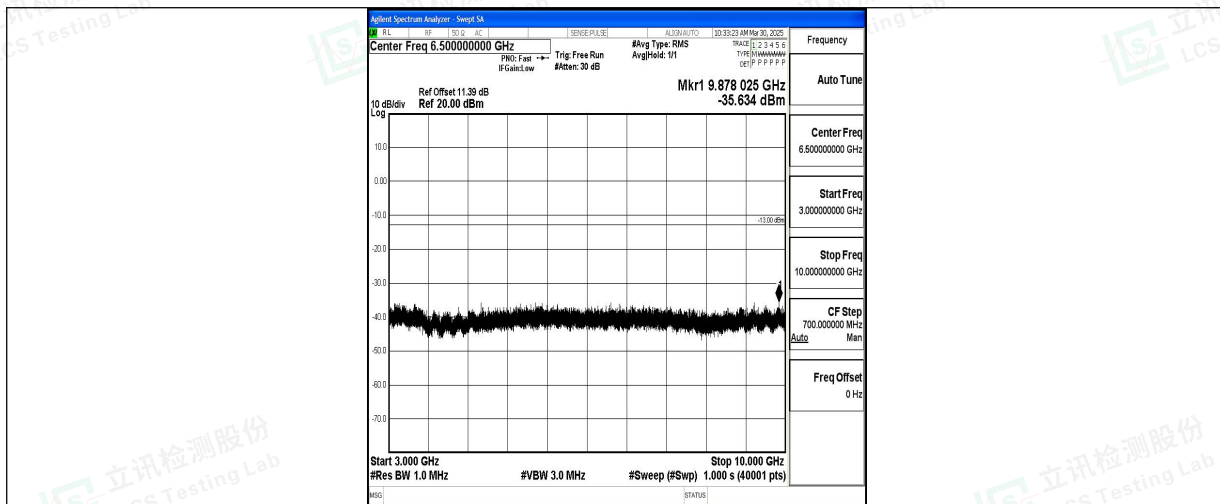
Band5_3MHz_QPSK_20635_1RB#0_3000~10000_3000~10000
