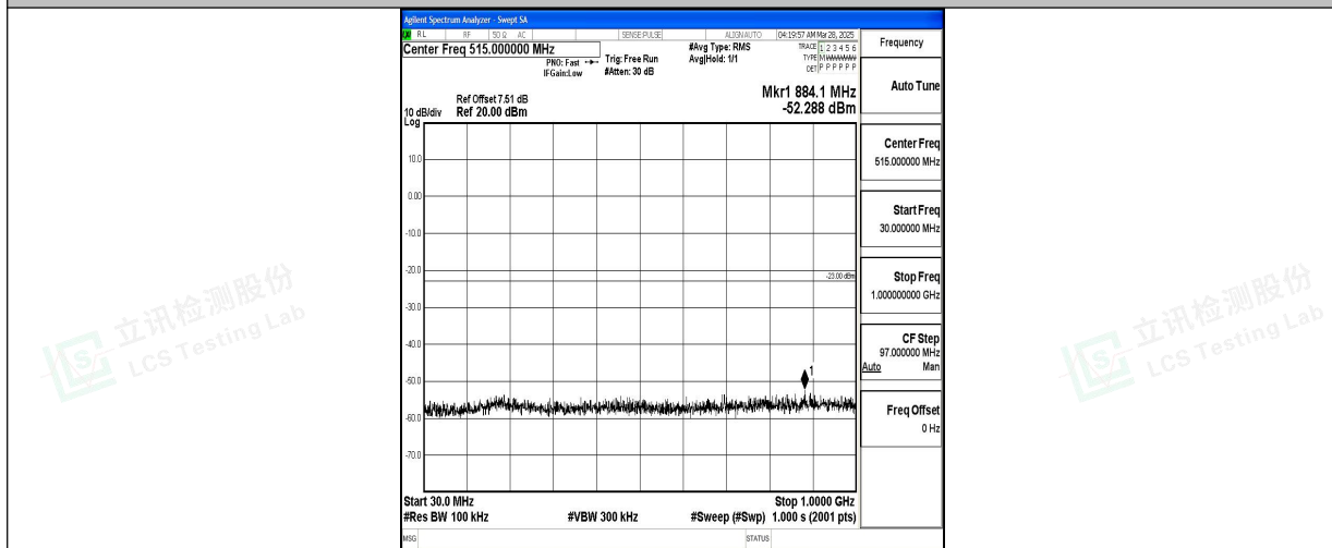
Band4_3MHz_QPSK_20385_1RB#0_30~1000_30~1000
