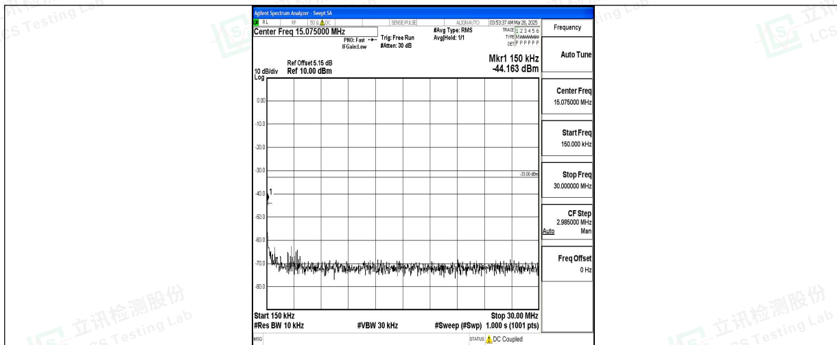
Band4_1.4MHz_16QAM_20393_1RB#0_0.15~30_0.15~30
