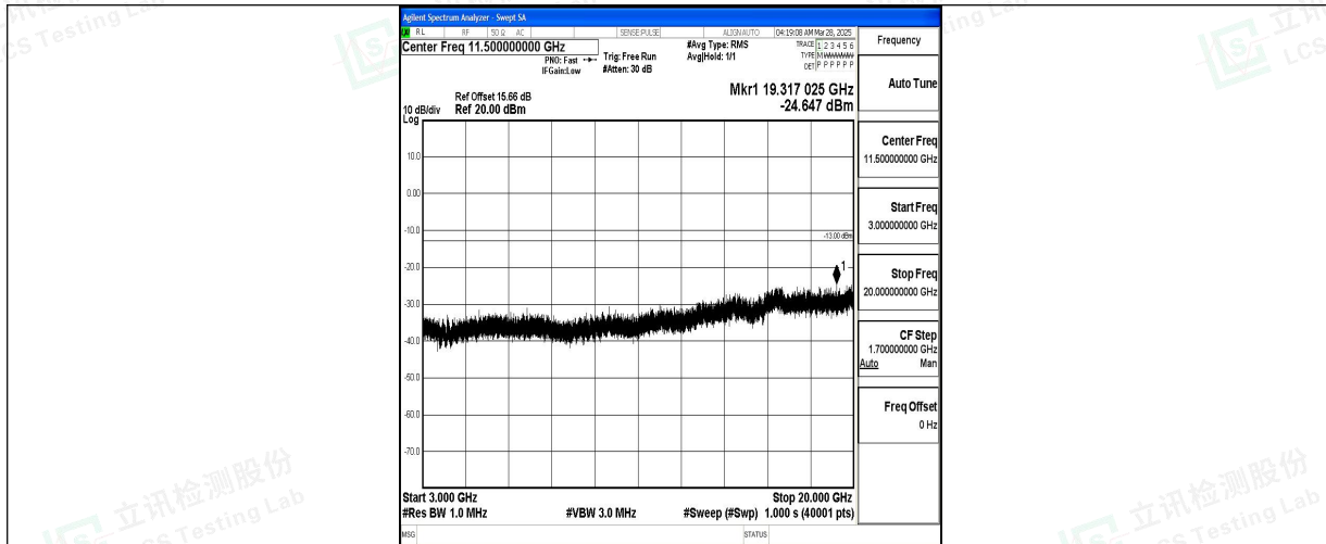
Band4_3MHz_QPSK_20175_1RB#0_3000~20000_3000~20000
