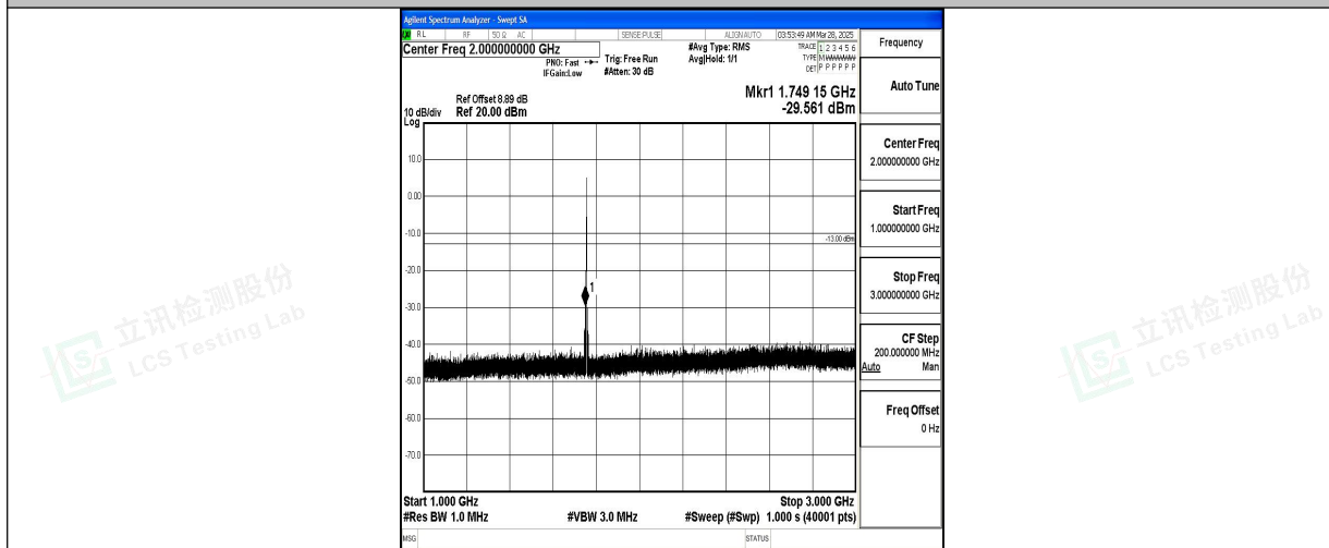
Band4_1.4MHz_16QAM_20393_1RB#0_1000~3000_1000~3000
