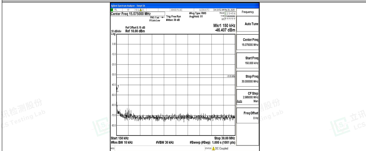
Band4_3MHz_QPSK_20385_1RB#0_0.15~30_0.15~30
