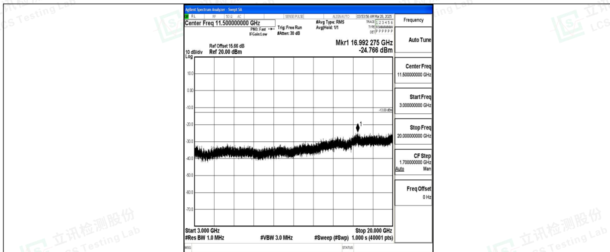
Band4_1.4MHz_16QAM_20393_1RB#0_3000~20000_3000~20000
