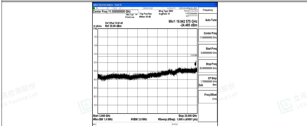
Band4_1.4MHz_QPSK_20393_1RB#0_3000~20000_3000~20000
