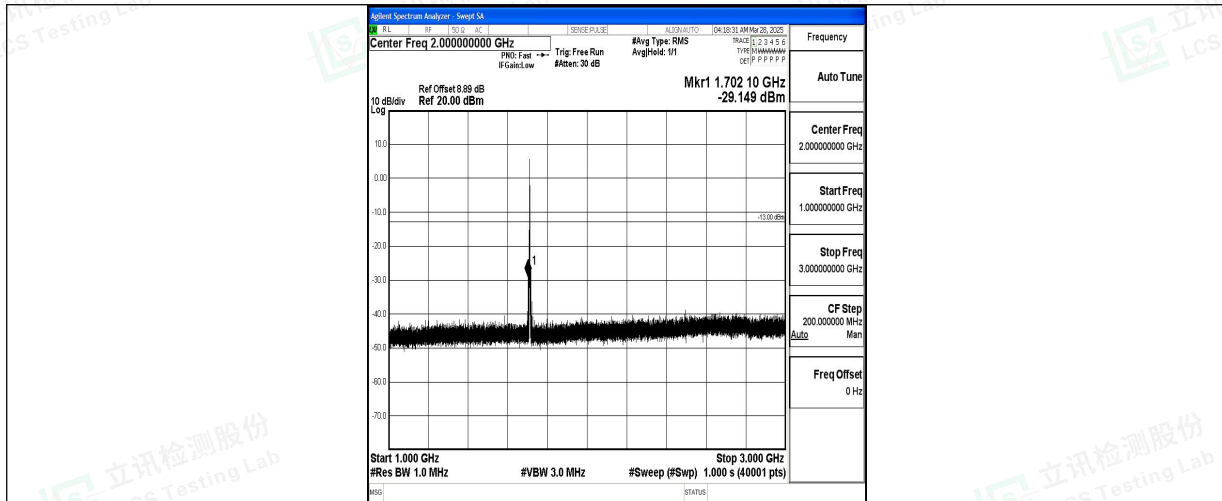
Band4_3MHz_16QAM_19965_1RB#0_1000~3000_1000~3000
