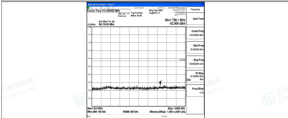
Band4_3MHz_QPSK_20175_1RB#0_30~1000_30~1000
