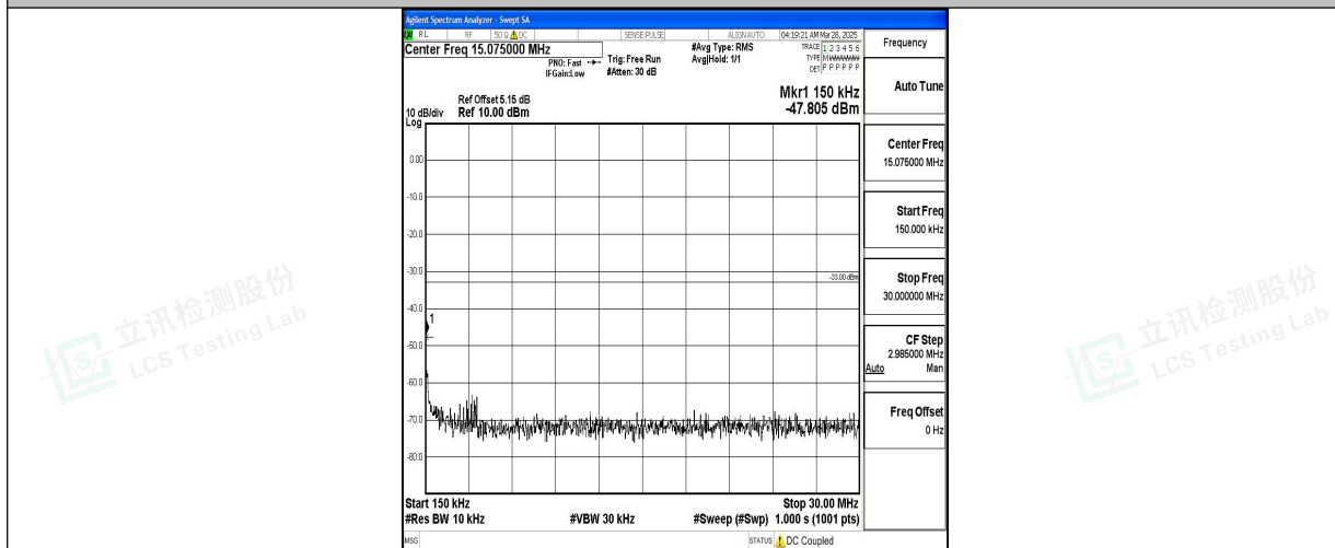
Band4_3MHz_16QAM_20175_1RB#0_0.15~30_0.15~30
