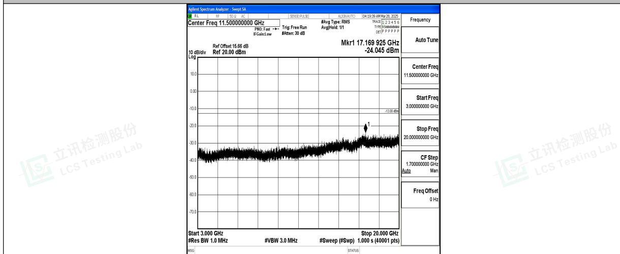
Band4_3MHz_16QAM_20175_1RB#0_3000~20000_3000~20000
