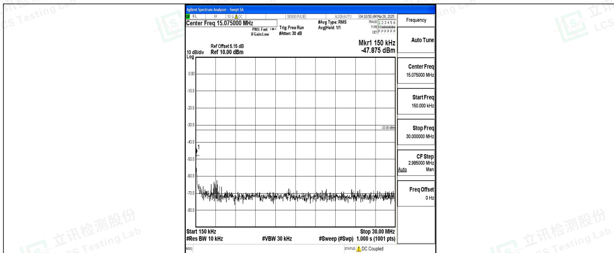
Band4_3MHz_QPSK_20175_1RB#0_0.15~30_0.15~30
