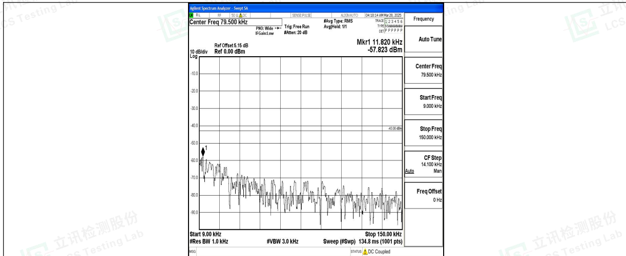
Band4_3MHz_16QAM_19965_1RB#0_0.009~0.15_0.009~0.15
