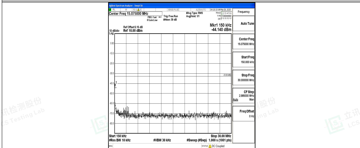
Band4_3MHz_16QAM_19965_1RB#0_0.15~30_0.15~30
