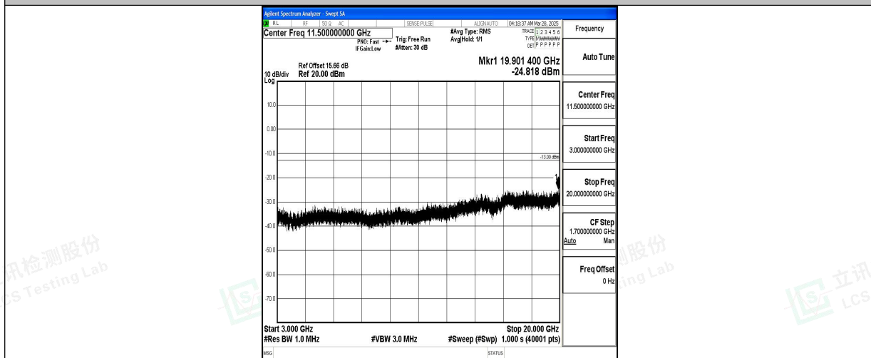
Band4_3MHz_16QAM_19965_1RB#0_3000~20000_3000~20000
