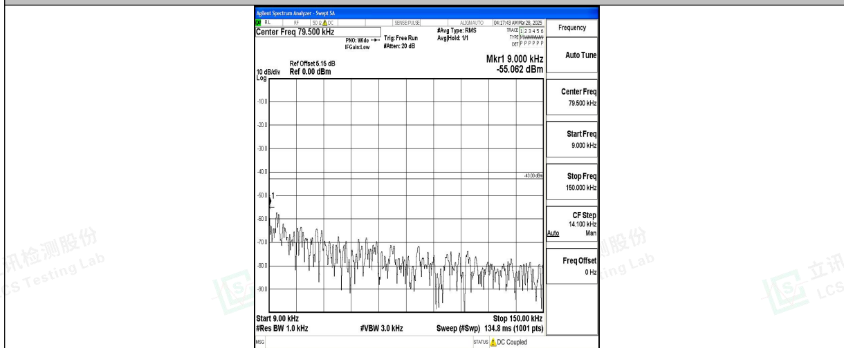
Band4_3MHz_QPSK_19965_1RB#0_0.009~0.15_0.009~0.15
