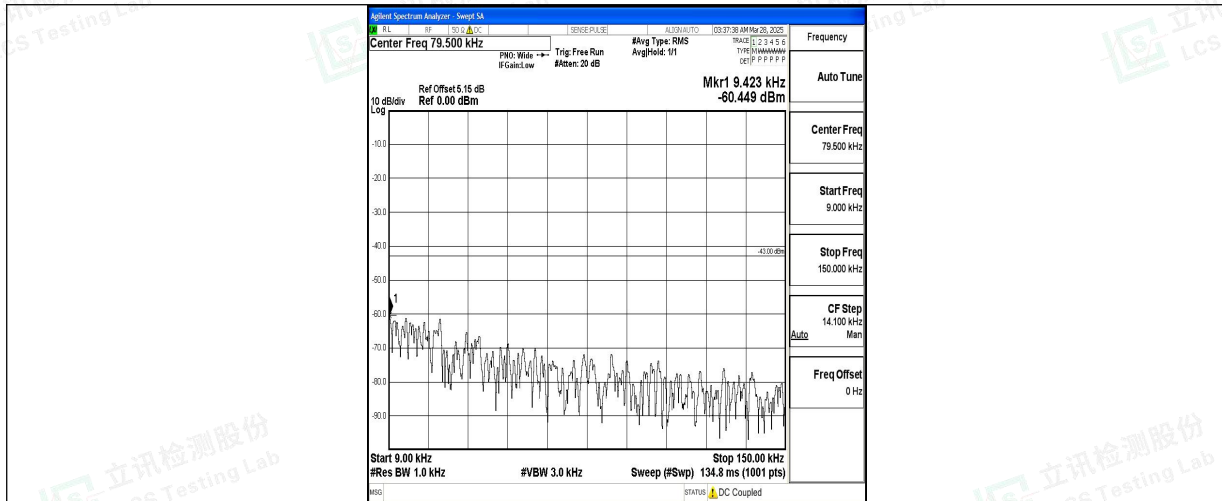
Band2_20MHz_16QAM_19100_1RB#0_0.009~0.15_0.009~0.15
