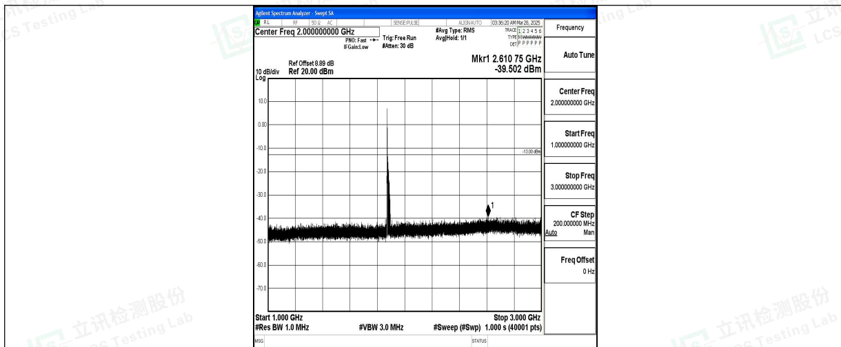
Band2_20MHz_QPSK_18900_1RB#0_1000~3000_1000~3000
