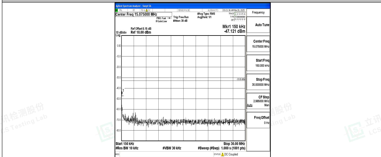
Band2_15MHz_16QAM_19125_1RB#0_0.15~30_0.15~30
