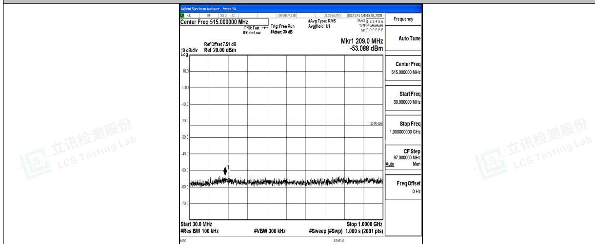
Band2_15MHz_16QAM_19125_1RB#0_30~1000_30~1000
