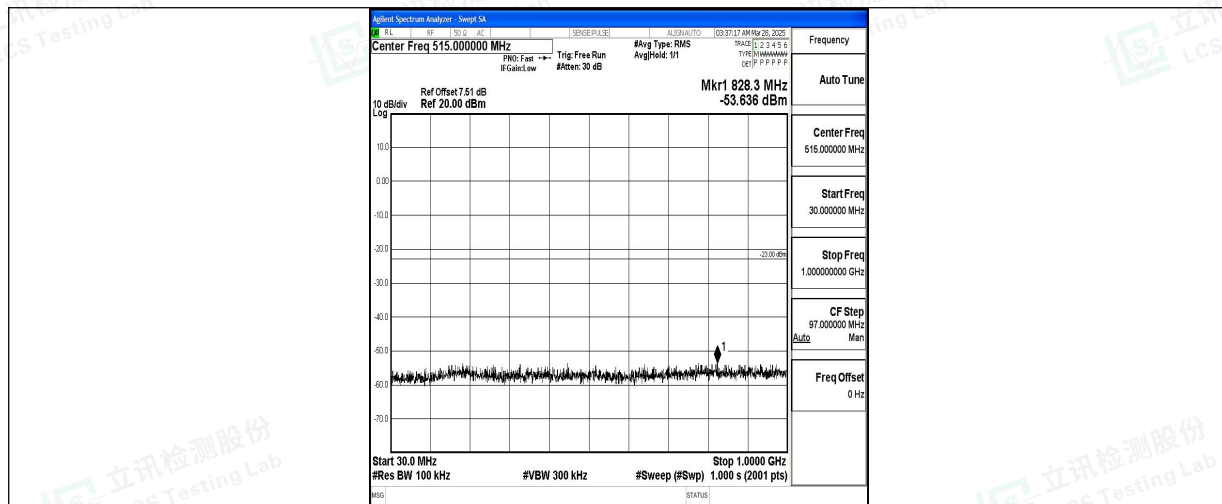
Band2_20MHz_QPSK_19100_1RB#0_30~1000_30~1000
