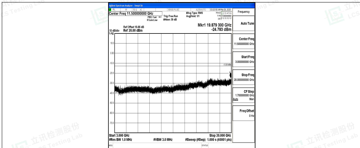
Band2_15MHz_16QAM_18900_1RB#0_3000~20000_3000~20000
