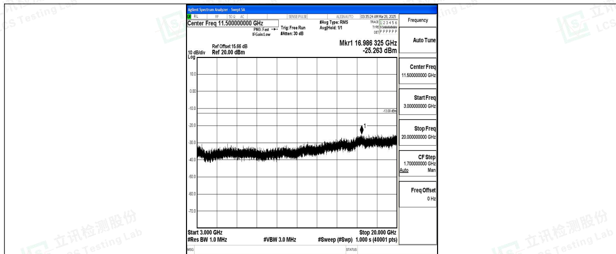
Band2_20MHz_QPSK_18700_1RB#0_3000~20000_3000~20000
