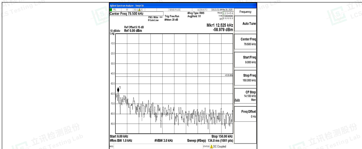
Band2_15MHz_16QAM_19125_1RB#0_0.009~0.15_0.009~0.15
