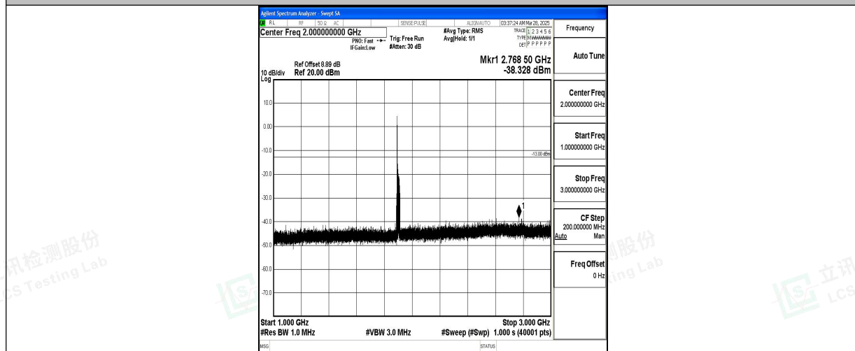
Band2_20MHz_QPSK_19100_1RB#0_1000~3000_1000~3000
