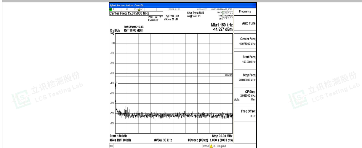
Band2_15MHz_QPSK_19125_1RB#0_0.15~30_0.15~30
