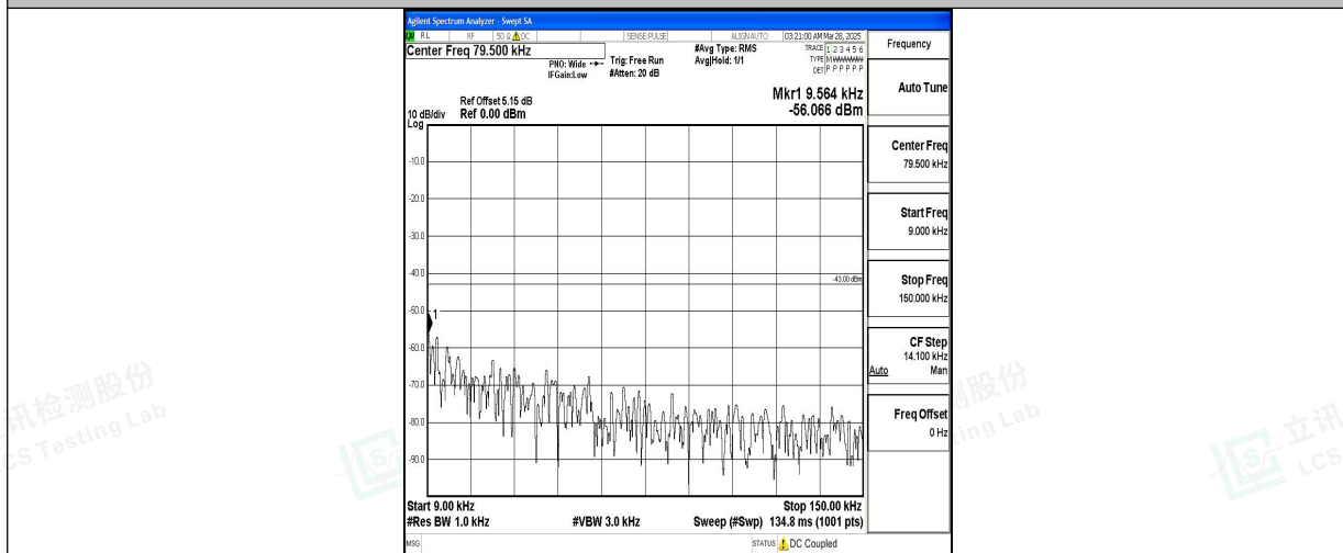
Band2_15MHz_QPSK_19125_1RB#0_0.009~0.15_0.009~0.15
