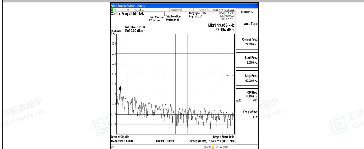
Band2_20MHz_16QAM_18700_1RB#0_0.009~0.15_0.009~0.15
