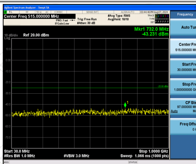
Band7-10MHz-QPSK-21400-1RB#0-Range1:30~1000MHz
