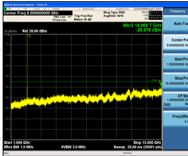
Band7-5MHz-16QAM-21100-1RB#0-Range2:1000~15000MHz
