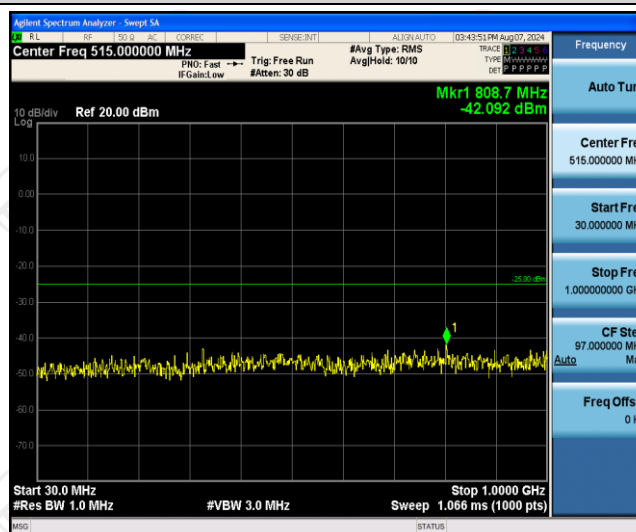
Band7-10MHz-16QAM-21100-1RB#0-Range1:30~1000MHz
