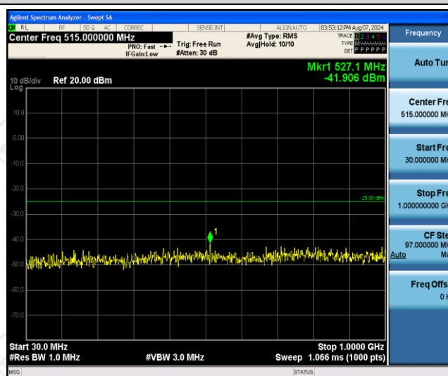
Band7-15MHz-QPSK-21100-1RB#0-Range1:30~1000MHz
