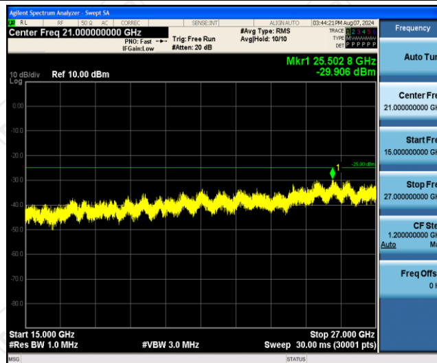
Band7-10MHz-16QAM-21100-1RB#0-Range3:15000~27000MHz
