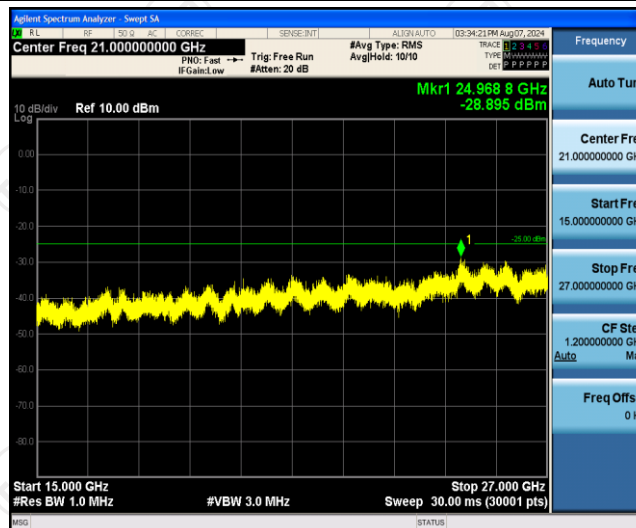
Band7-5MHz-16QAM-21100-1RB#0-Range3:15000~27000MHz
