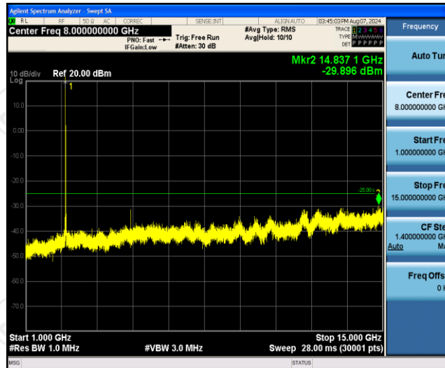
Band7-10MHz-QPSK-21400-1RB#0-Range2:1000~15000MHz
