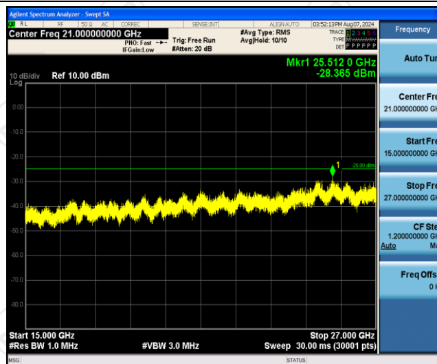
Band7-15MHz-QPSK-20825-1RB#0-Range3:15000~27000MHz
