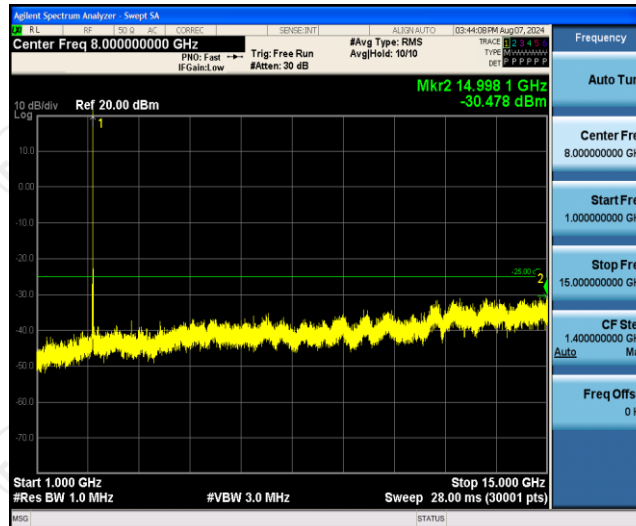
Band7-10MHz-16QAM-21100-1RB#0-Range2:1000~15000MHz
