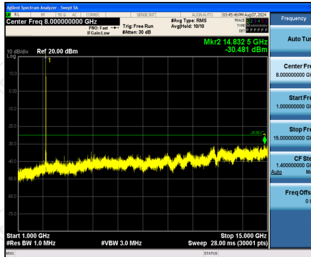
Band7-10MHz-16QAM-21400-1RB#0-Range2:1000~15000MHz
