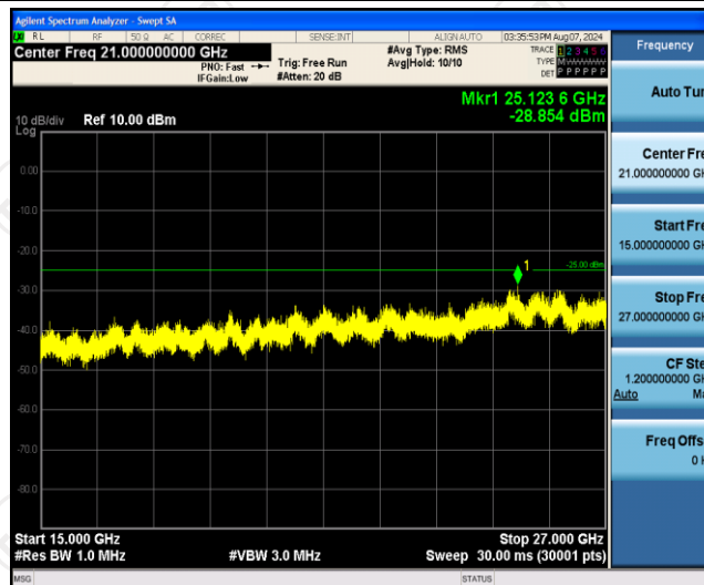
Band7-5MHz-16QAM-21425-1RB#0-Range3:15000~27000MHz
