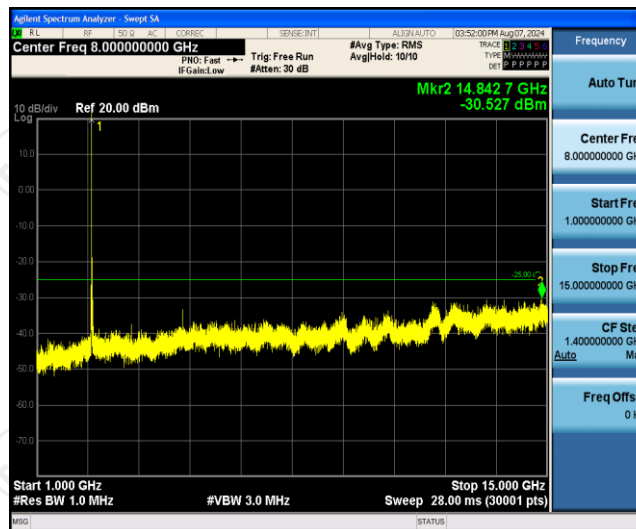
Band7-15MHz-QPSK-20825-1RB#0-Range2:1000~15000MHz
