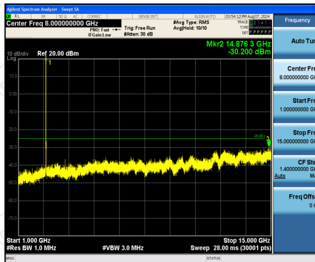
Band7-15MHz-16QAM-21100-1RB#0-Range2:1000~15000MHz
