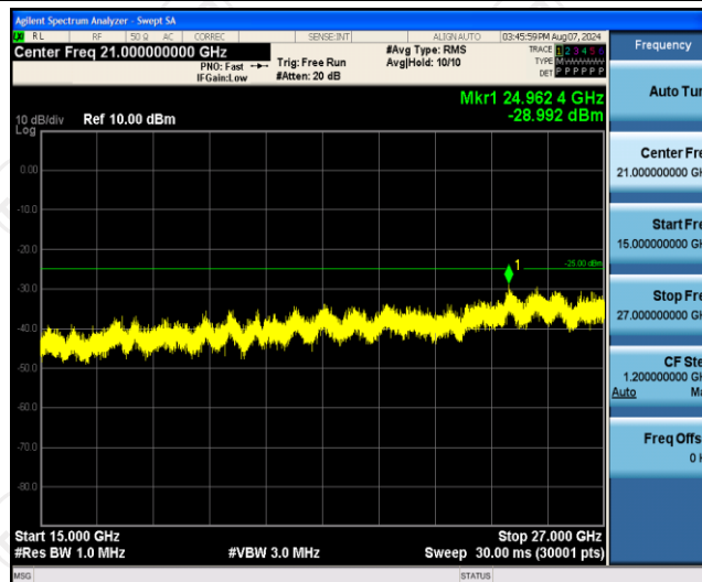
Band7-10MHz-16QAM-21400-1RB#0-Range3:15000~27000MHz
