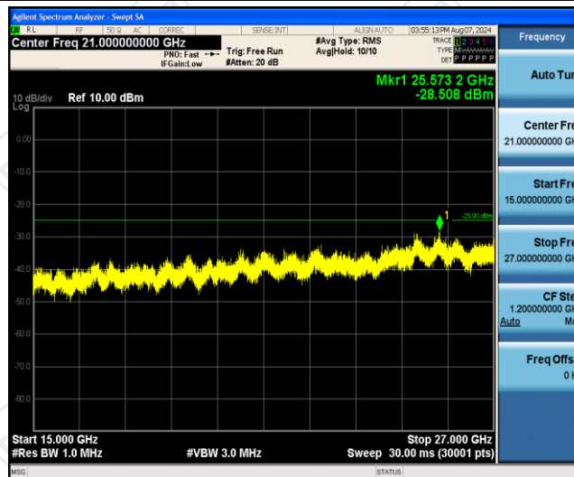
Band7-15MHz-QPSK-21375-1RB#0-Range3:15000~27000MHz
