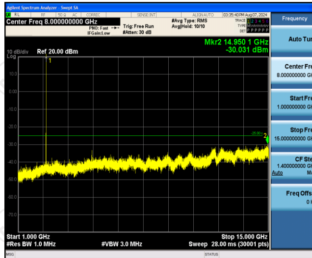
Band7-5MHz-16QAM-21425-1RB#0-Range2:1000~15000MHz
