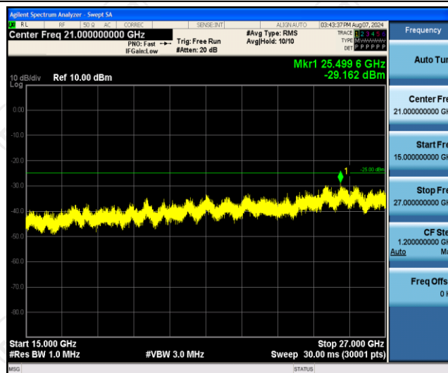
Band7-10MHz-QPSK-21100-1RB#0-Range3:15000~27000MHz
