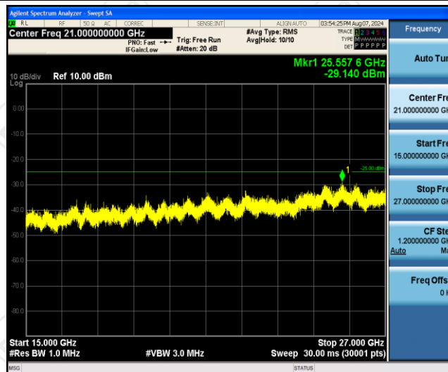
Band7-15MHz-16QAM-21100-1RB#0-Range3:15000~27000MHz
