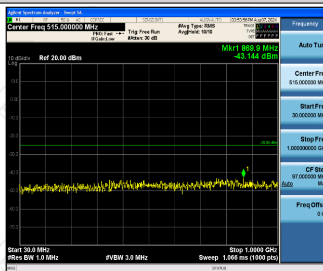
Band7-15MHz-16QAM-21100-1RB#0-Range1:30~1000MHz
