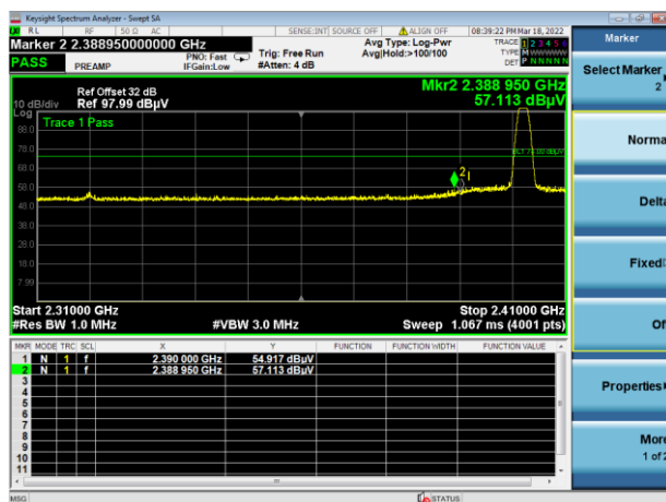
GFSK (BLE 1Mbps) LOW CHANNEL, PEAK
