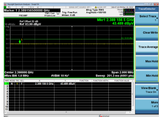
GFSK (BLE 1Mbps) LOW CHANNEL, AVERAGE
