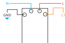
Dimmer switch
