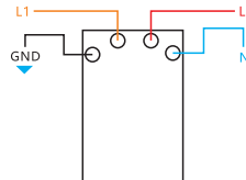
1 gang switch
