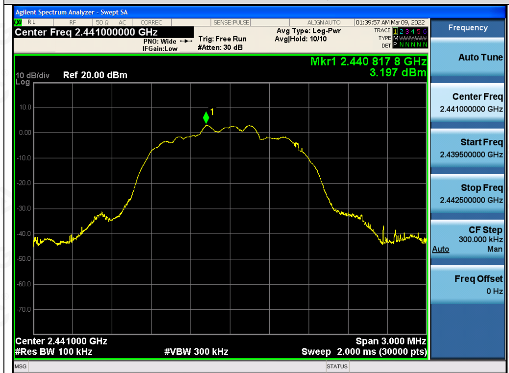
Test_Graph_EDR_ANT1_2441_3Mbps_Reference Level
