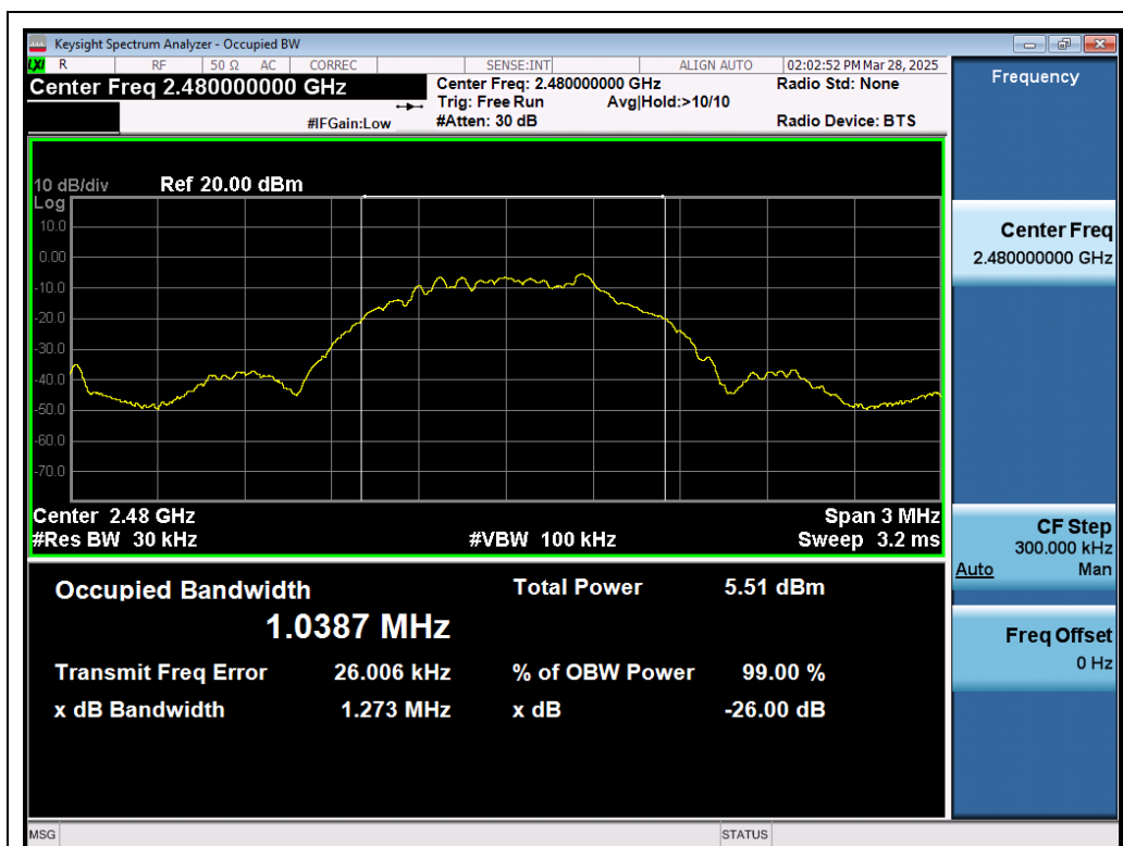
Test_Graph_LE1M_ANT1_2480_1Mbps_OBW
