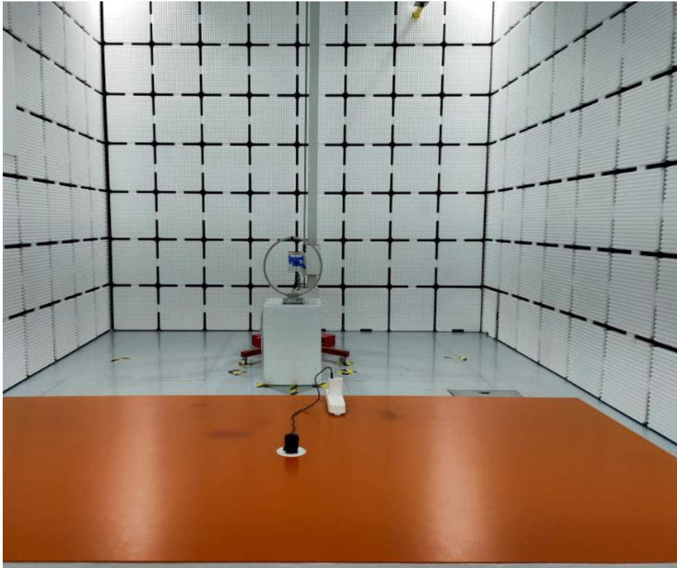
Radiated emissions- Below 30MHz
