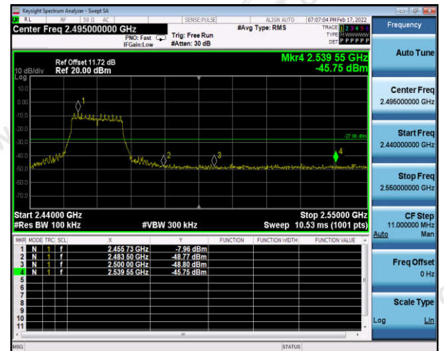
Right bandedge
