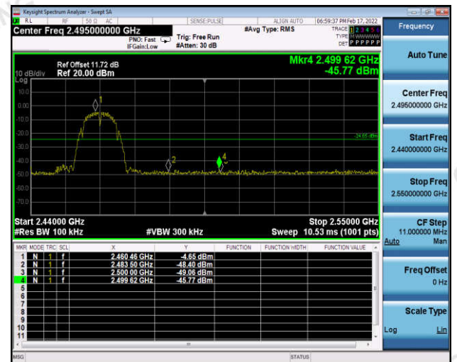
Right bandedge
