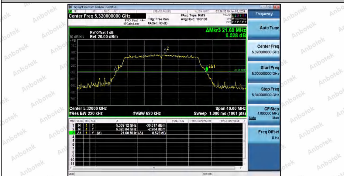
11N20SISO_Ant1_5320
