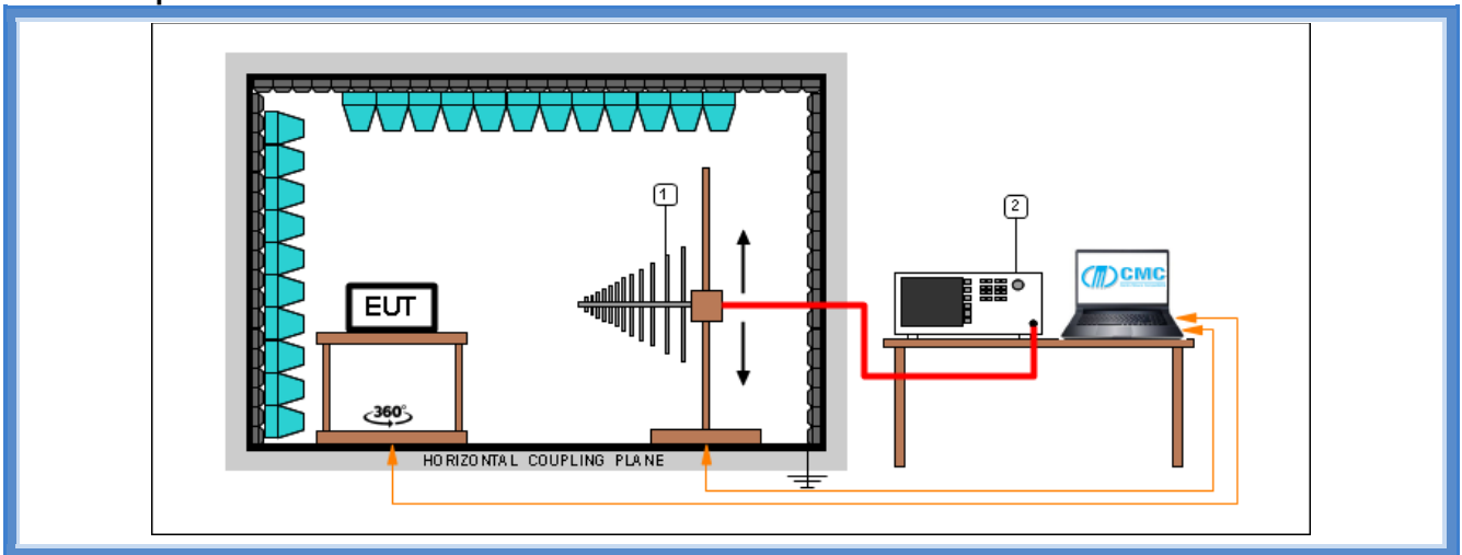
Test setup PE004_02
