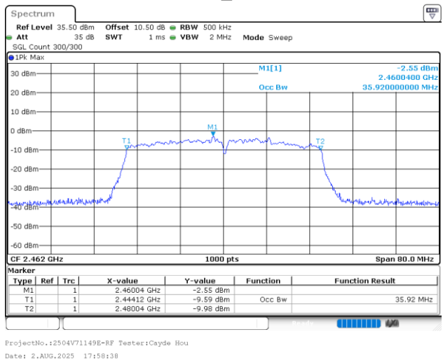
802.11n40_2462MHz
