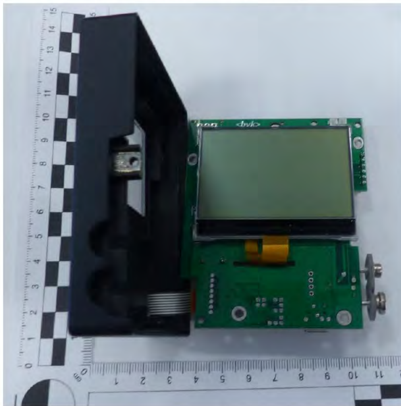
EUT PCB TOP with display
