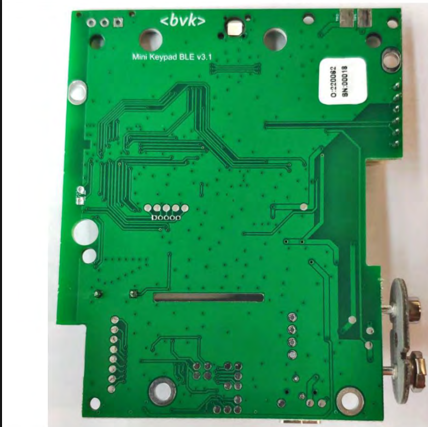
PCB bottom side
