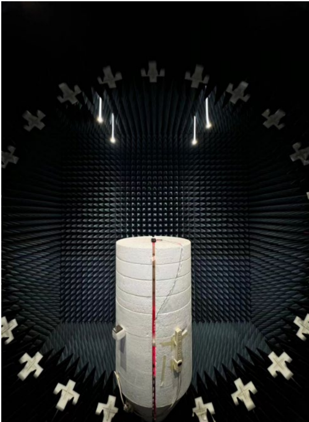
Antenna gain setup photo for PA2M36
