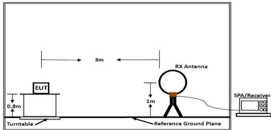
Below 30MHz
